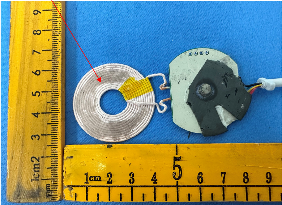
Coil Antenna
