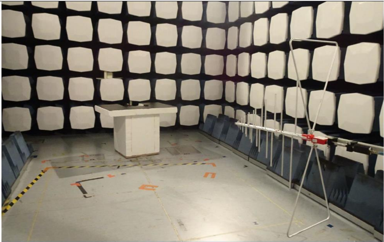
Picture 11, Radiated Spurious Emissions, common setup, TX and RX 30 - 1000 MHz
