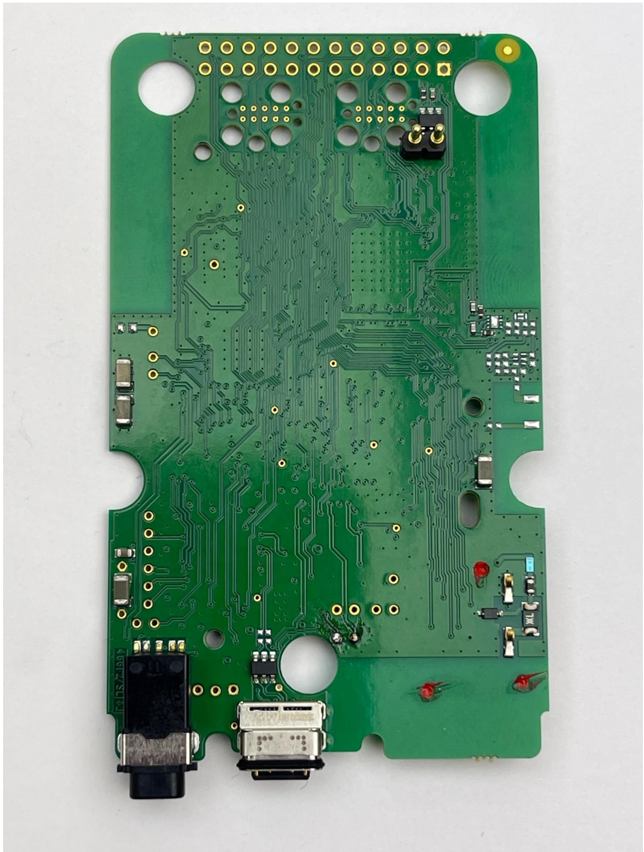
PCB Bottom:
