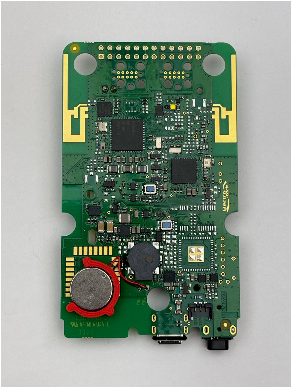
PCB top:
