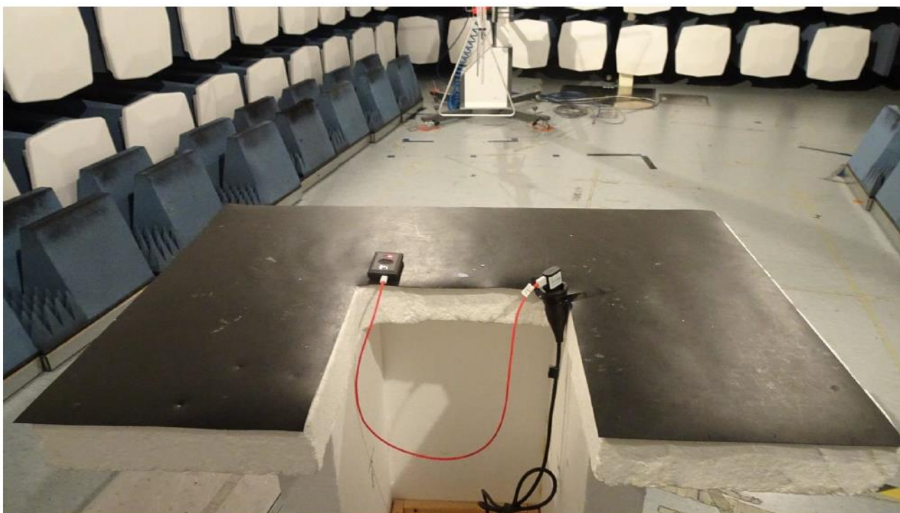
Picture 11 Radiated emission pictures, back view OM2
