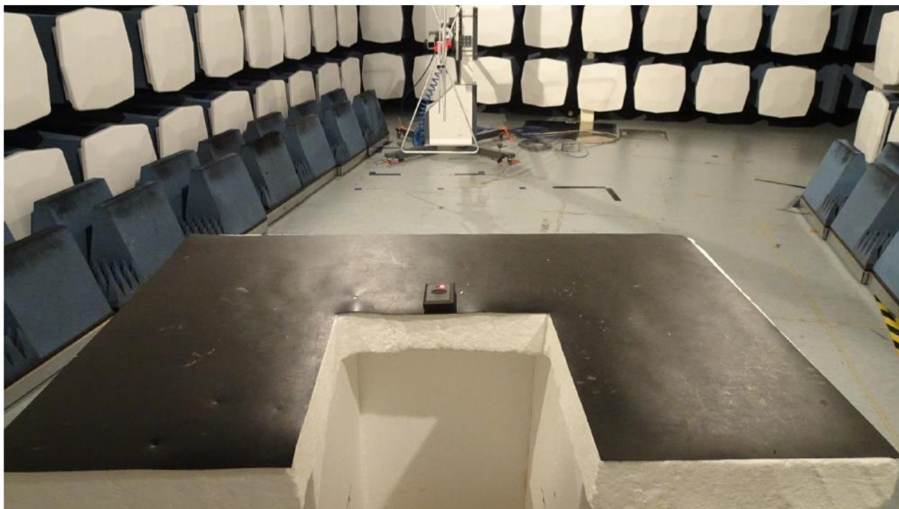
Picture 10 Radiated emission pictures, back view OM1
