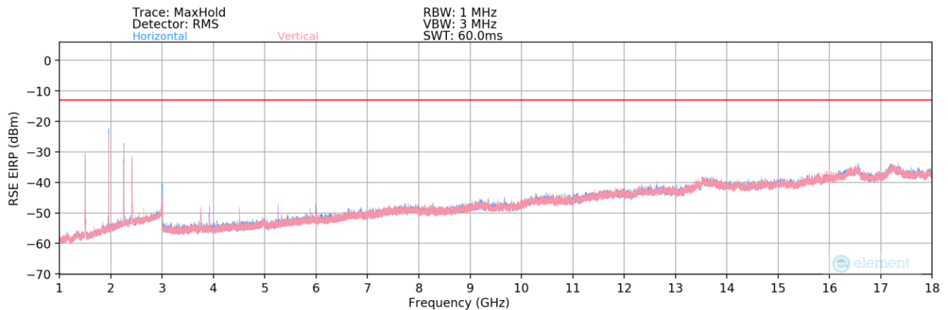
Plot 7-52. Radiated Spurious Plot – Above 1GHz
