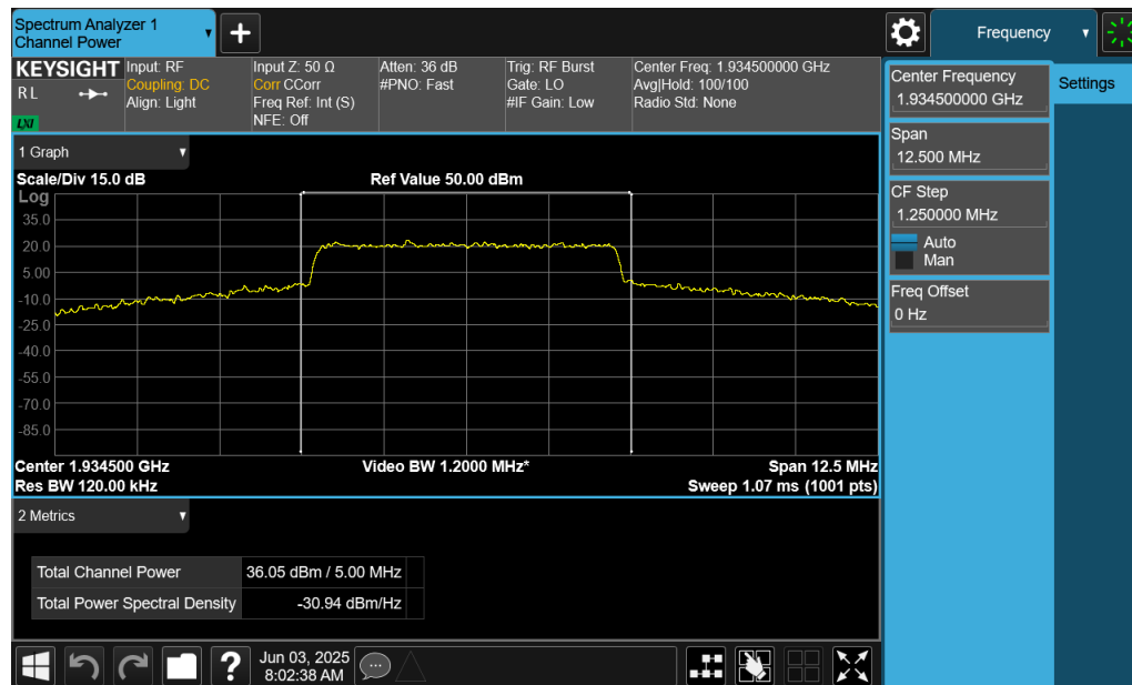
Plot 7-1. Conducted Power Output Data (LTE Band 25/2 – Low Channel)
