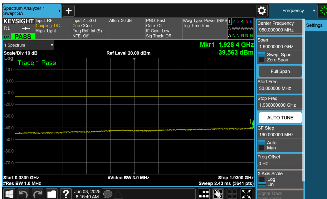
Plot 7-16. Conducted Spurious Plot (LTE Band 25/2 - 5MHz QPSK - Mid Channel)
