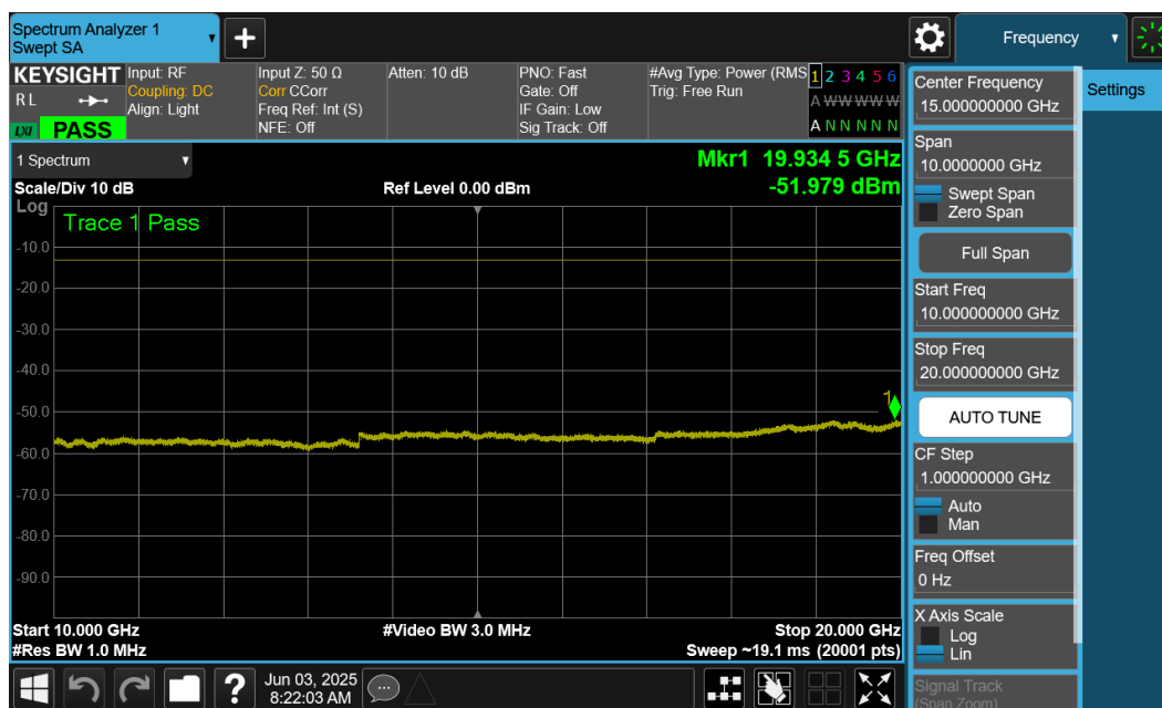
Plot 7-21. Conducted Spurious Plot (LTE Band 25/2 - 5MHz QPSK - High Channel)
