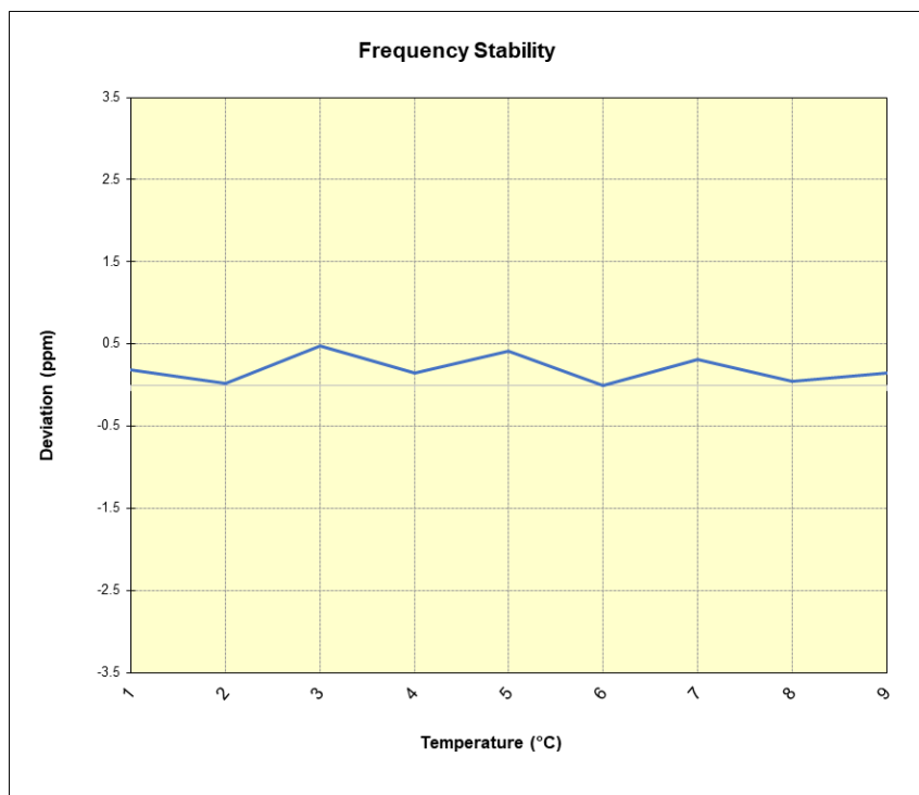
Plot 7-55. LTE Band 25/2 Frequency Stability Chart
