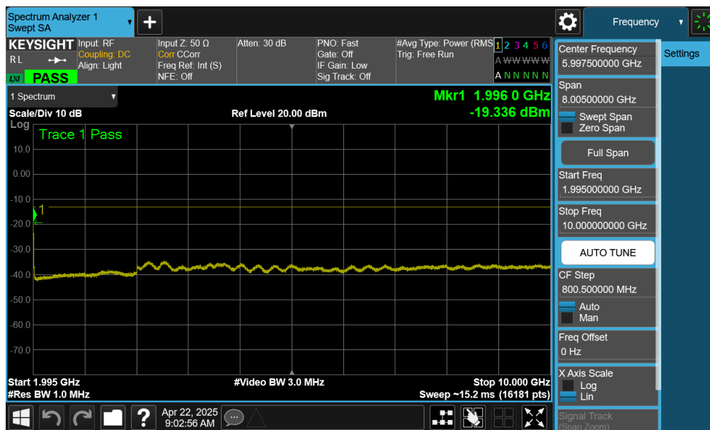
Plot 7-38. Conducted Spurious Plot (WCDMA – High Channel)
