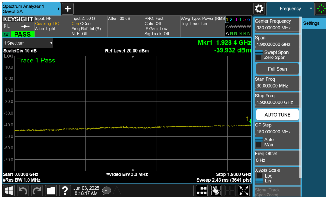
Plot 7-19. Conducted Spurious Plot (LTE Band 25/2 - 5MHz QPSK - High Channel)
