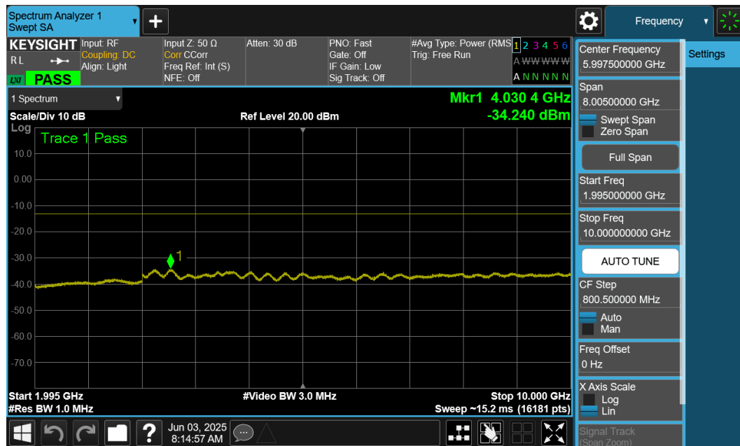
Plot 7-14. Conducted Spurious Plot (LTE Band 25/2 - 5MHz QPSK - Low Channel)
