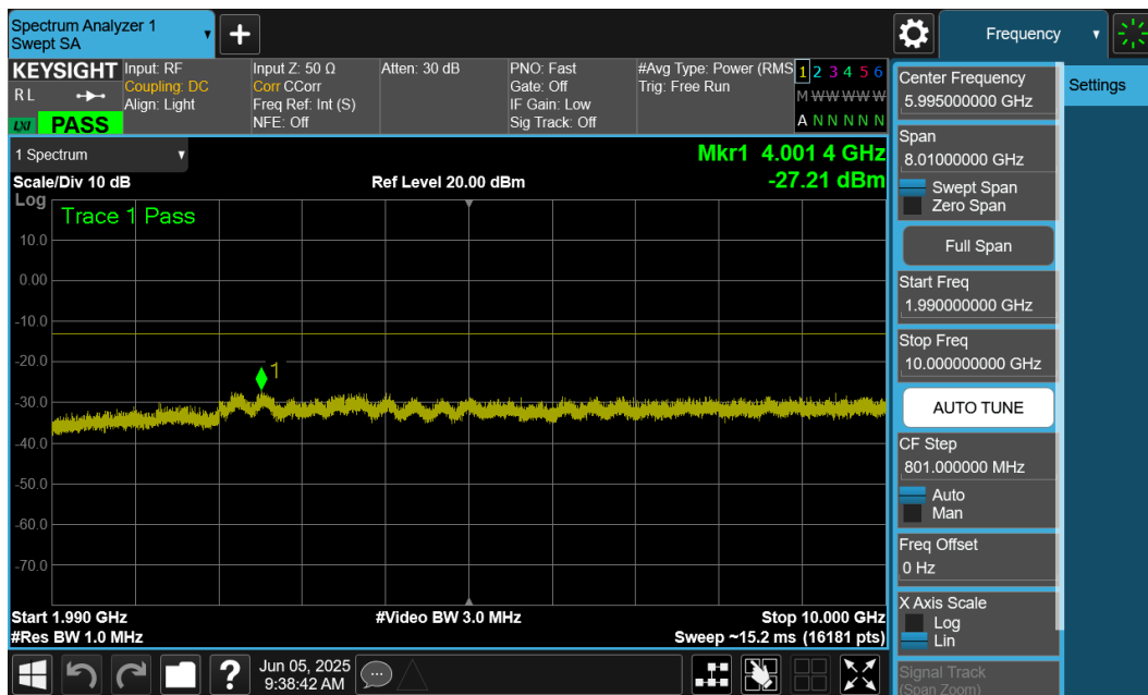
Plot 7-23. Conducted Spurious Plot (GSM – Low Channel)
