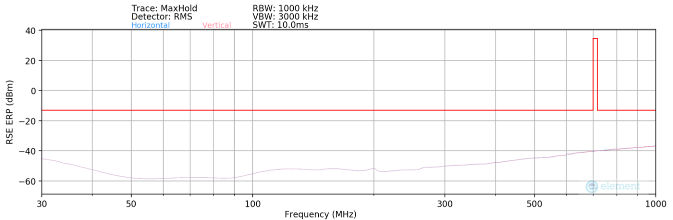
Plot 7-51. Radiated Spurious Plot – Below 1GHz
