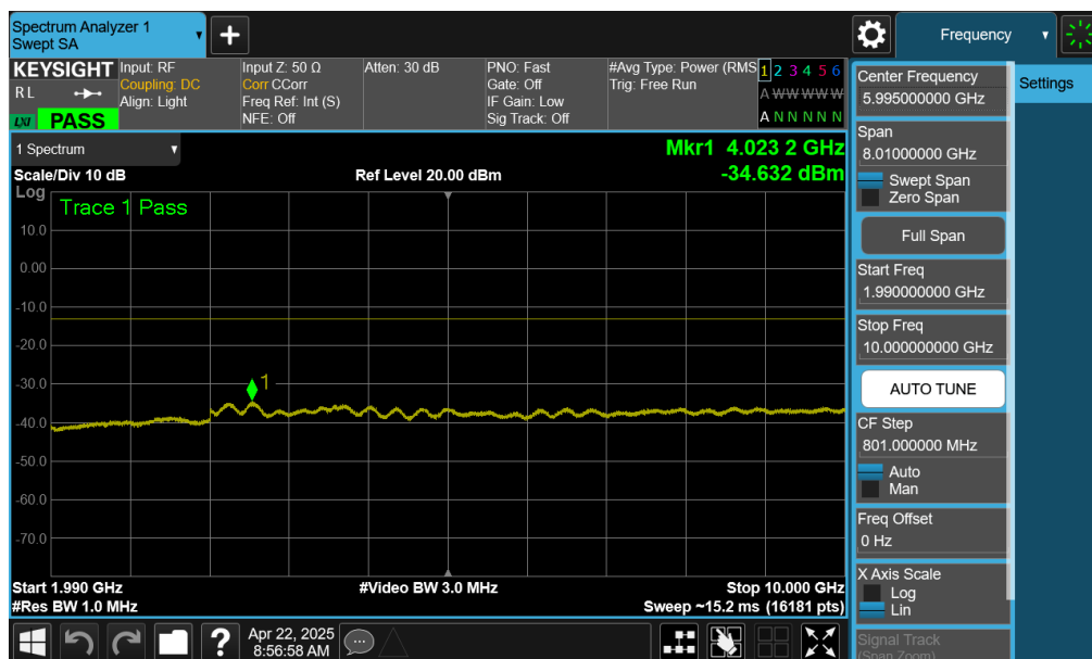
Plot 7-32. Conducted Spurious Plot (WCDMA – Low Channel)
