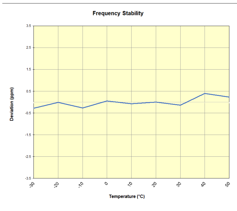
Plot 7-57. WCDMA PCS Frequency Stability Chart
