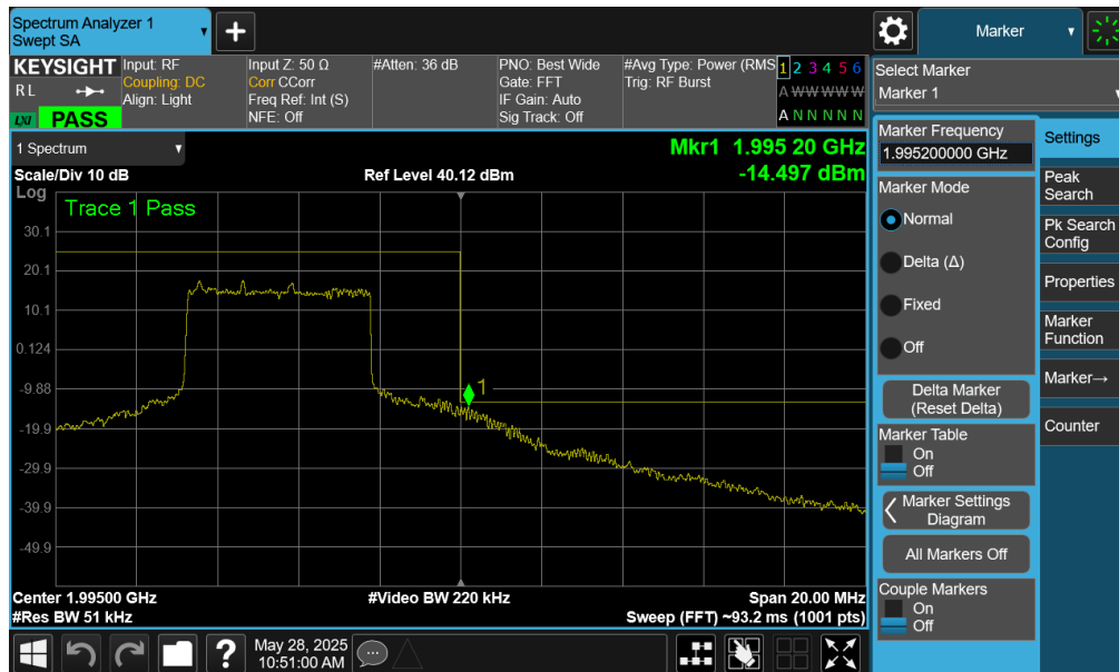
Plot 7-41. Upper Band Edge Plot (LTE Band 25/2 - 5MHz QPSK – Full RB)
