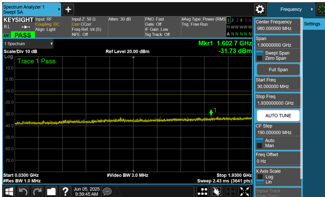
Plot 7-25. Conducted Spurious Plot (GSM – Mid Channel)
