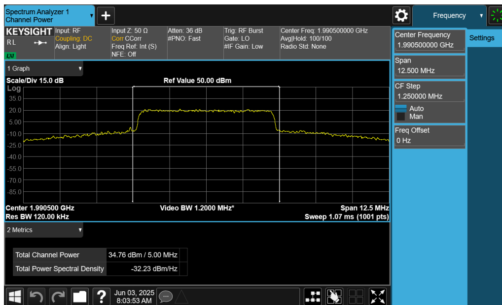
Plot 7-3. Conducted Power Output Data (LTE Band 25/2 – High Channel)
