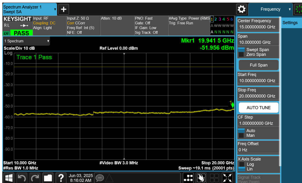
Plot 7-15. Conducted Spurious Plot (LTE Band 25/2 - 5MHz QPSK - Low Channel)
