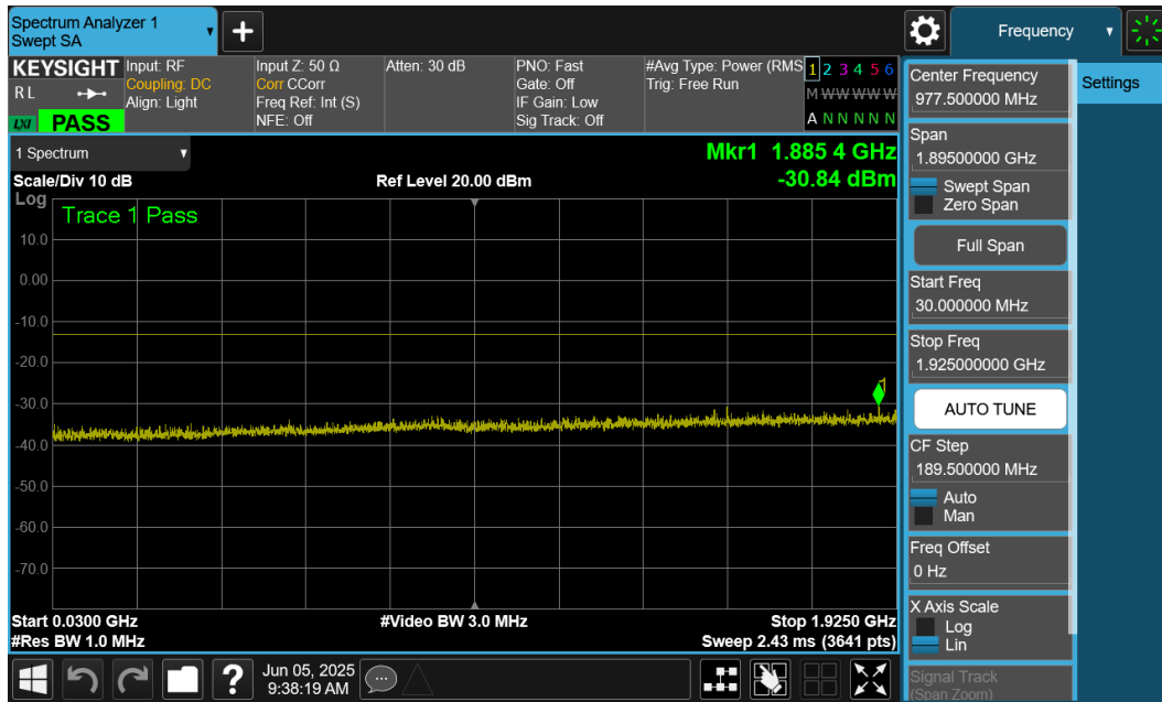
Plot 7-22. Conducted Spurious Plot (GSM – Low Channel)
