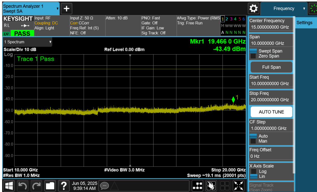
Plot 7-24. Conducted Spurious Plot (GSM – Low Channel)
