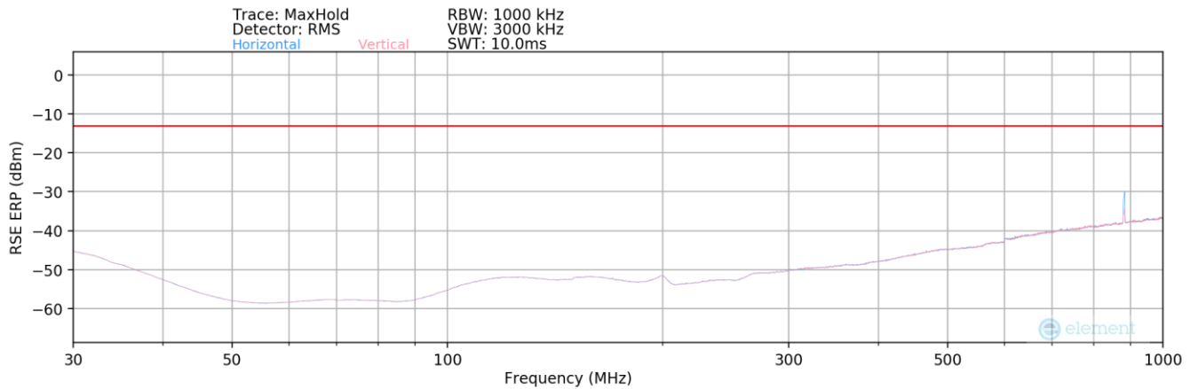
Plot 7-49. Radiated Spurious Plot - Below 1GHz
