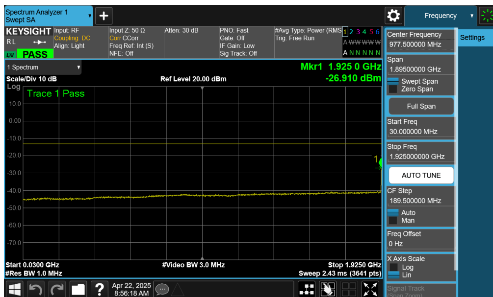
Plot 7-31. Conducted Spurious Plot (WCDMA – Low Channel)
