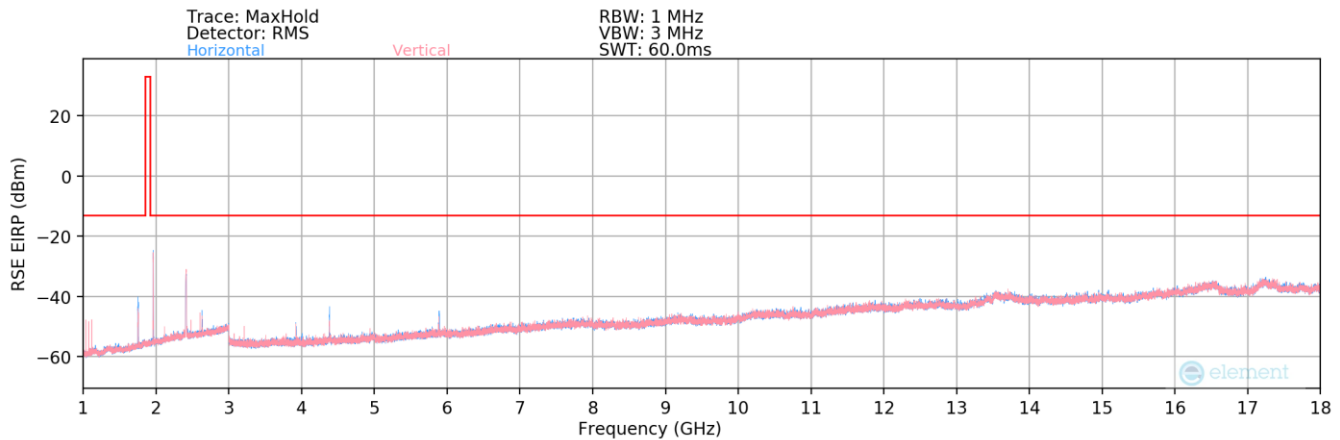
Plot 7-50. Radiated Spurious Plot - Above 1GHz
