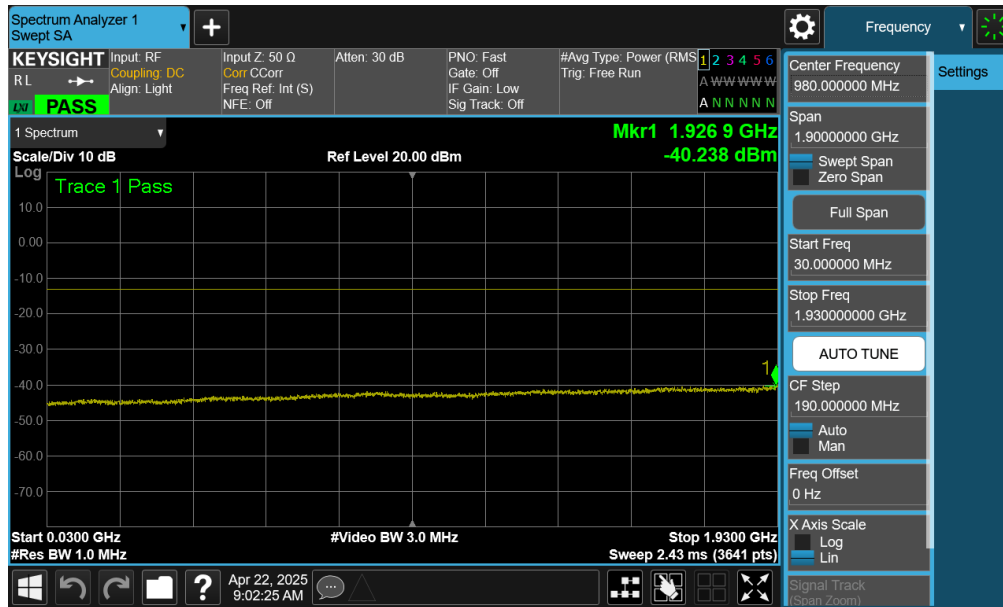
Plot 7-37. Conducted Spurious Plot (WCDMA – High Channel)
