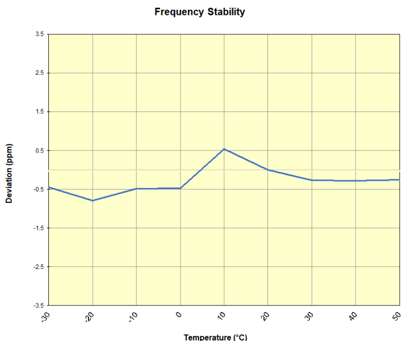
Plot 7-56. GSM/GPRS PCS Frequency Stability Chart
