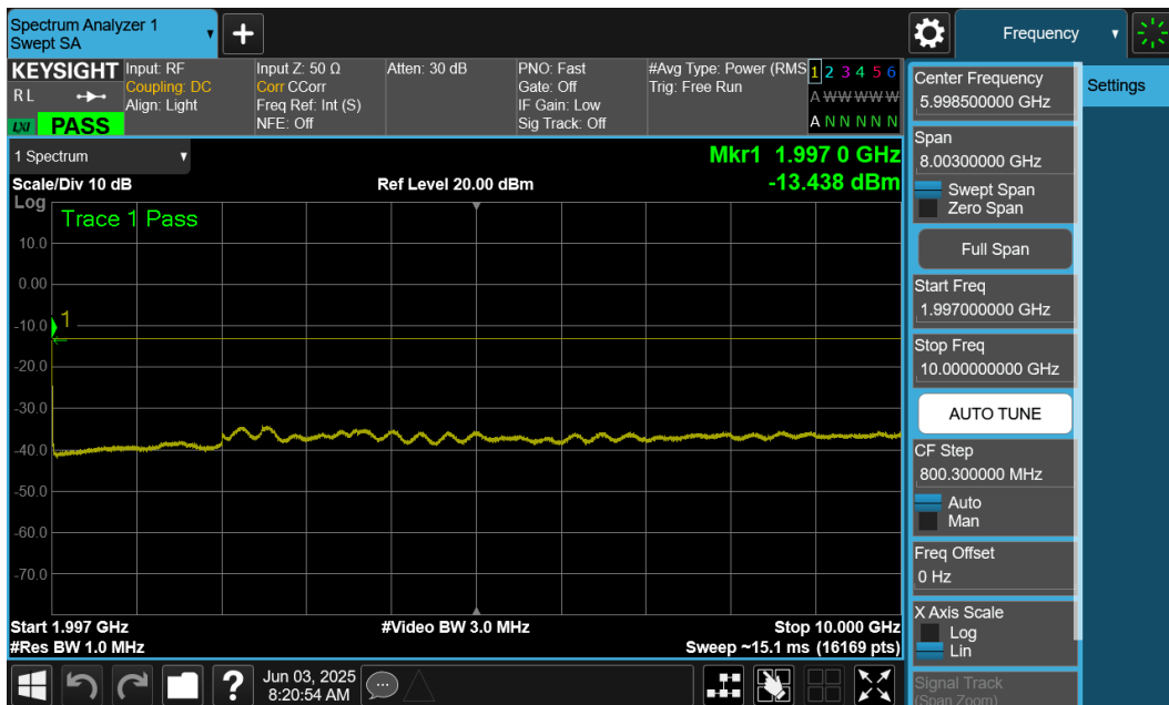
Plot 7-20. Conducted Spurious Plot (LTE Band 25/2 - 5MHz QPSK - High Channel)
