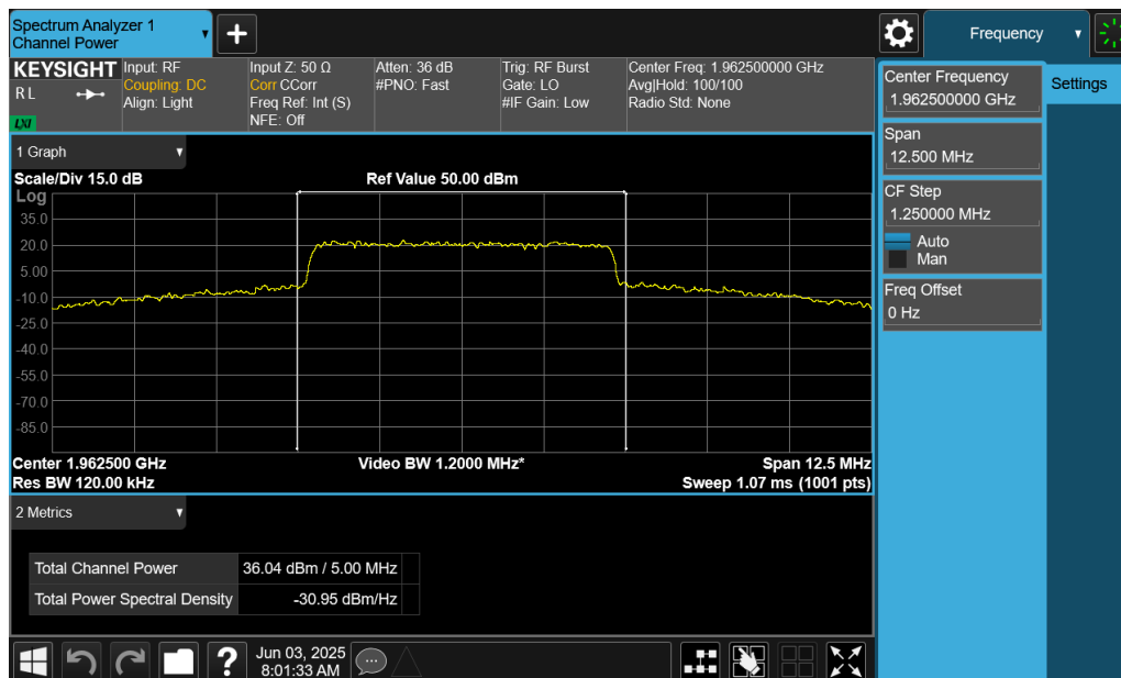
Plot 7-2. Conducted Power Output Data (LTE Band 25/2 – Mid Channel)
