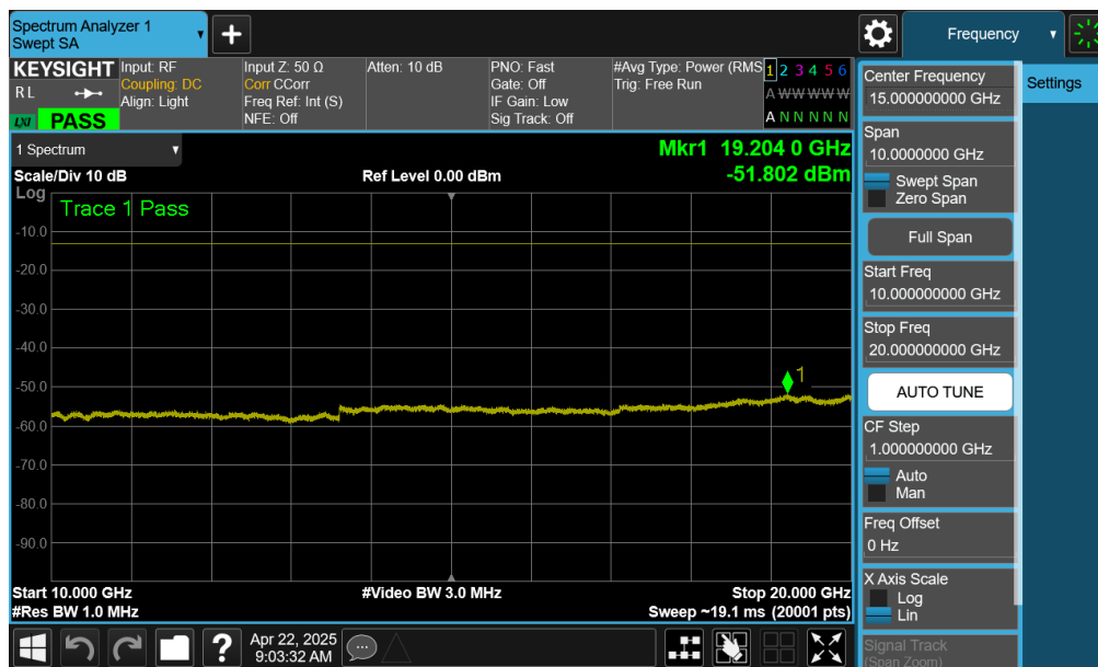
Plot 7-39. Conducted Spurious Plot (WCDMA – High Channel)
