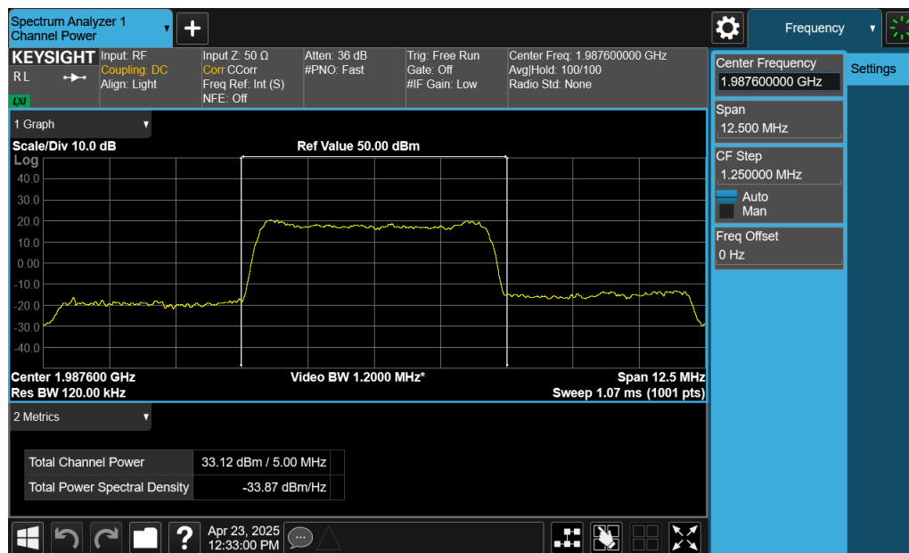
Plot 7-6. Conducted Power Output Data (WCDMA 1900 – High Channel)
