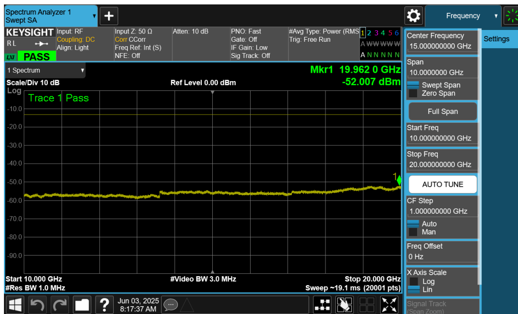
Plot 7-18. Conducted Spurious Plot (LTE Band 25/2 - 5MHz QPSK - Mid Channel)
