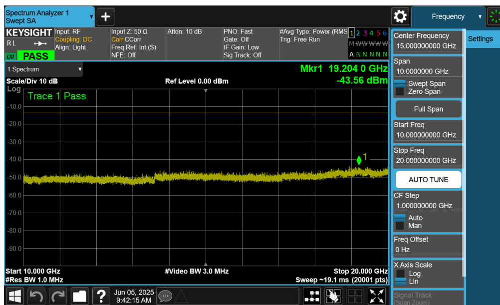
Plot 7-30. Conducted Spurious Plot (GSM – High Channel)
