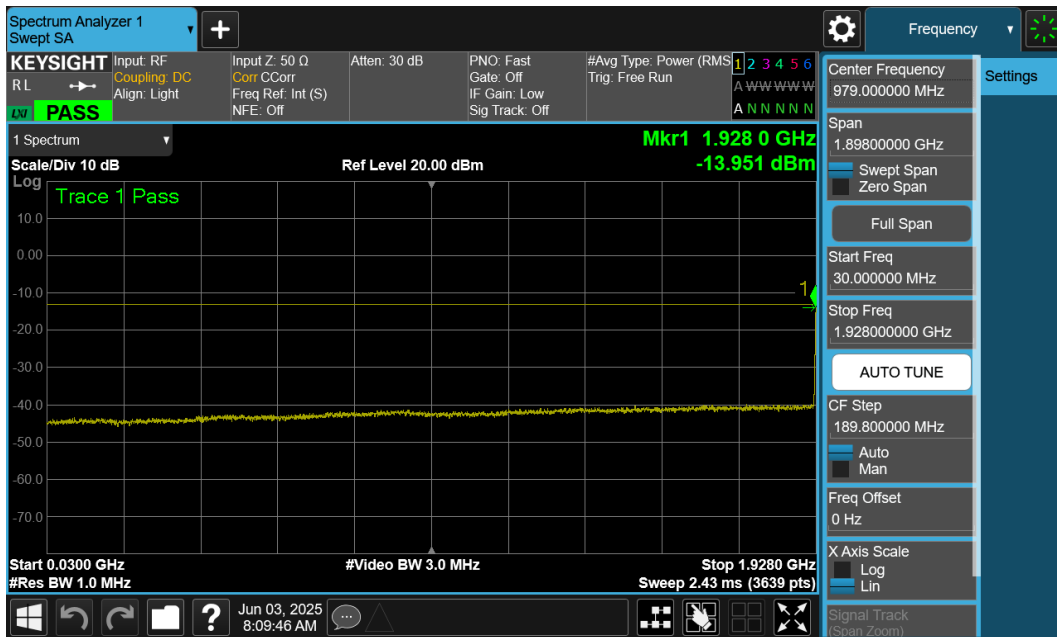
Plot 7-13. Conducted Spurious Plot (LTE Band 25/2 - 5MHz QPSK - Low Channel)
