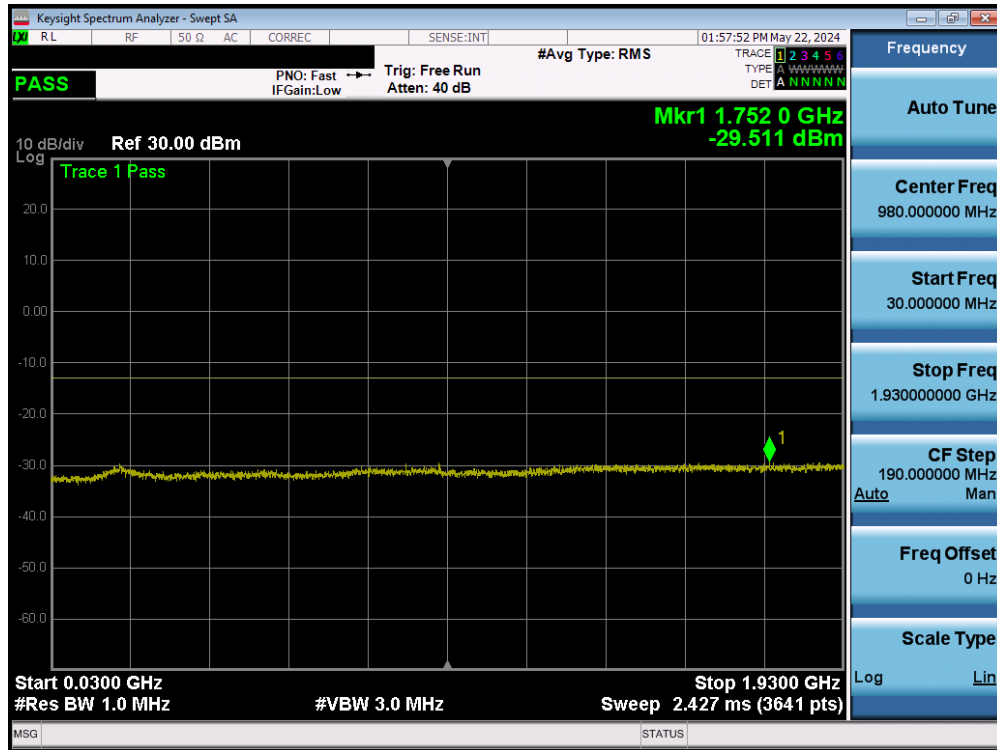
Plot 7-19. Conducted Spurious Plot (LTE Band 25/2 – High Channel)
