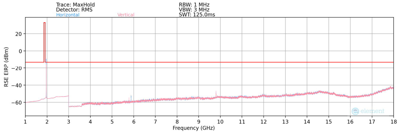
Plot 7-54. Radiated Spurious Plot (WCDMA 1900) - 1-18GHz
