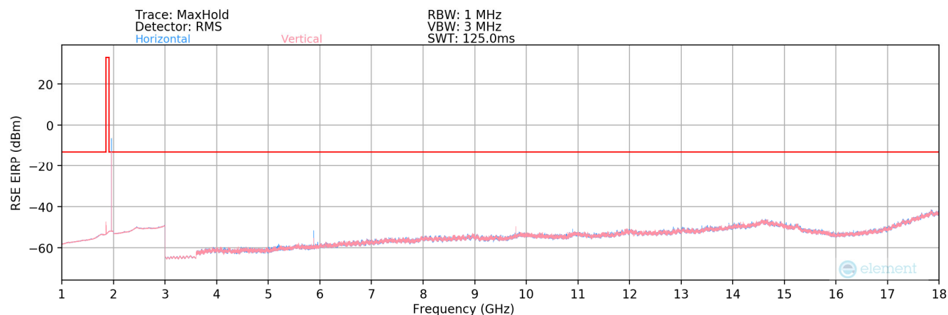
Plot 7-56. Radiated Spurious Plot (GSM 1900) - 1-18GHz
