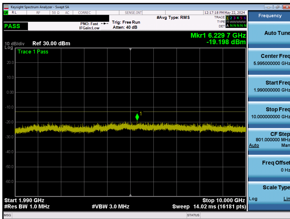
Plot 7-32. Conducted Spurious Plot (GSM PCS – Low Channel)
