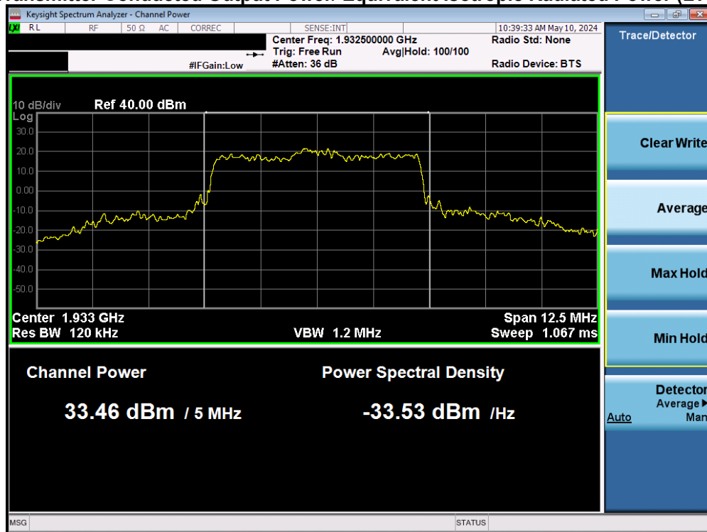
Plot 7-1. Conducted Power Output Data (LTE Band 25/2 – Low Channel)
