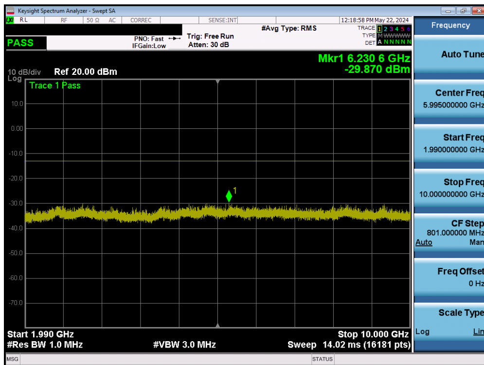
Plot 7-35. Conducted Spurious Plot (GSM PCS – Mid Channel)
