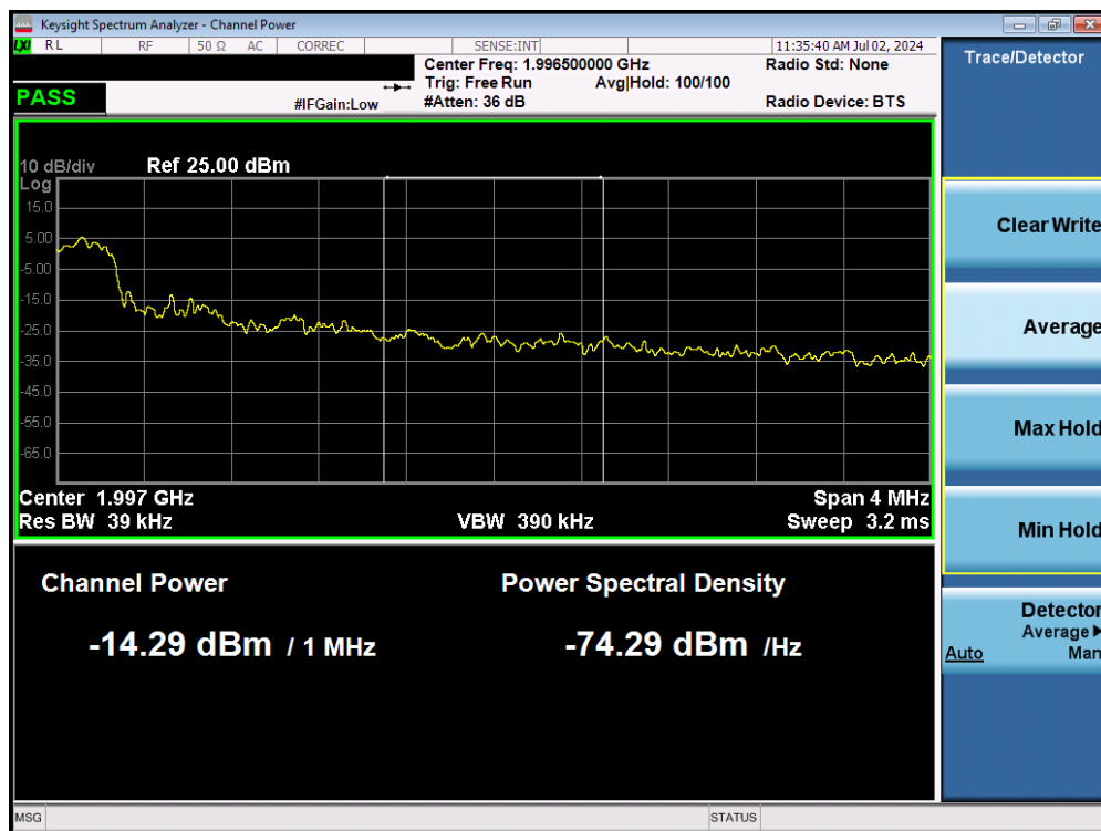
Plot 7-42. Upper Extended Band Edge Plot (LTE Band 25 – High Channel)
