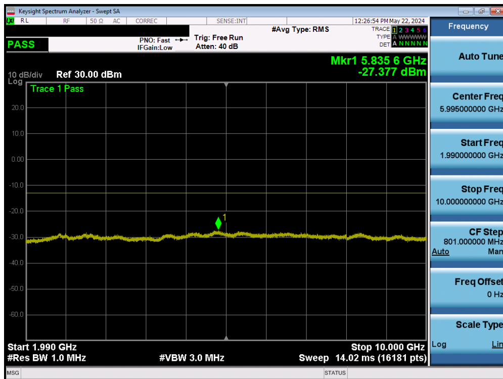
Plot 7-26. Conducted Spurious Plot (WCDMA PCS - Mid Channel)
