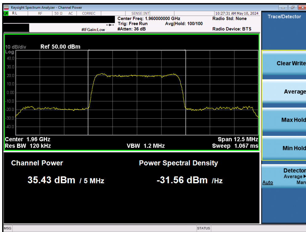
Plot 7-5. Conducted Power Output Data (WCDMA 1900 – Mid Channel)
