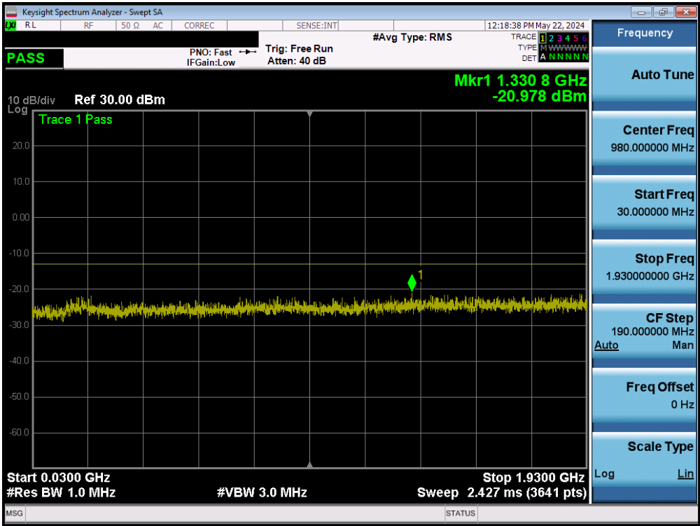
Plot 7-34. Conducted Spurious Plot (GSM PCS – Mid Channel)
