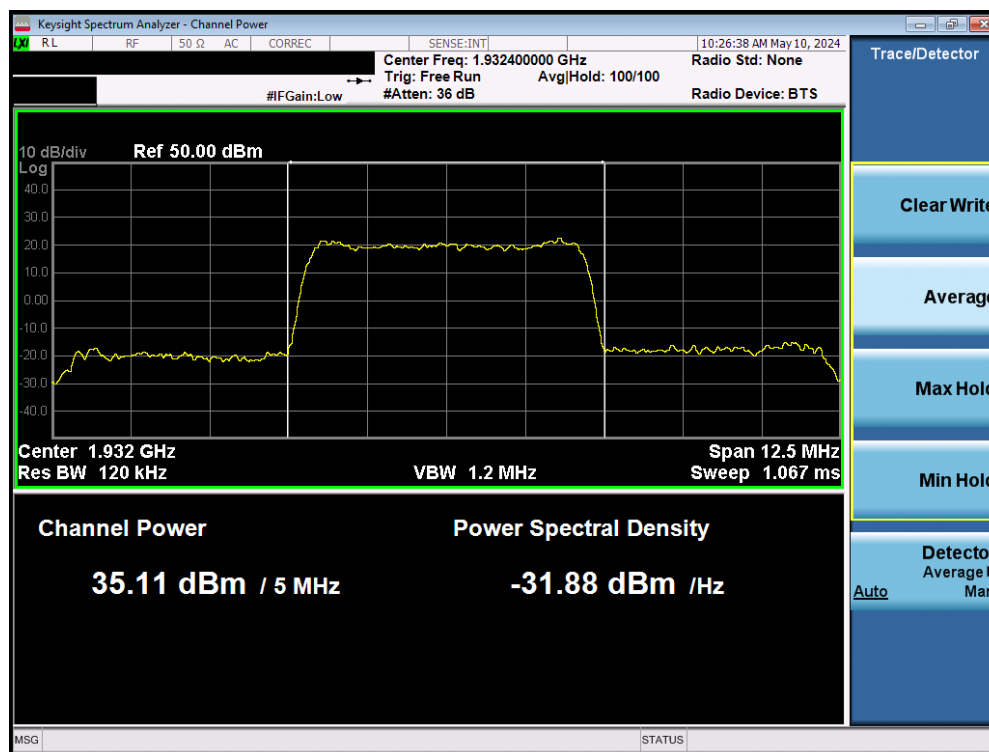
Plot 7-4. Conducted Power Output Data (WCDMA 1900 – Low Channel)
