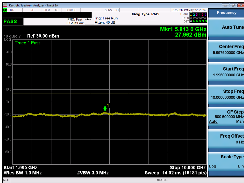
Plot 7-17. Conducted Spurious Plot (LTE Band 25/2 – Mid Channel)
