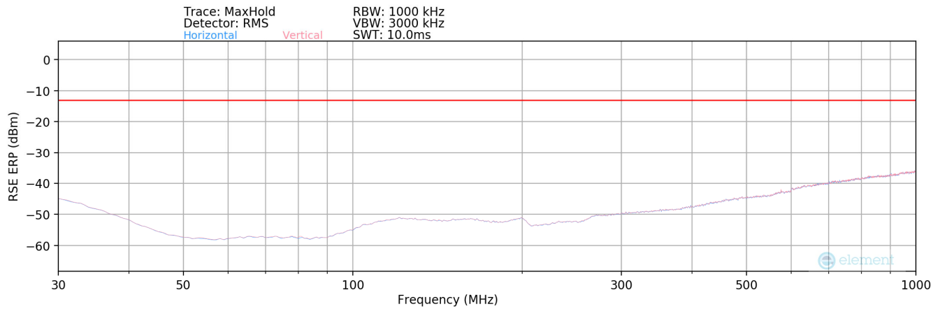
Plot 7-53. Radiated Spurious Plot (WCDMA 1900) - Below 1GHz
