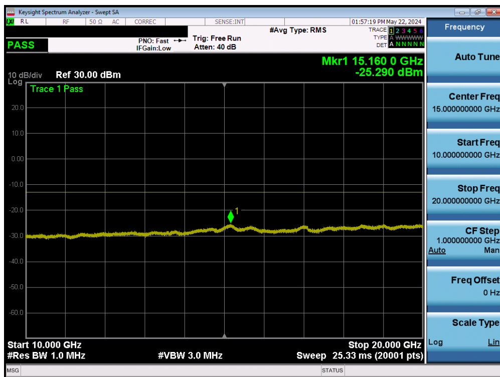
Plot 7-18. Conducted Spurious Plot (LTE Band 25/2 – Mid Channel)
