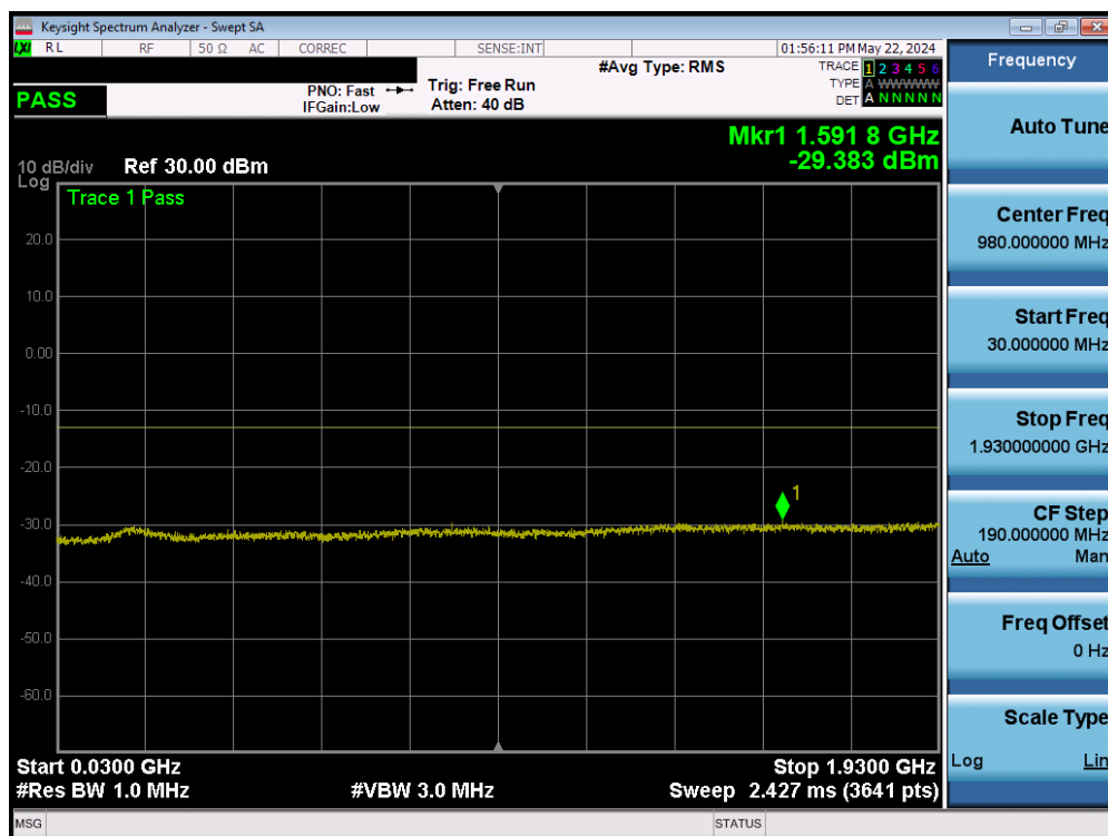
Plot 7-16. Conducted Spurious Plot (LTE Band 25/2 – Mid Channel)
