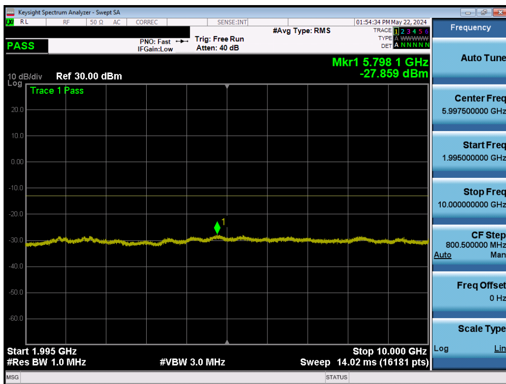
Plot 7-14. Conducted Spurious Plot (LTE Band 25/2 – Low Channel)
