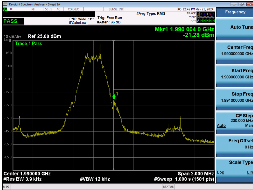
Plot 7-47. Upper Band Edge Plot (GSM PCS – High Channel)
