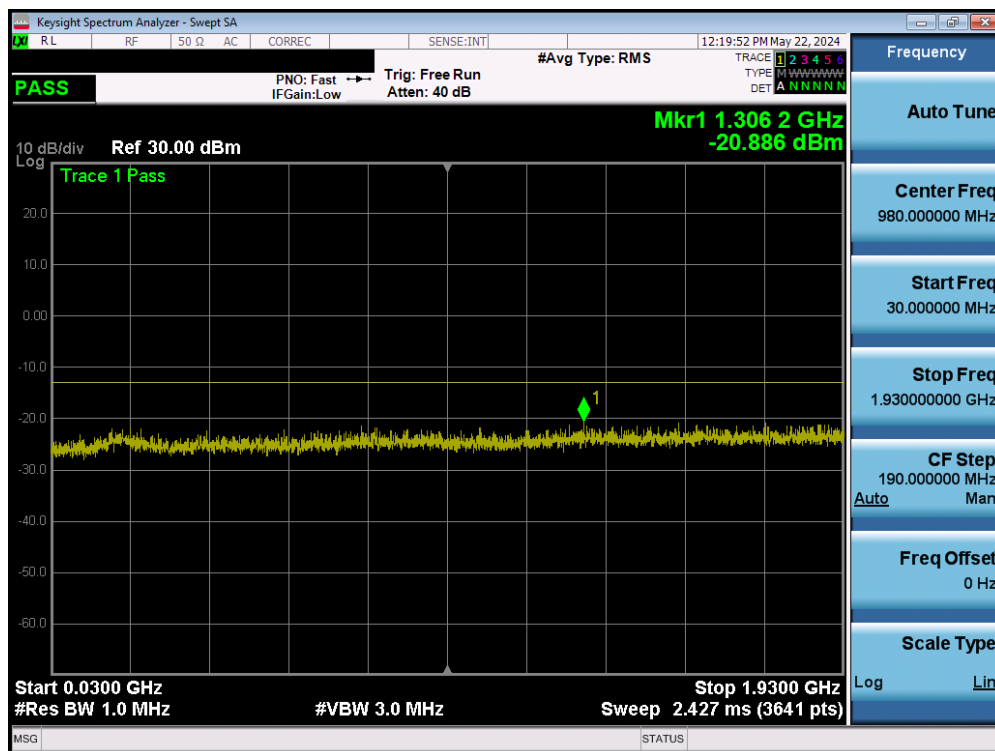
Plot 7-37. Conducted Spurious Plot (GSM PCS – High Channel)
