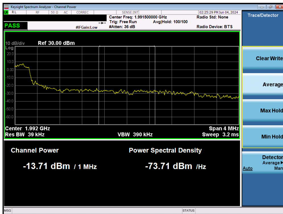
Plot 7-43. Upper Extended Band Edge Plot (LTE Band 2 – High Channel)
