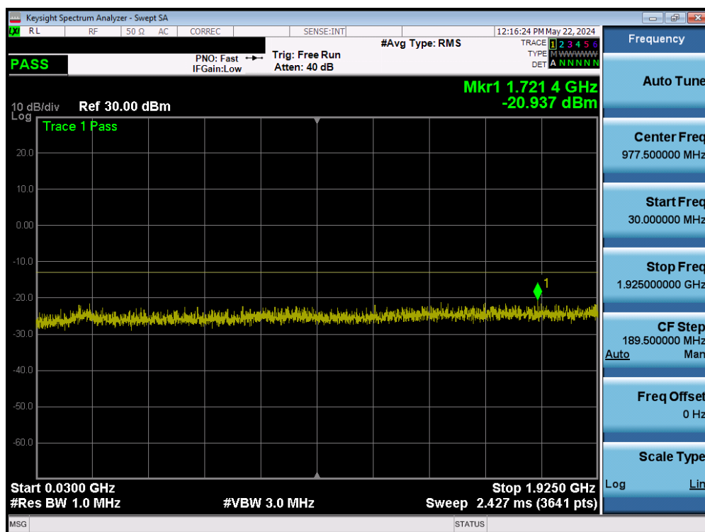
Plot 7-31. Conducted Spurious Plot (GSM PCS – Low Channel)
