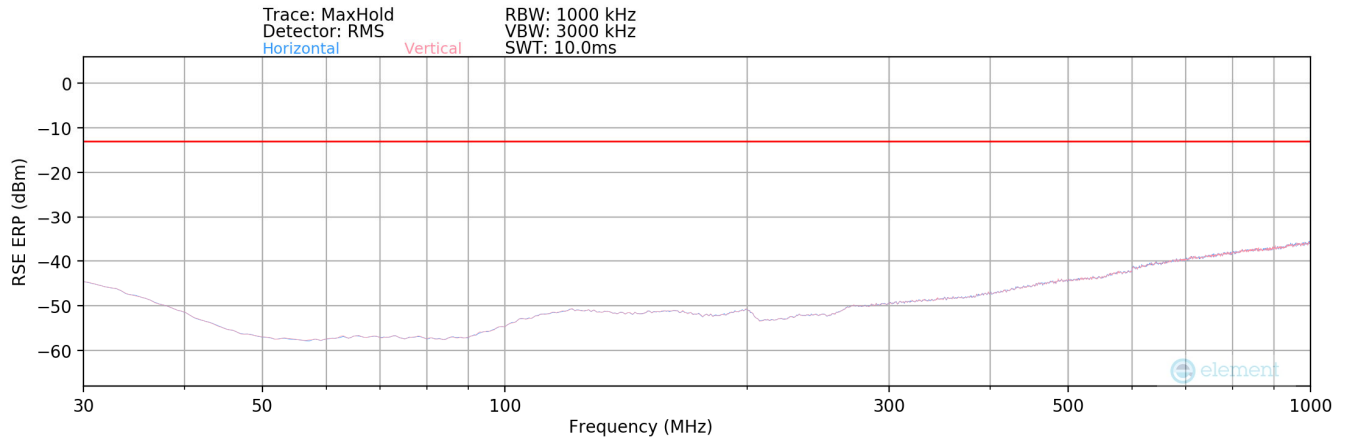
Plot 7-51. Radiated Spurious Plot (LTE Band 25) - Below 1GHz
