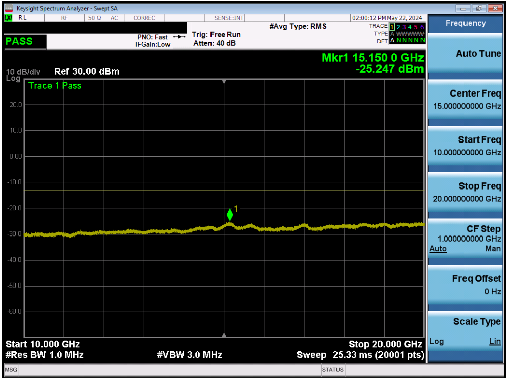
Plot 7-21. Conducted Spurious Plot (LTE Band 25/2 – High Channel)
