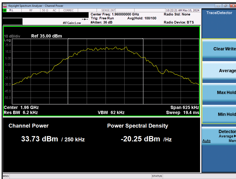
Plot 7-8. Conducted Power Output Data (GSM 1900 – Mid Channel)
