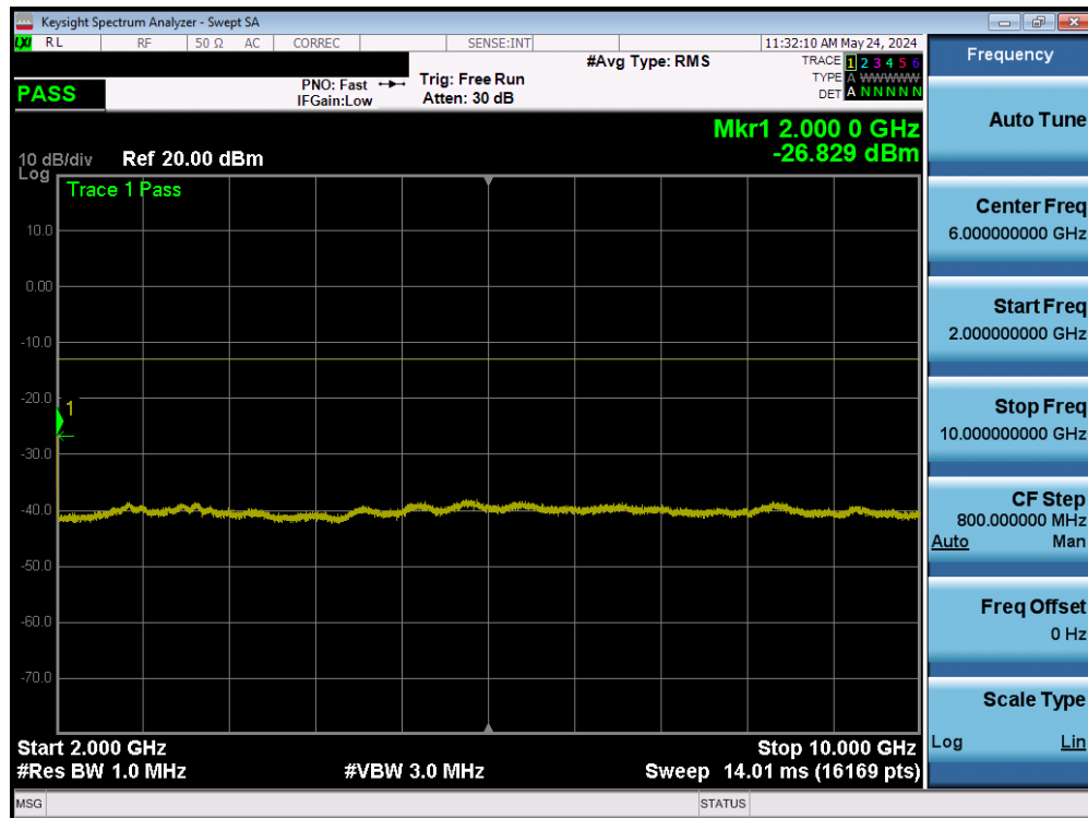
Plot 7-20. Conducted Spurious Plot (LTE Band 25/2 – High Channel)
