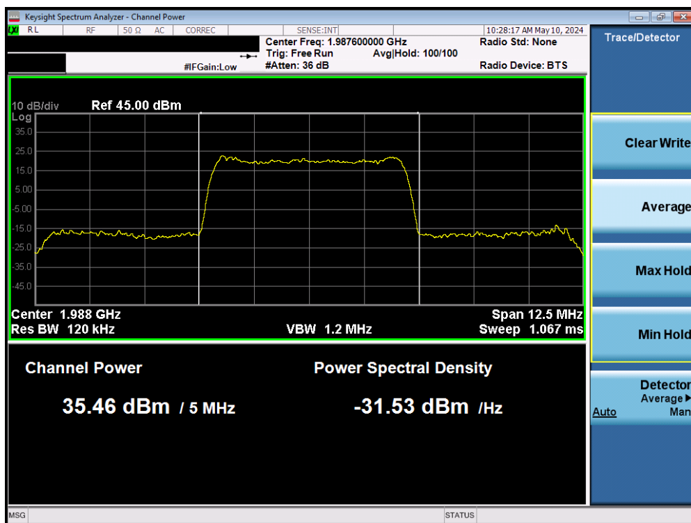
Plot 7-6. Conducted Power Output Data (WCDMA 1900 – High Channel)
