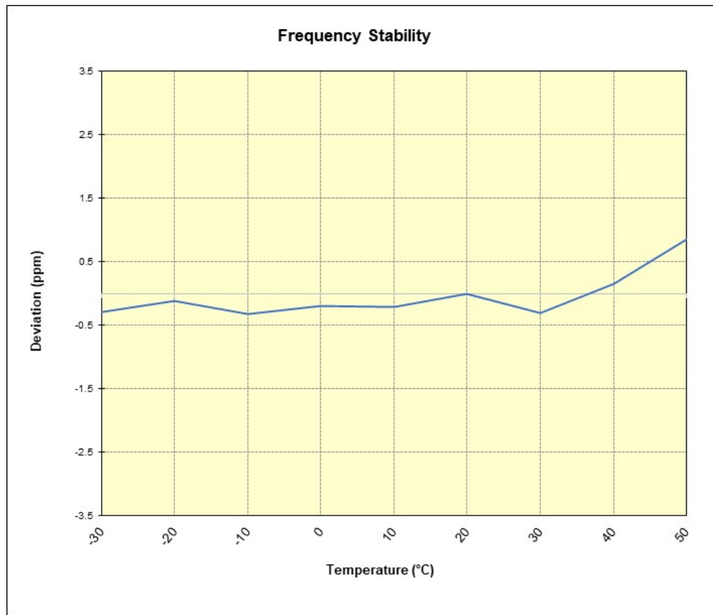
Plot 7-59. GSM 1900 Frequency Stability Chart
