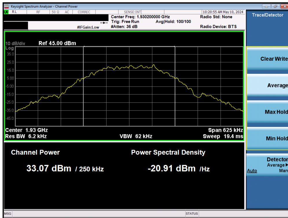
Plot 7-7. Conducted Power Output Data (GSM 1900 – Low Channel)
