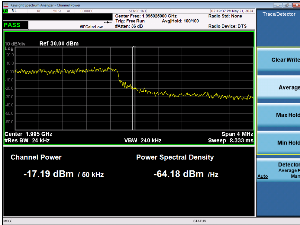
Plot 7-41. Upper Band Edge Plot (LTE Band 25 – High Channel)
