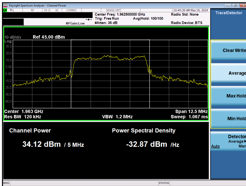
Plot 7-2. Conducted Power Output Data (LTE Band 25/2 – Mid Channel)
