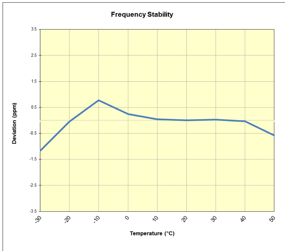
Plot 7-58. WCDMA 1900 Frequency Stability Chart
