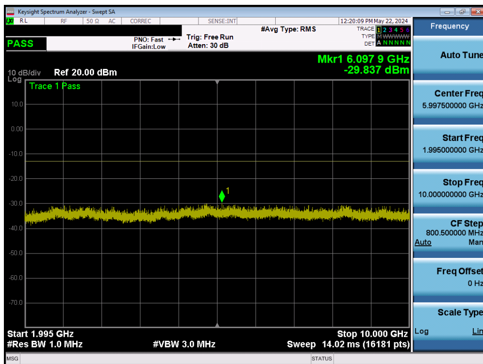
Plot 7-38. Conducted Spurious Plot (GSM PCS – High Channel)
