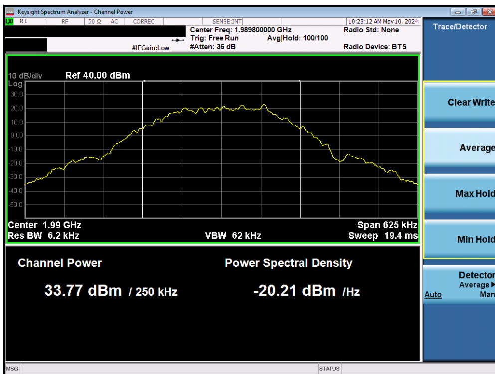
Plot 7-9. Conducted Power Output Data (GSM 1900 – High Channel)
