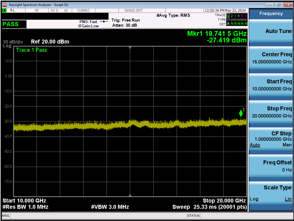
Plot 7-39. Conducted Spurious Plot (GSM PCS – High Channel)
