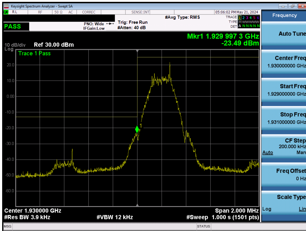
Plot 7-46. Lower Band Edge Plot (GSM PCS – Low Channel)
