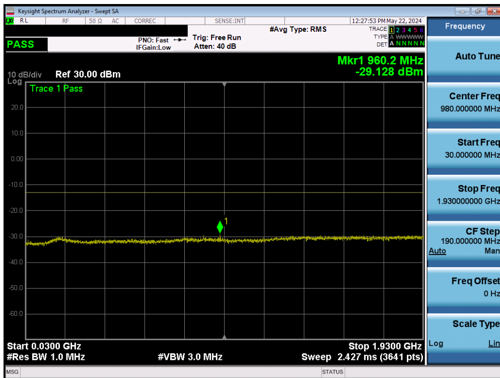
Plot 7-28. Conducted Spurious Plot (WCDMA PCS – High Channel)
