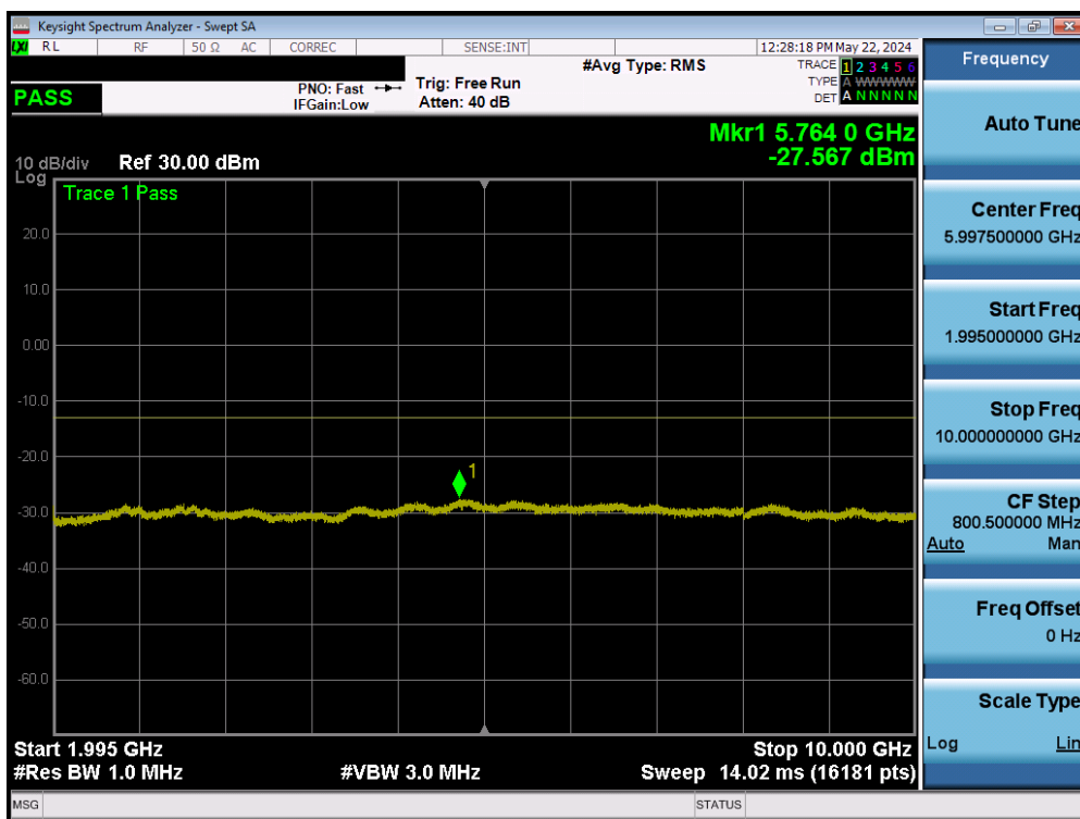
Plot 7-29. Conducted Spurious Plot (WCDMA PCS – High Channel)
