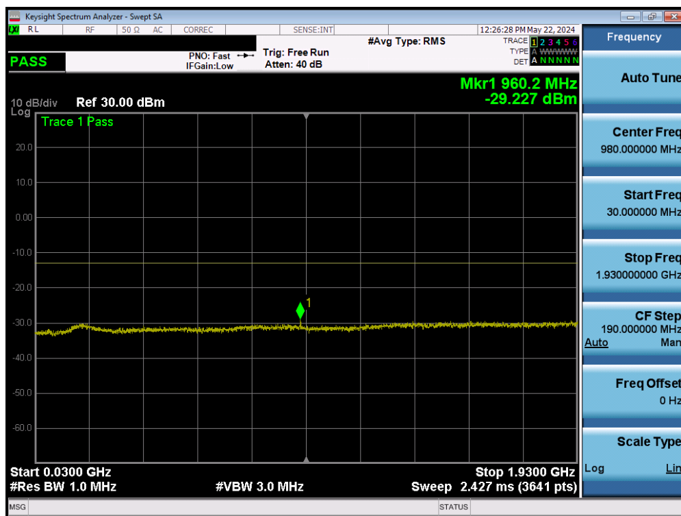
Plot 7-25. Conducted Spurious Plot (WCDMA PCS – Mid Channel)
