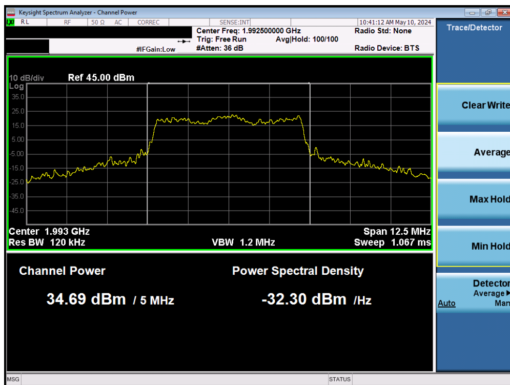
Plot 7-3. Conducted Power Output Data (LTE Band 25/2 – High Channel)
