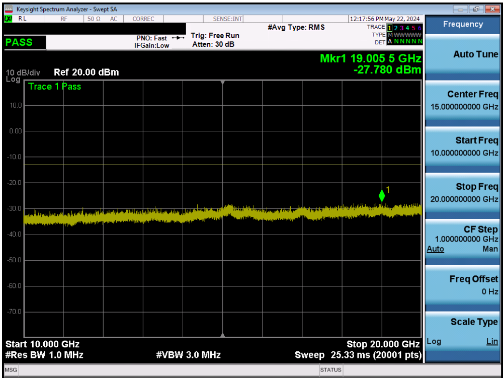
Plot 7-33. Conducted Spurious Plot (GSM PCS – Low Channel)
