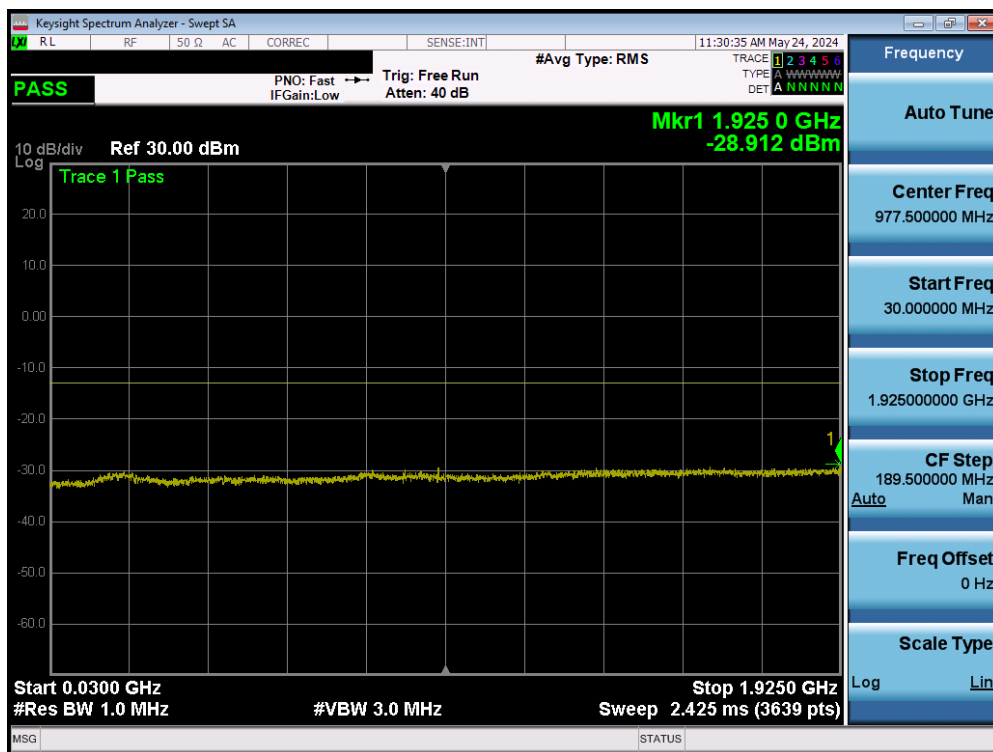
Plot 7-13. Conducted Spurious Plot (LTE Band 25/2 – Low Channel)
