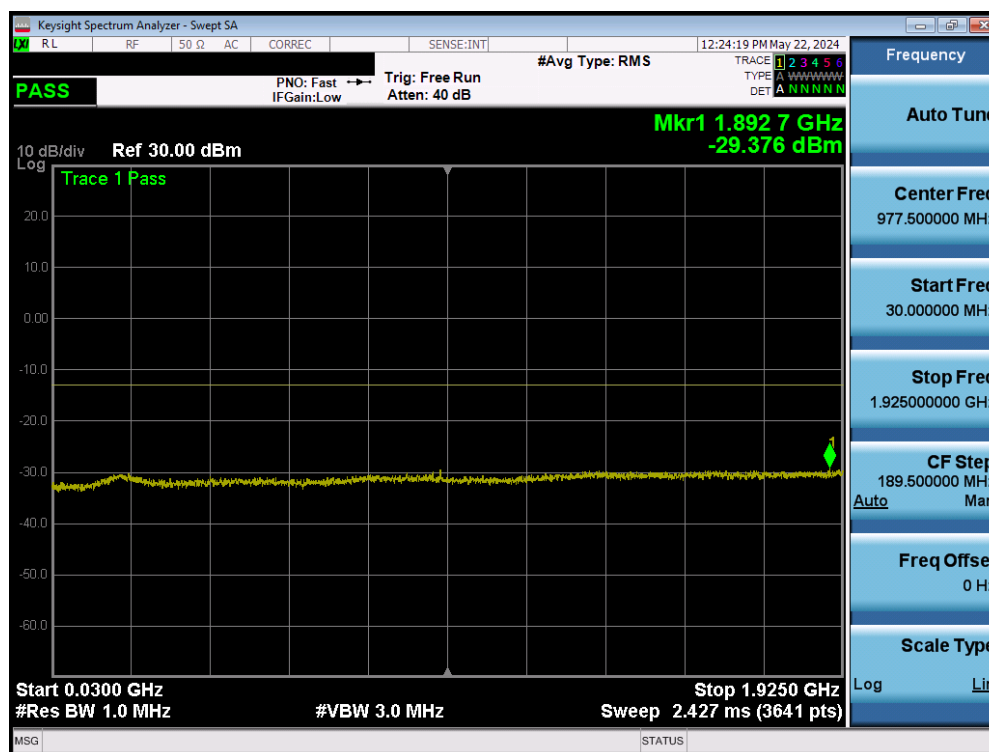
Plot 7-22. Conducted Spurious Plot (WCDMA PCS – Low Channel)
