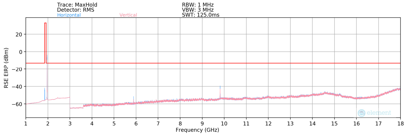
Plot 7-52. Radiated Spurious Plot (LTE Band 25) - 1-18GHz
