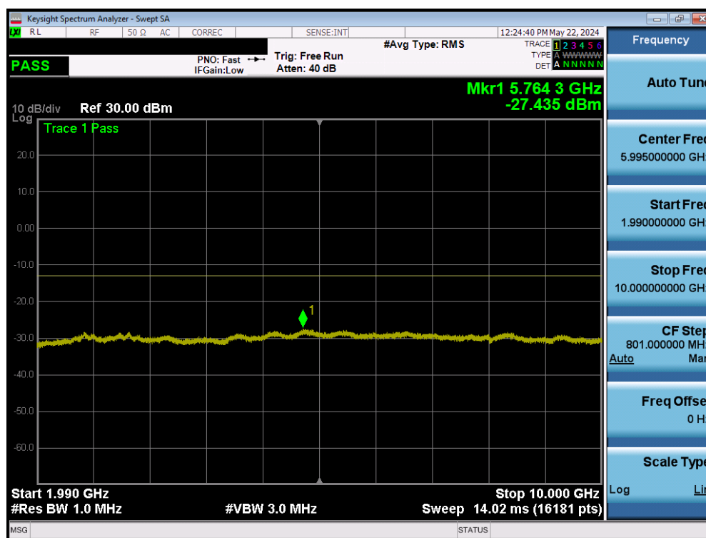
Plot 7-23. Conducted Spurious Plot (WCDMA PCS – Low Channel)
