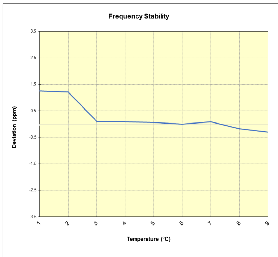
Plot 7-57. LTE Band 25 Frequency Stability Chart
