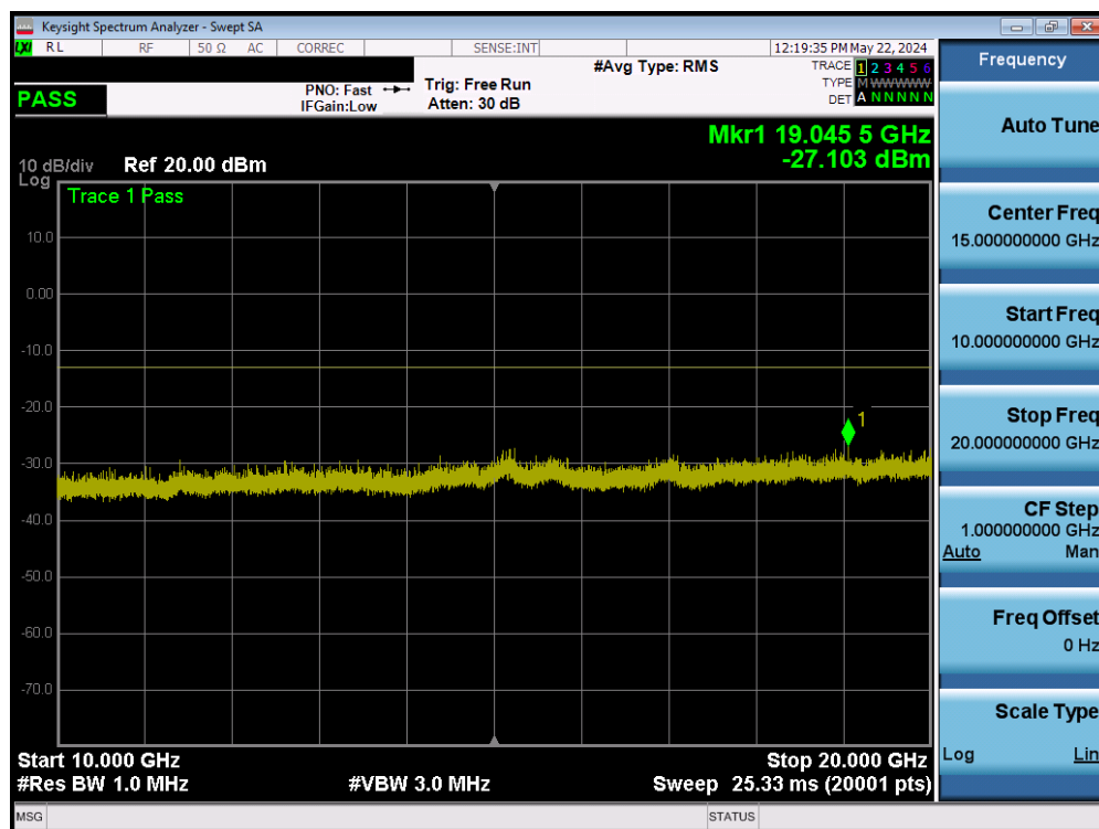
Plot 7-36. Conducted Spurious Plot (GSM PCS – Mid Channel)
