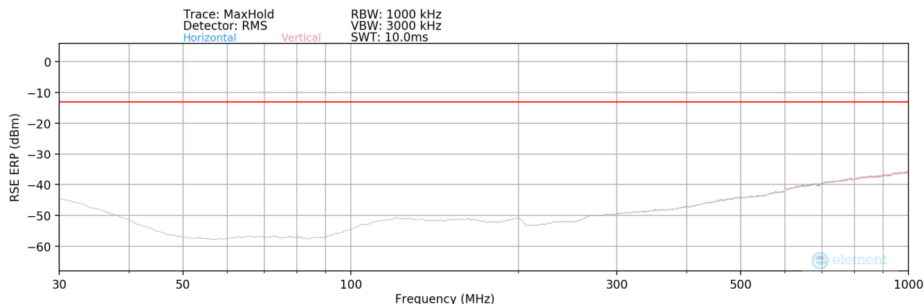
Plot 7-55. Radiated Spurious Plot (GSM 1900) - Below 1GHz
