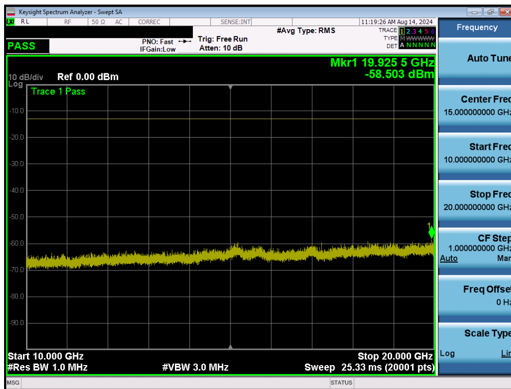
Plot 7-17. Conducted Spurious Plot (GSM Ch. 810)
