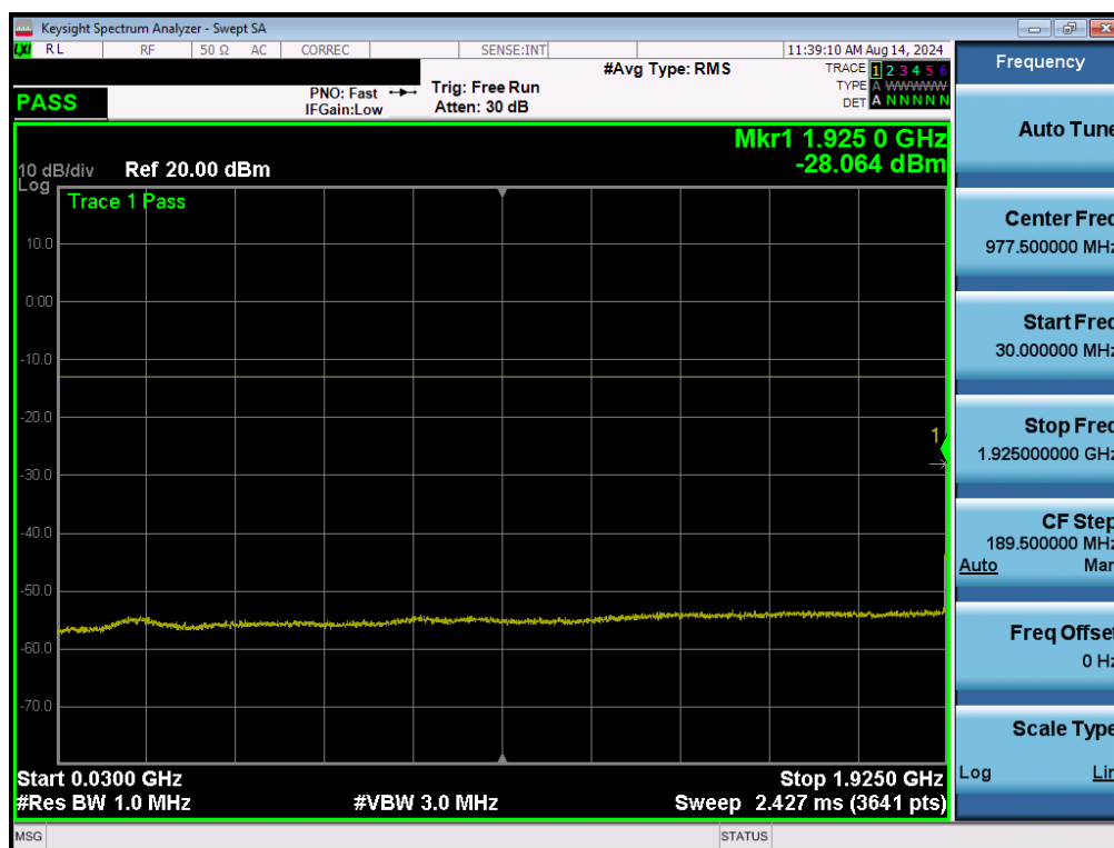
Plot 7-18. Conducted Spurious Plot (UMTS Ch. 9662)
