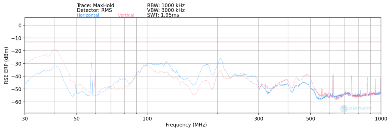
Plot 7-38. Radiated Spurious Plot (UMTS PCS) – Below 1GHz
