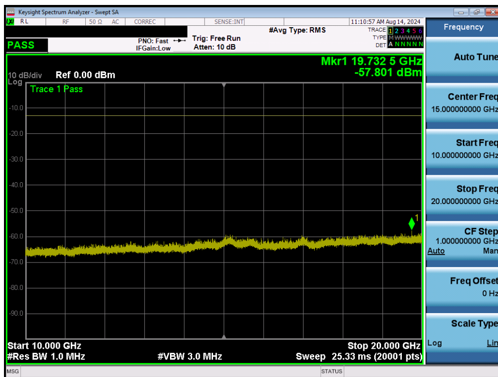
Plot 7-11. Conducted Spurious Plot (GSM Ch. 512)
