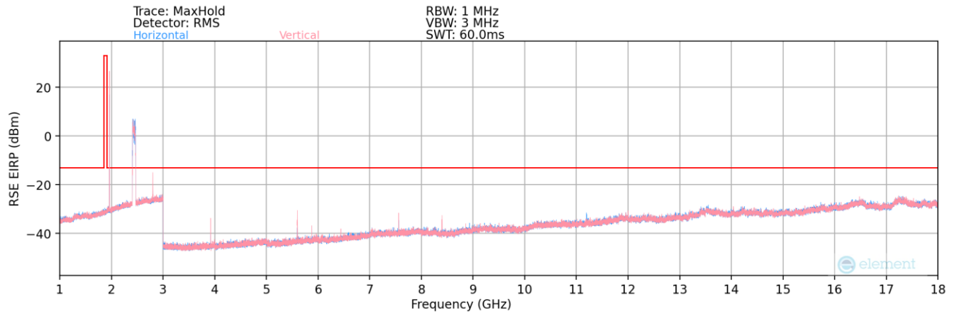
Plot 7-35. Radiated Spurious Plot (GSM PCS) – Above 1GHz
