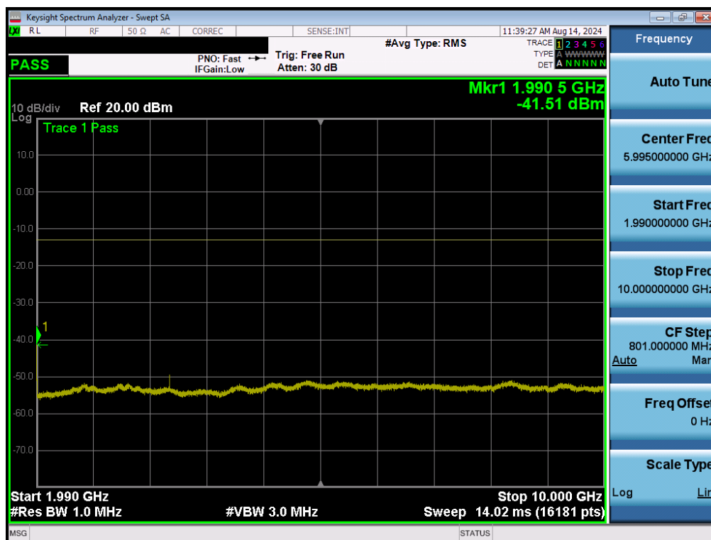
Plot 7-19. Conducted Spurious Plot (UMTS Ch. 9662)
