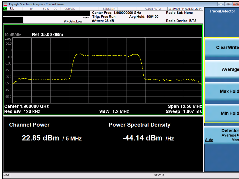
Plot 7-2. Conducted Power Output Data (UMTS 1900 – Mid Channel)
