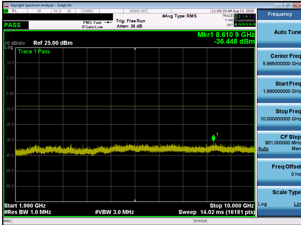
Plot 7-10. Conducted Spurious Plot (GSM Ch. 512)
