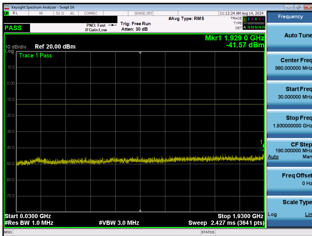
Plot 7-12. Conducted Spurious Plot (GSM Ch. 661)
