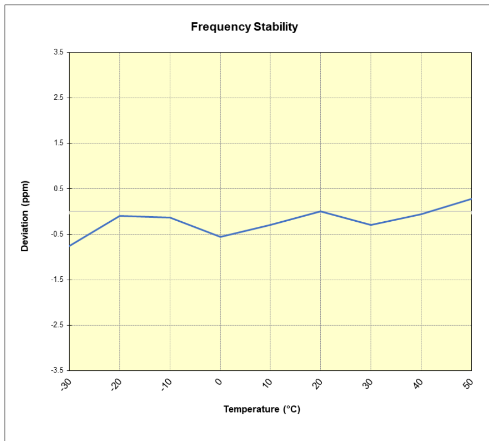
Plot 7-39. GSM PCS Frequency Stability Chart
