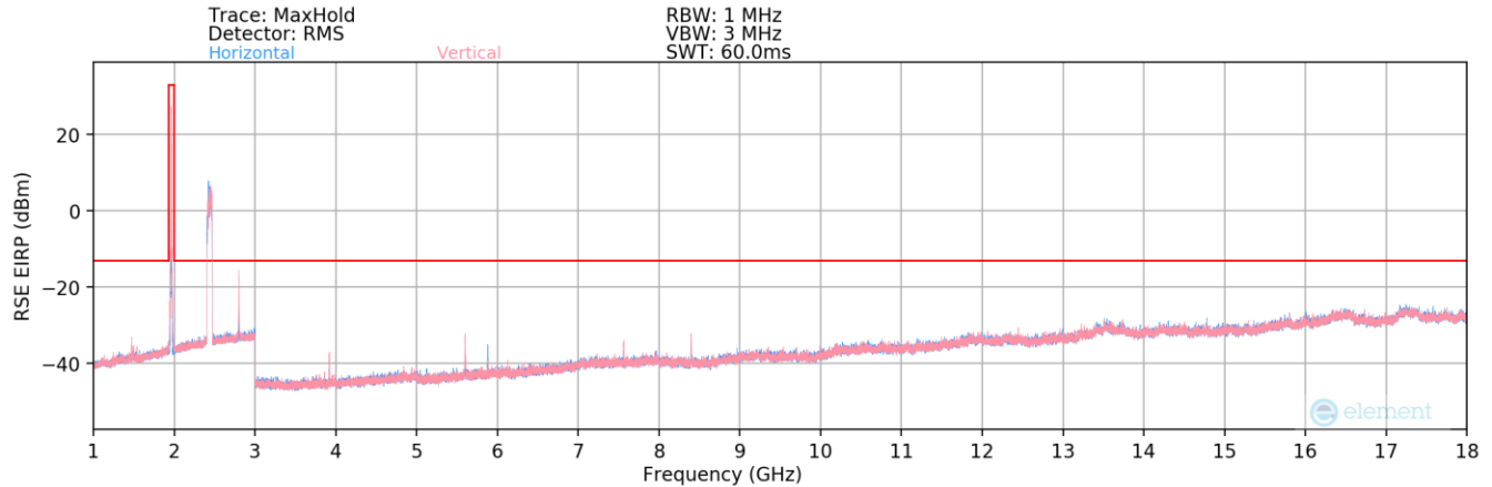
Plot 7-37. Radiated Spurious Plot (UMTS PCS) – Above 1GHz
