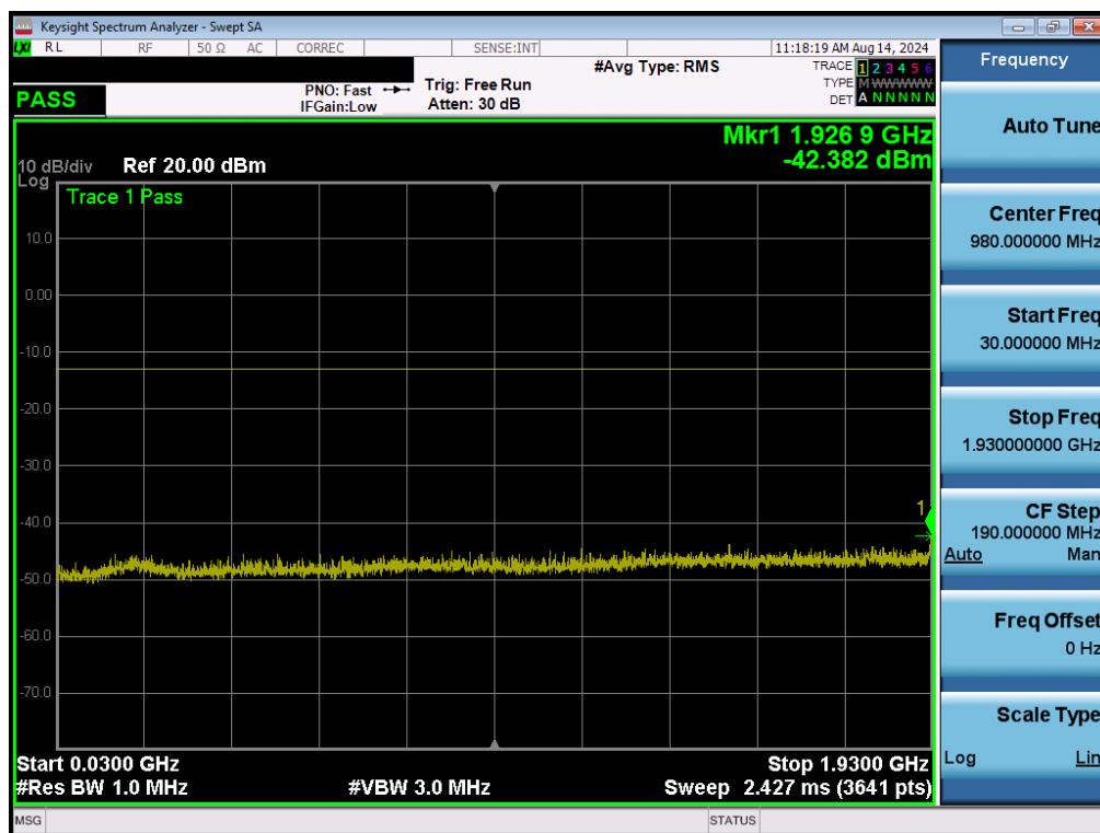
Plot 7-15. Conducted Spurious Plot (GSM Ch. 810)
