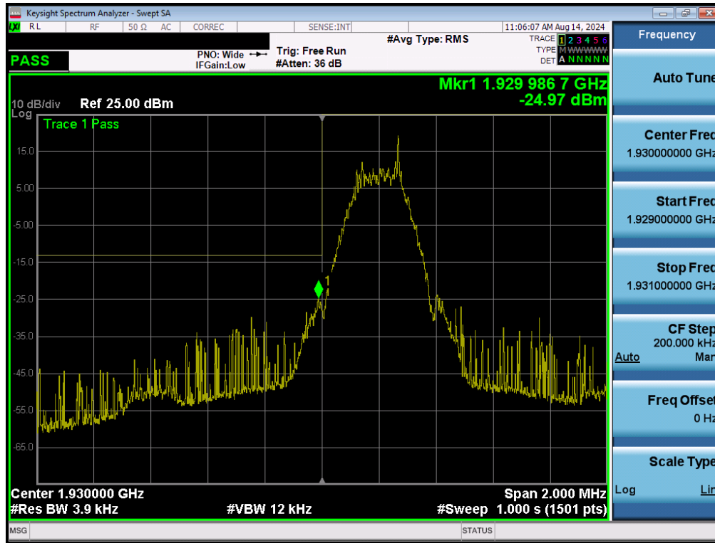
Plot 7-27. Lower Band Edge Plot (GSM PCS – Ch. 512)
