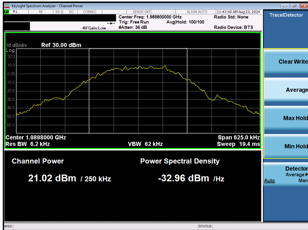
Plot 7-6. Conducted Power Output Data (GSM 1900 – High Channel)
