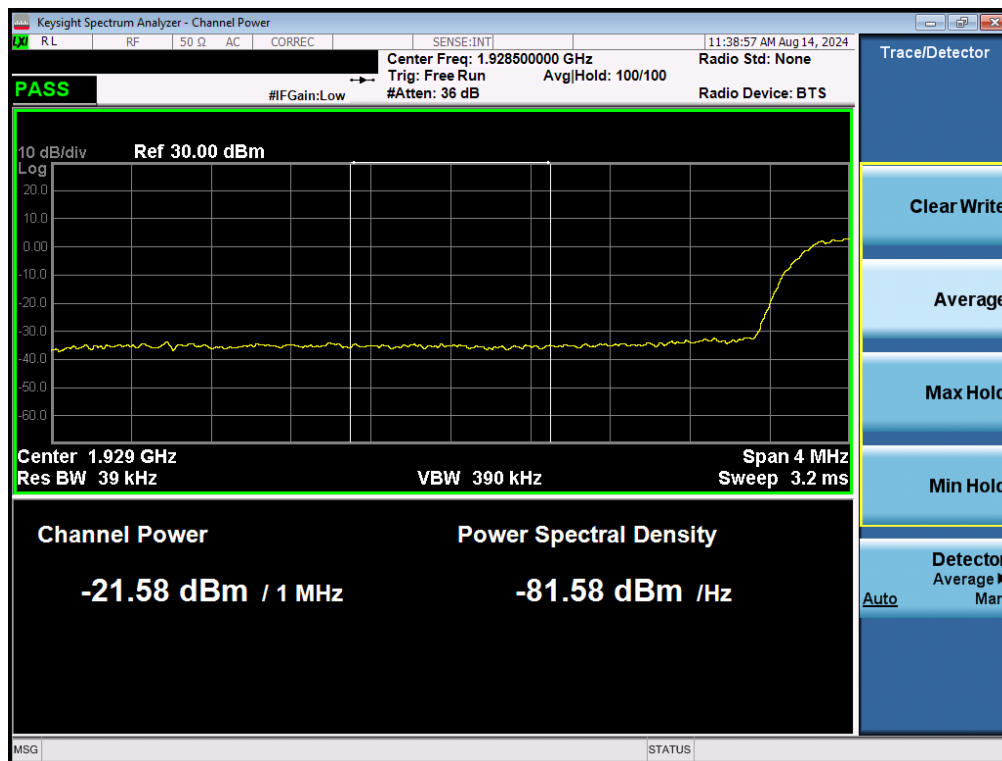
Plot 7-30. Extended Lower Band Edge Plot (UMTS PCS – Ch. 9662)
