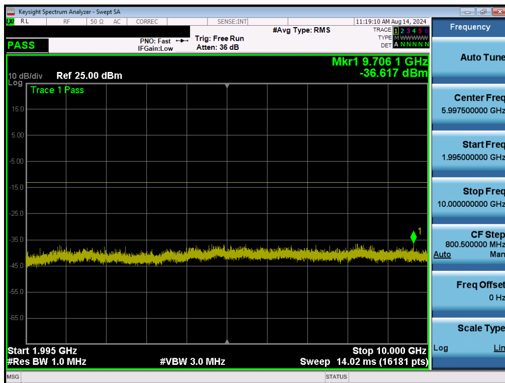
Plot 7-16. Conducted Spurious Plot (GSM Ch. 810)
