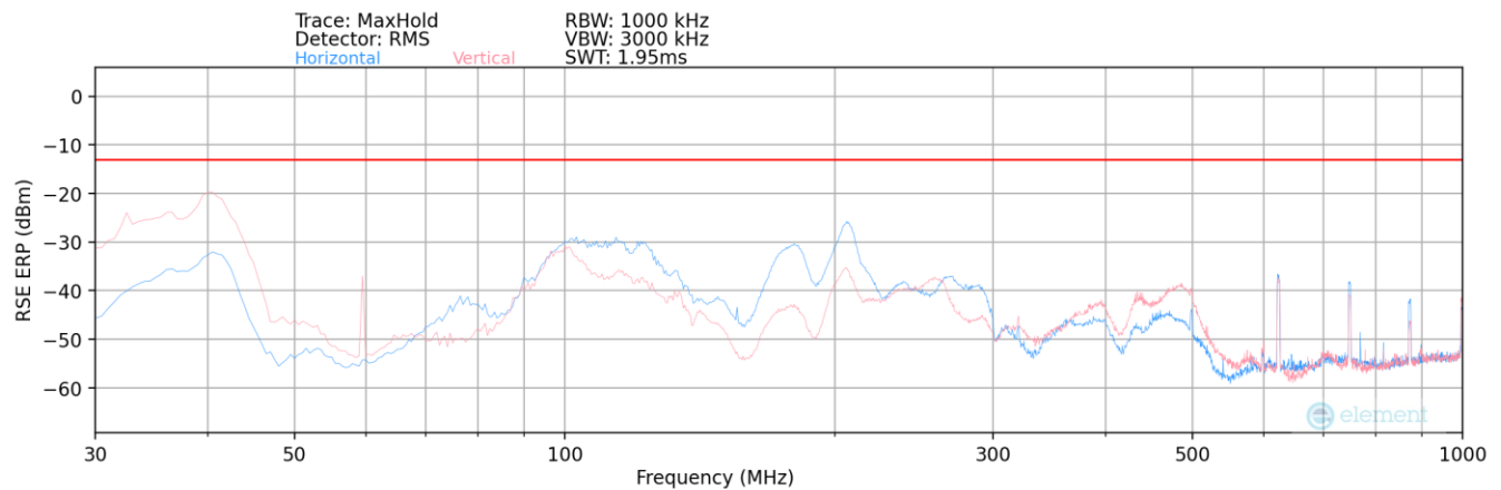
Plot 7-36. Radiated Spurious Plot (GSM PCS) – Below 1GHz
