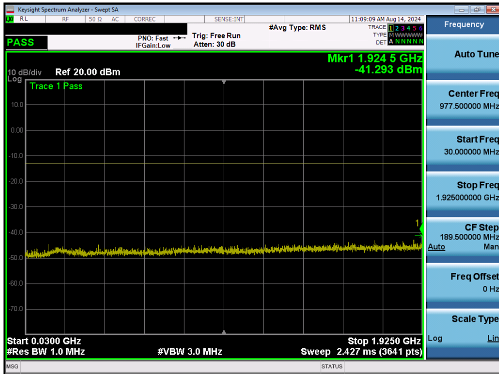
Plot 7-9. Conducted Spurious Plot (GSM Ch. 512)
