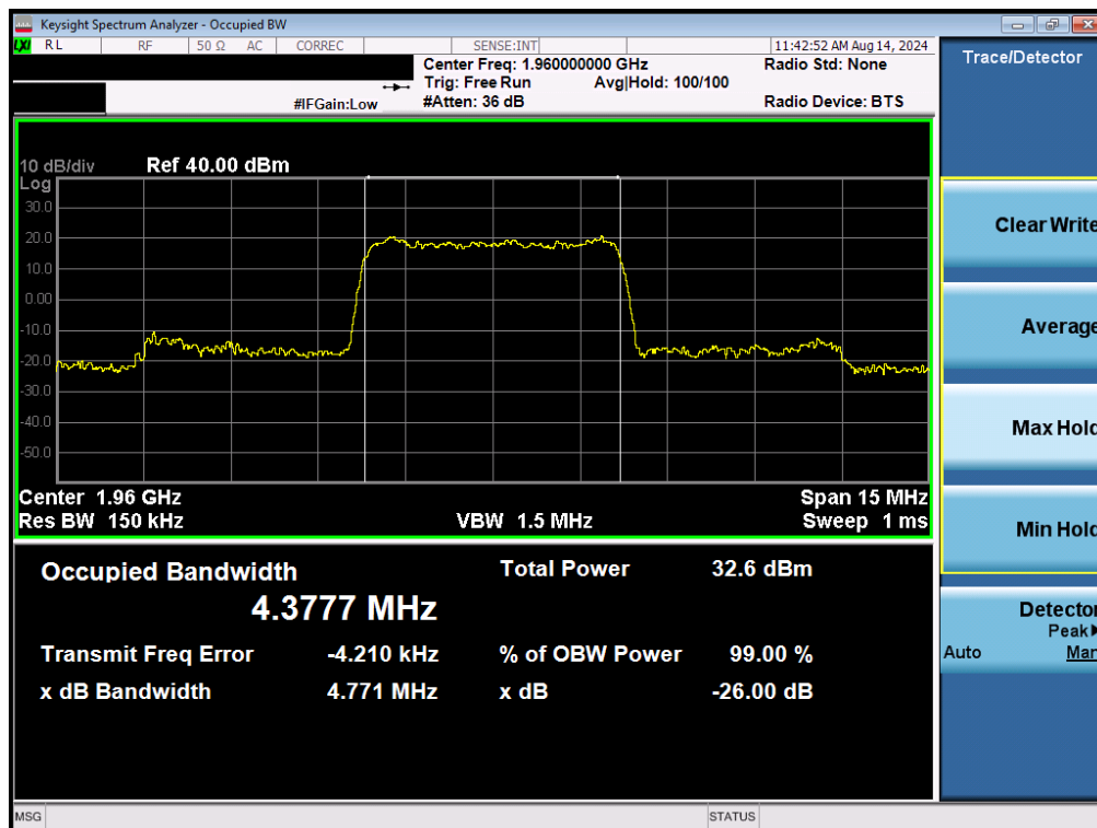
Plot 7-8. Occupied Bandwidth Plot (UMTS, Ch. 9800)
