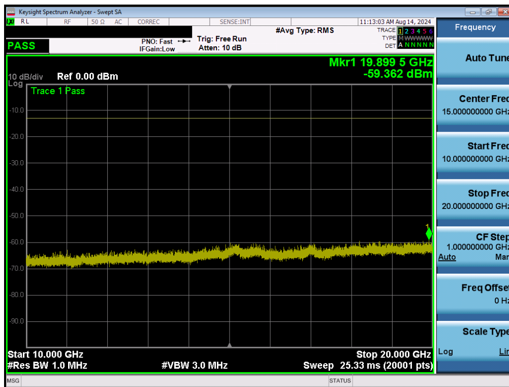
Plot 7-14. Conducted Spurious Plot (GSM Ch. 661)
