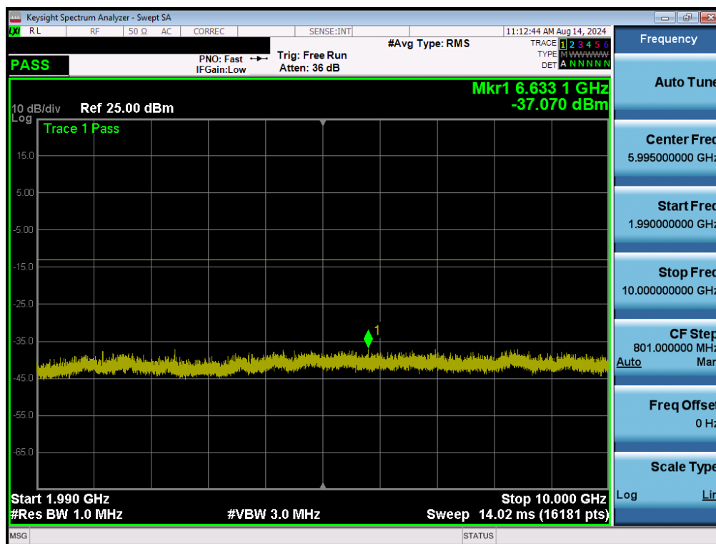
Plot 7-13. Conducted Spurious Plot (GSM Ch. 661)
