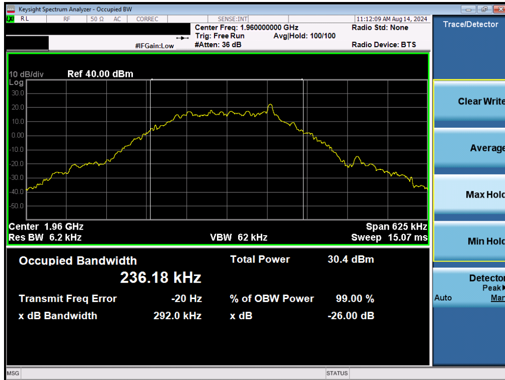
Plot 7-7. Occupied Bandwidth Plot (GSM, Ch. 661)
