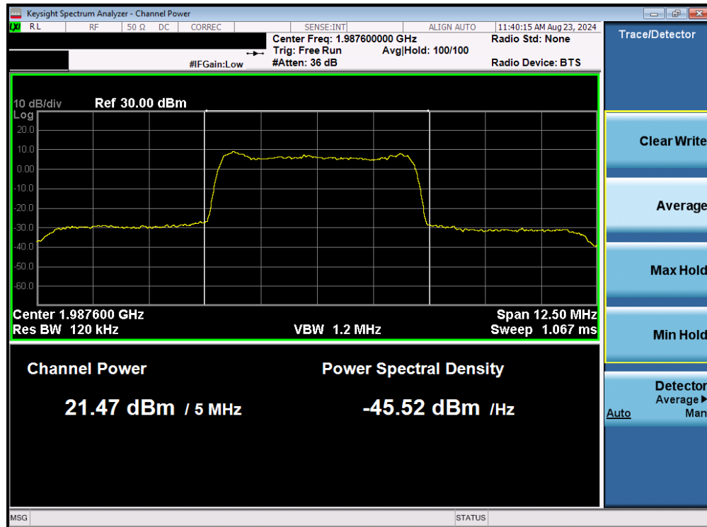
Plot 7-3. Conducted Power Output Data (UMTS 1900 – High Channel)
