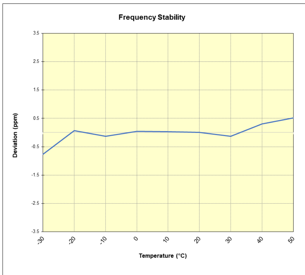
Plot 7-40. UMTS PCS Frequency Stability Chart
