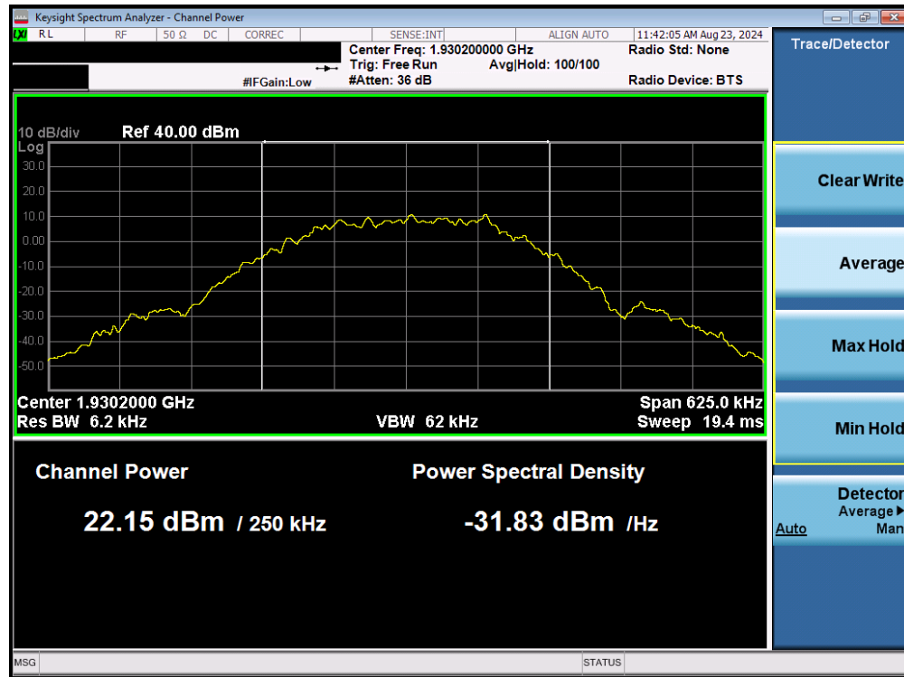
Plot 7-4. Conducted Power Output Data (GSM 1900 – Low Channel)
