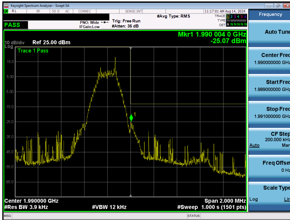
Plot 7-28. Upper Band Edge Plot (GSM PCS – Ch. 810)
