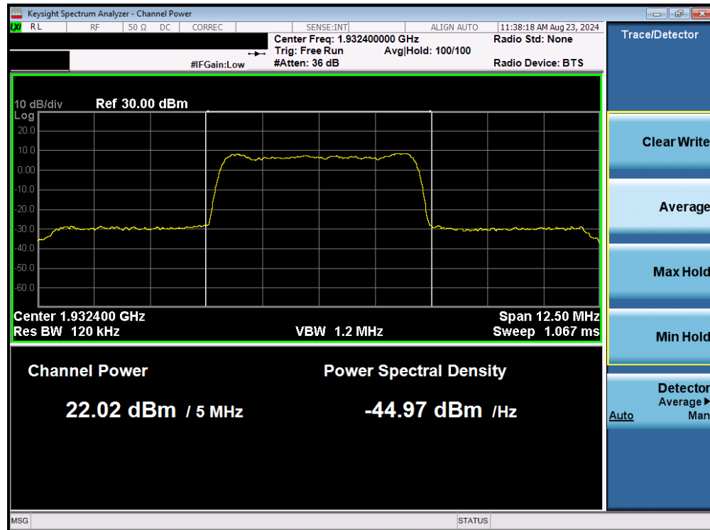
Plot 7-1. Conducted Power Output Data (UMTS 1900 – Low Channel)
