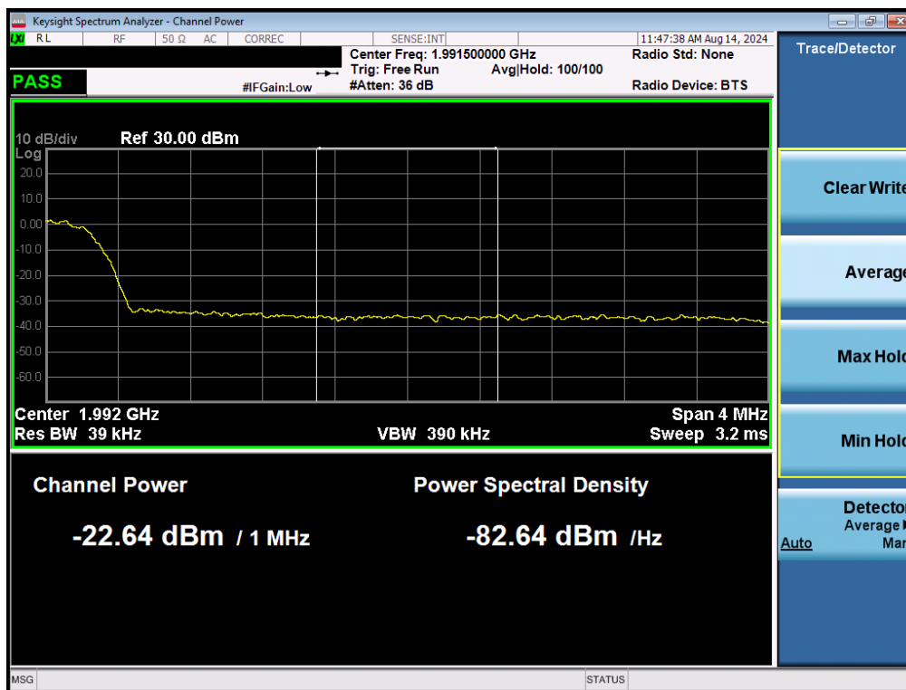
Plot 7-32. Extended Upper Band Edge Plot (UMTS PCS – Ch. 9938)
