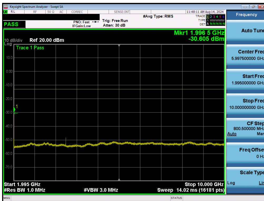
Plot 7-25. Conducted Spurious Plot (UMTS Ch. 9938)
