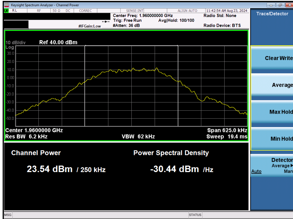
Plot 7-5. Conducted Power Output Data (GSM 1900 – Mid Channel)
