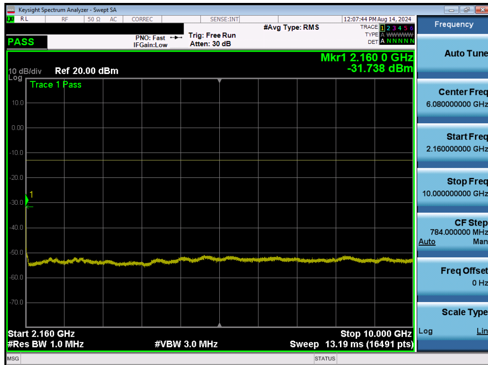
Plot 7-20. Conducted Spurious Plot (UMTS Ch. 1738- High Channel)
