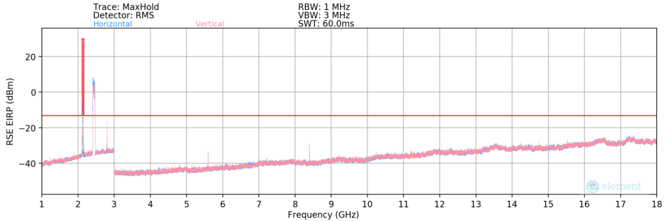
Plot 7-54. Radiated Spurious Plot (UMTS B4)
