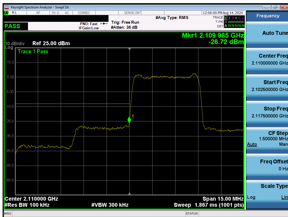
Plot 7-40. Lower Band Edge Plot (UMTS B4 – Ch. 1537)
