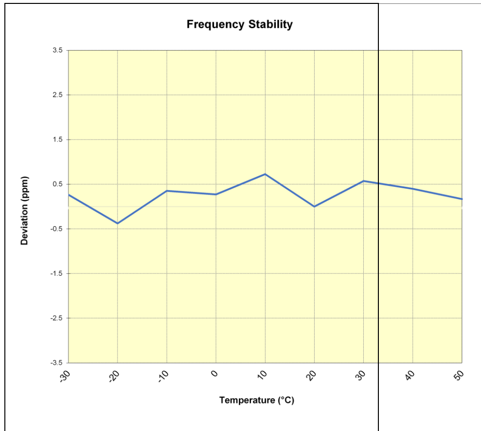
Plot 7-57. UMTS B4 Frequency Stability Chart
