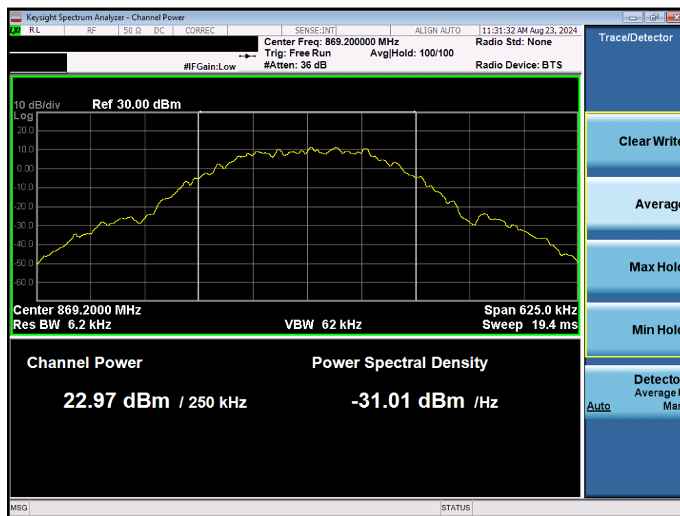
Plot 7-4. Conducted Power Output Data (GSM 850 – Low Channel)
