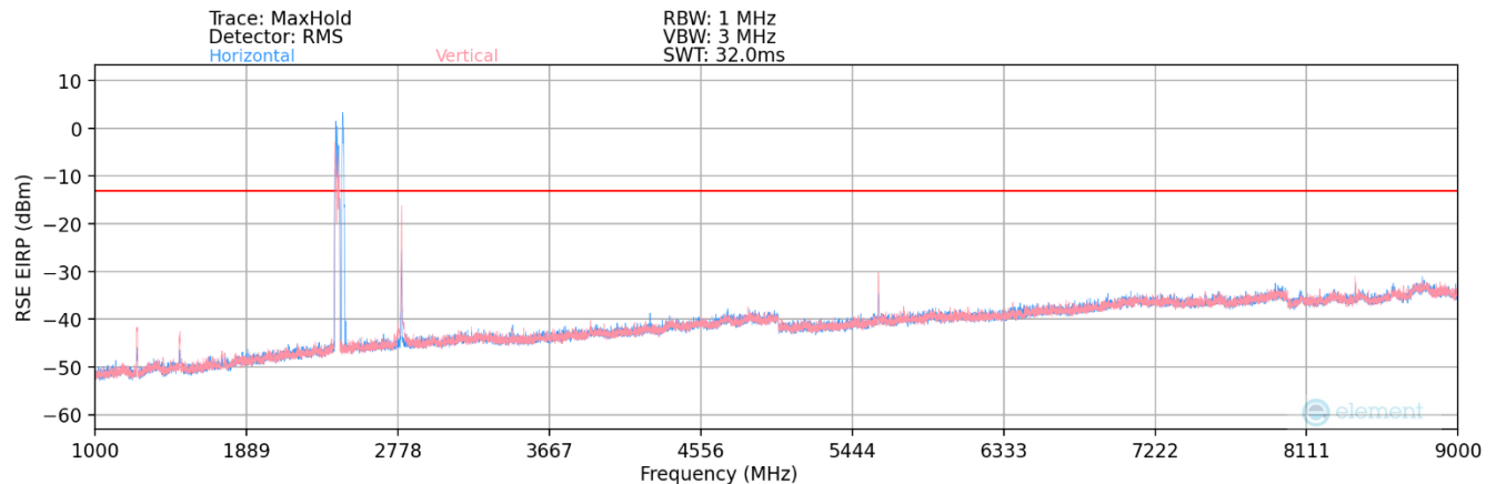
Plot 7-33. Radiated Spurious Plot (UMTS Cell) – Above 1GHz
