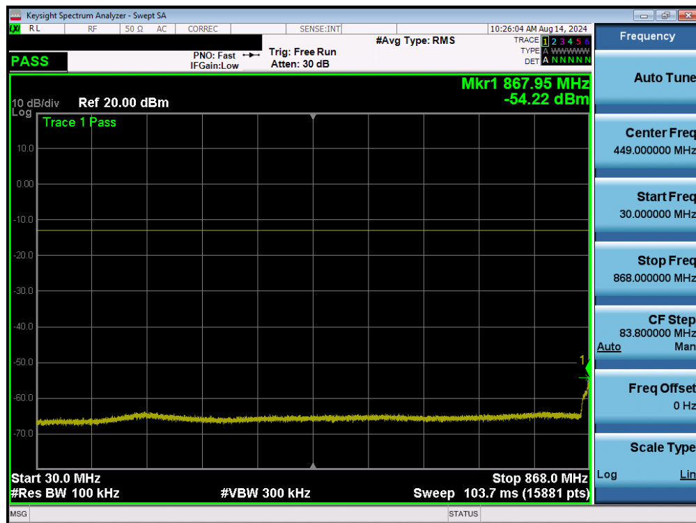
Plot 7-21. Conducted Spurious Plot (UMTS Ch. 4408)
