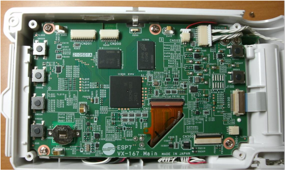
Rear panel removed (RF module mounted board)
