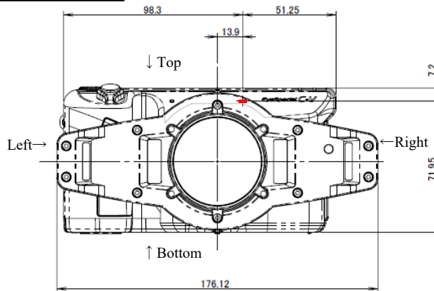
Rear face
