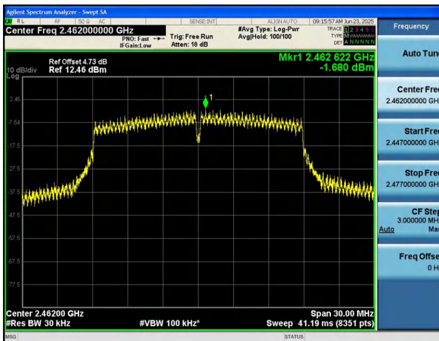
Power_Spectral_Density_HVNT_ANT1_802_11n(HT20)_2462
