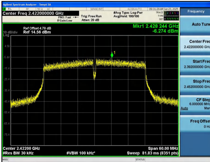
Power_Spectral_Density_HVNT_ANT1_802_11n(HT40)_2422
