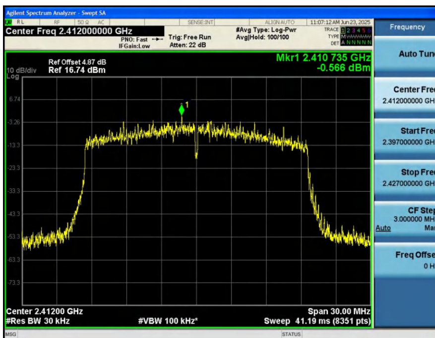
Power_Spectral_Density_HVNT_ANT1_802_11ax(HE20)_2412
