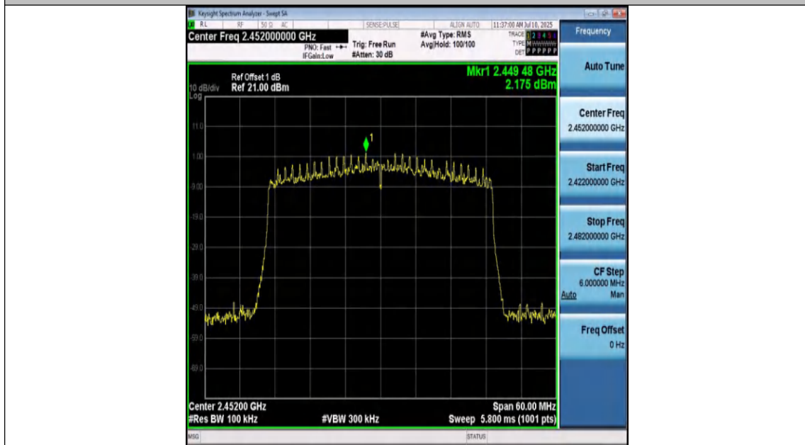
11AX40SISO-Ant1-2452-0~Reference-PASS
