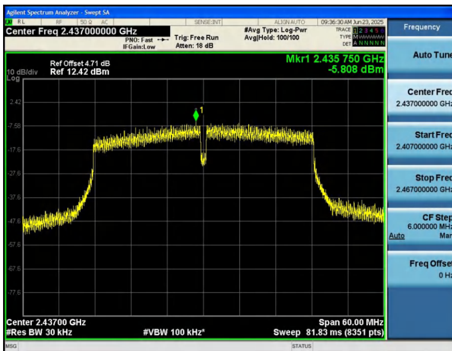
Power_Spectral_Density_HVNT_ANT1_802_11n(HT40)_2437
