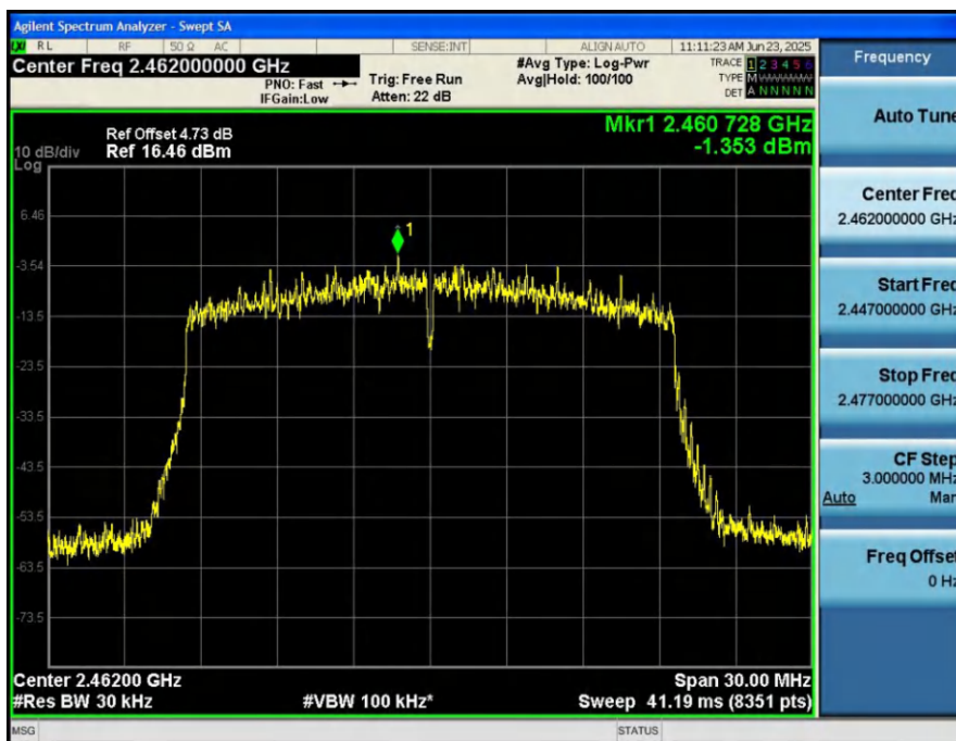
Power_Spectral_Density_HVNT_ANT1_802_11ax(HE20)_2462
