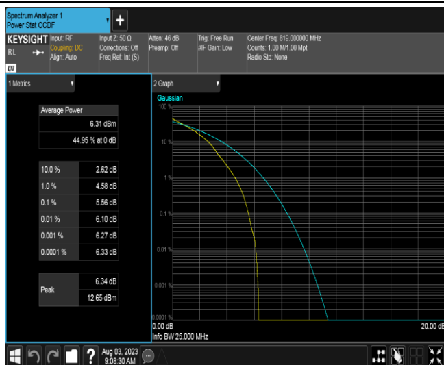
Band26B-1.4MHz-QPSK-26740-6RB#0
