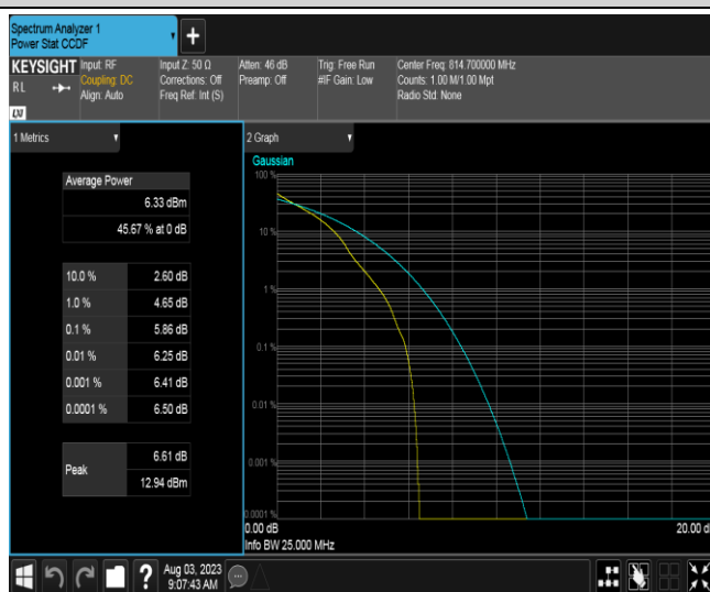
Band26B-1.4MHz-QPSK-26697-6RB#0
