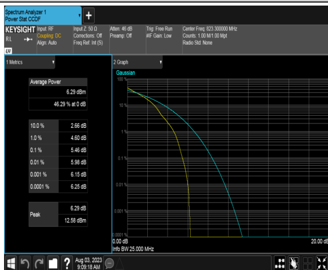
Band26B-1.4MHz-QPSK-26783-1RB#0
