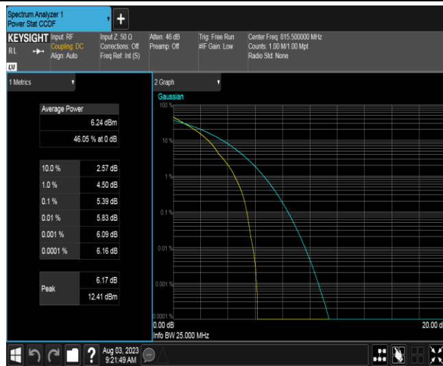
Band26B-3MHz-QPSK-26705-15RB#0
