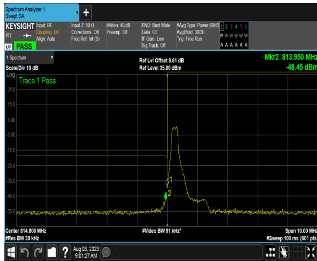
Band26B-1.4MHz-16QAM-26697-1RB#5
