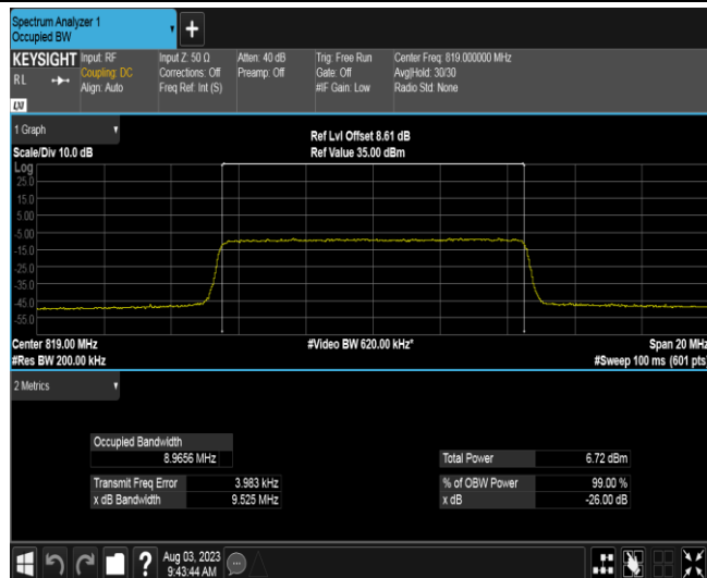
Band26B-10MHz-16QAM-26740-50RB#0
