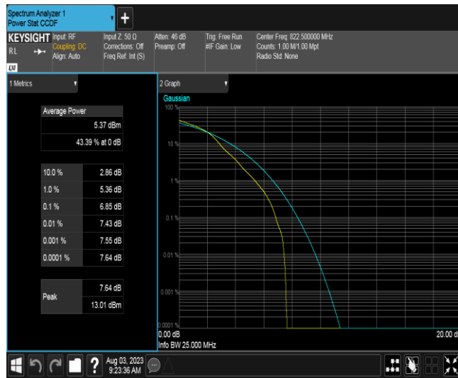
Band26B-3MHz-16QAM-26775-15RB#0
