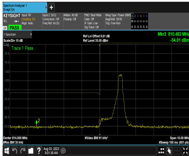
Band26B-1.4MHz-QPSK-26697-6RB#0
