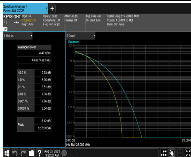
Band26B-3MHz-16QAM-26705-15RB#0
