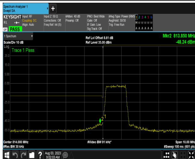
Band26B-1.4MHz-16QAM-26697-6RB#0
