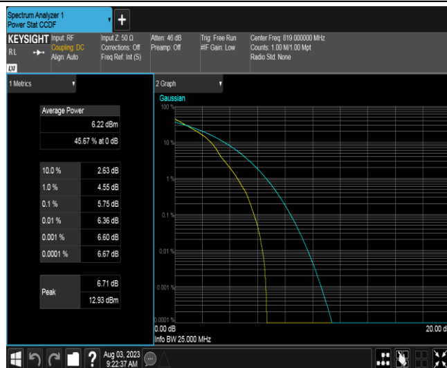
Band26B-3MHz-QPSK-26740-1RB#0
