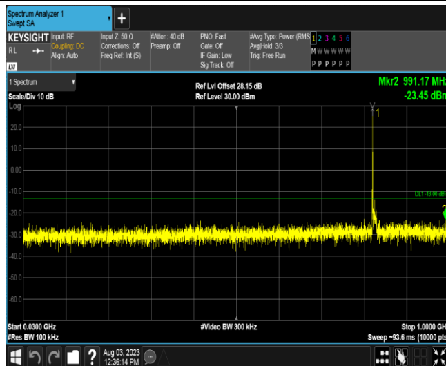
Band26A-10MHz-16QAM-26840-1RB#0-Range1:30~1000MHz
