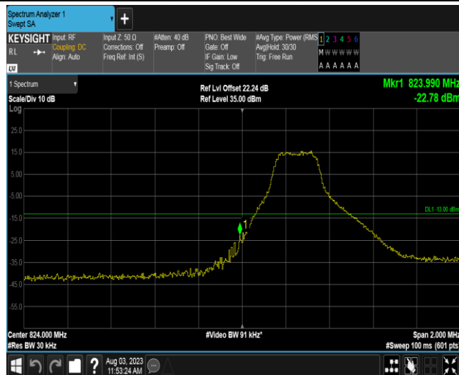
Band26A-1.4MHz-16QAM-26797-1RB#5
