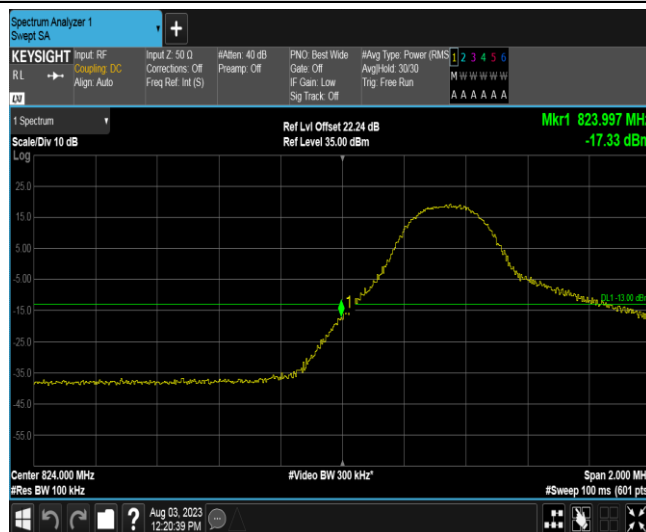
Band26A-5MHz-16QAM-26815-1RB#0
