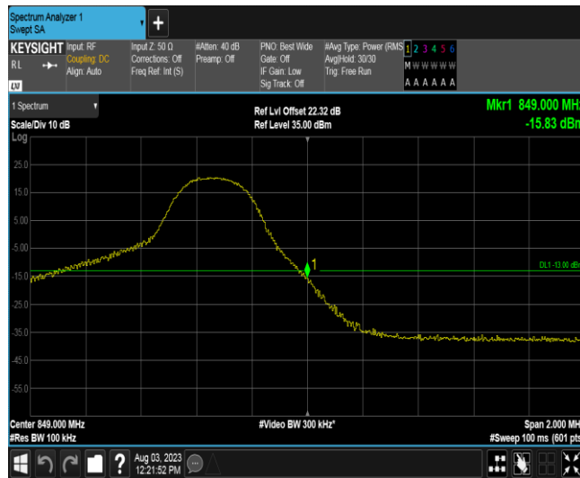
Band26A-5MHz-QPSK-27015-25RB#0
