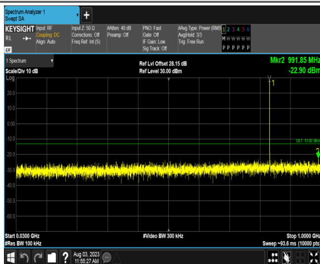
Band26A-1.4MHz-QPSK-26915-1RB#0-Range1:30~1000MHz
