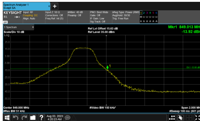
Band26A-3MHz-QPSK-27025-15RB#0
