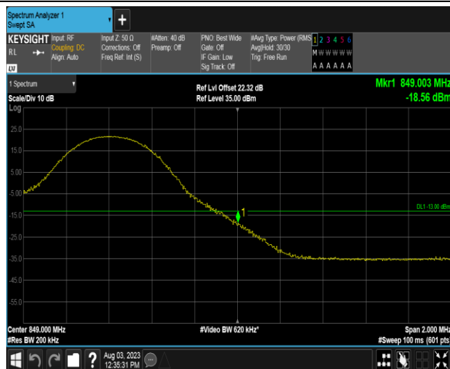
Band26A-10MHz-QPSK-26990-1RB#49
