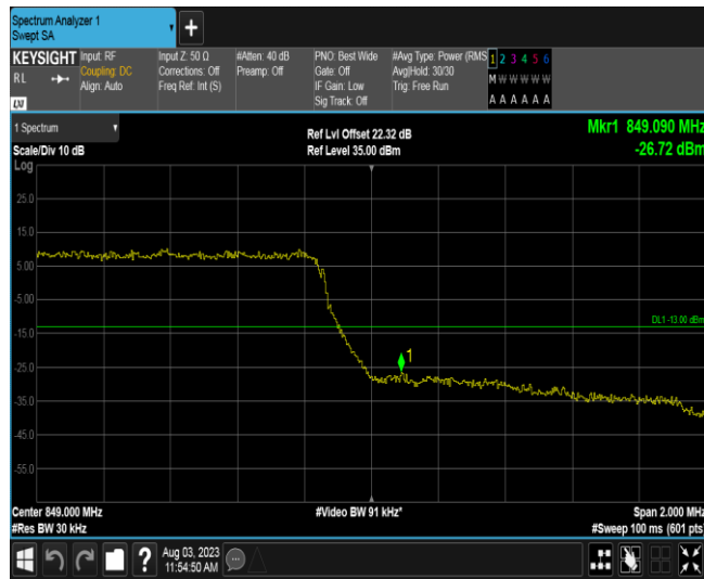
Band26A-1.4MHz-16QAM-26797-1RB#0
