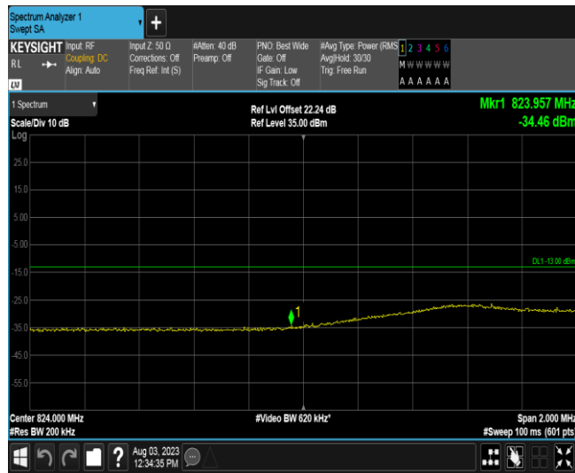
Band26A-10MHz-16QAM-26840-50RB#0
