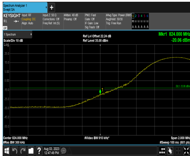
Band26A-15MHz-QPSK-26865-1RB#74
