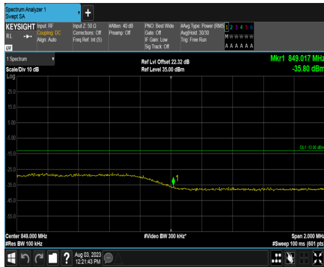
Band26A-5MHz-16QAM-27015-1RB#24
