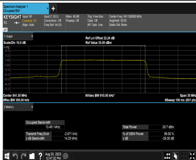
Band26A-15MHz-16QAM-26965-75RB#0
