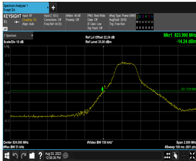
Band26A-3MHz-16QAM-26805-1RB#14
