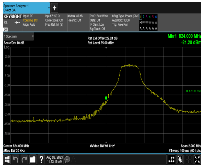
Band26A-1.4MHz-QPSK-26797-1RB#5
