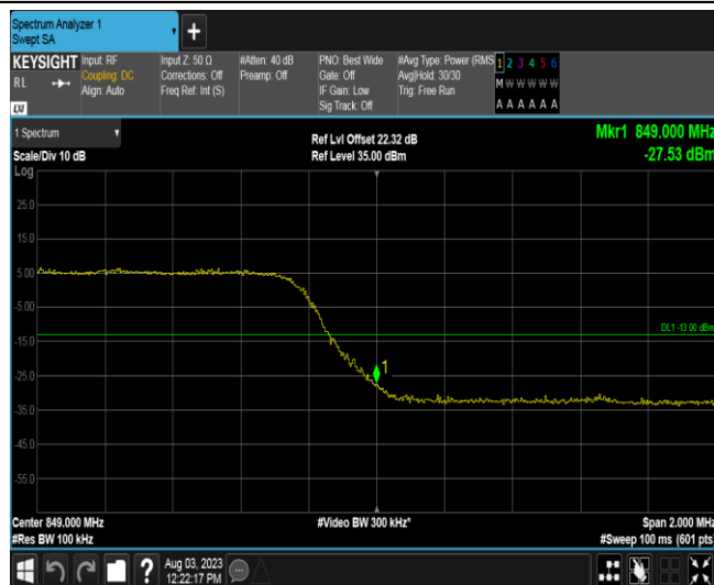
Band26A-5MHz-16QAM-27015-25RB#0
