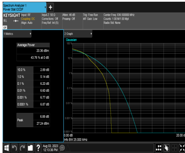
Band26A-3MHz-16QAM-26915-15RB#0
