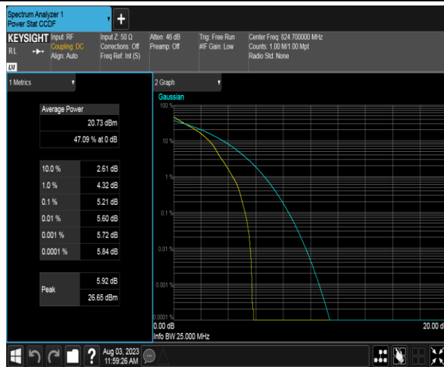
Band26A-1.4MHz-QPSK-26797-6RB#0
