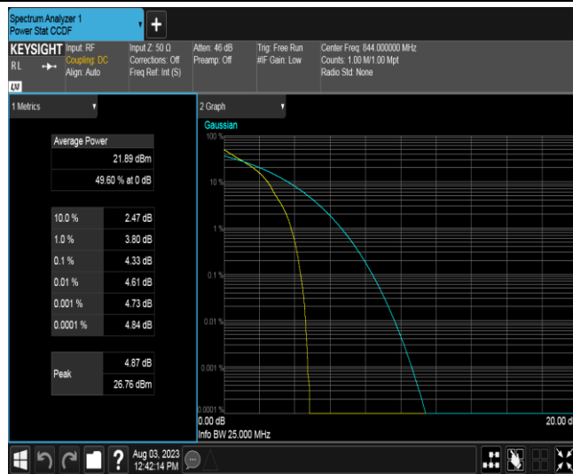
Band26A-10MHz-QPSK-26990-50RB#0
