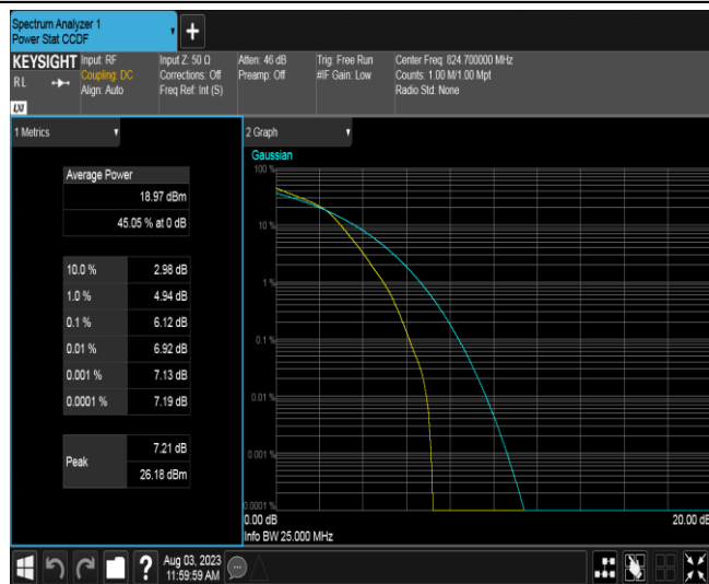
Band26A-1.4MHz-16QAM-26797-6RB#0
