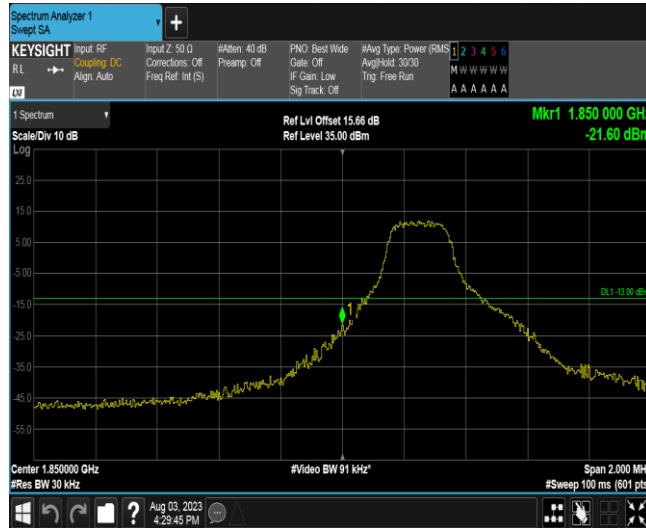
Band25-1.4MHz-QPSK-26047-1RB#5
