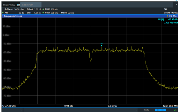
802.11n40 on Channel 03
