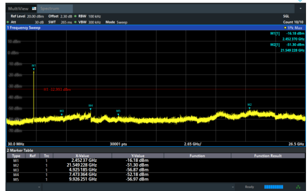
802.11n40 on Channel 06
