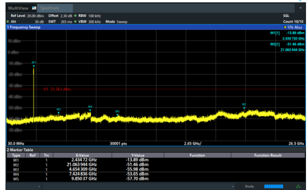
802.11n40 on Channel 03
