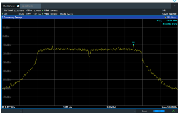
802.11n20 on Channel 06
