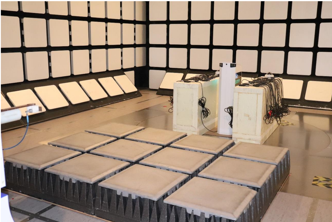
Photograph 4. Radiated emission test setup 18-26.5 GHz
