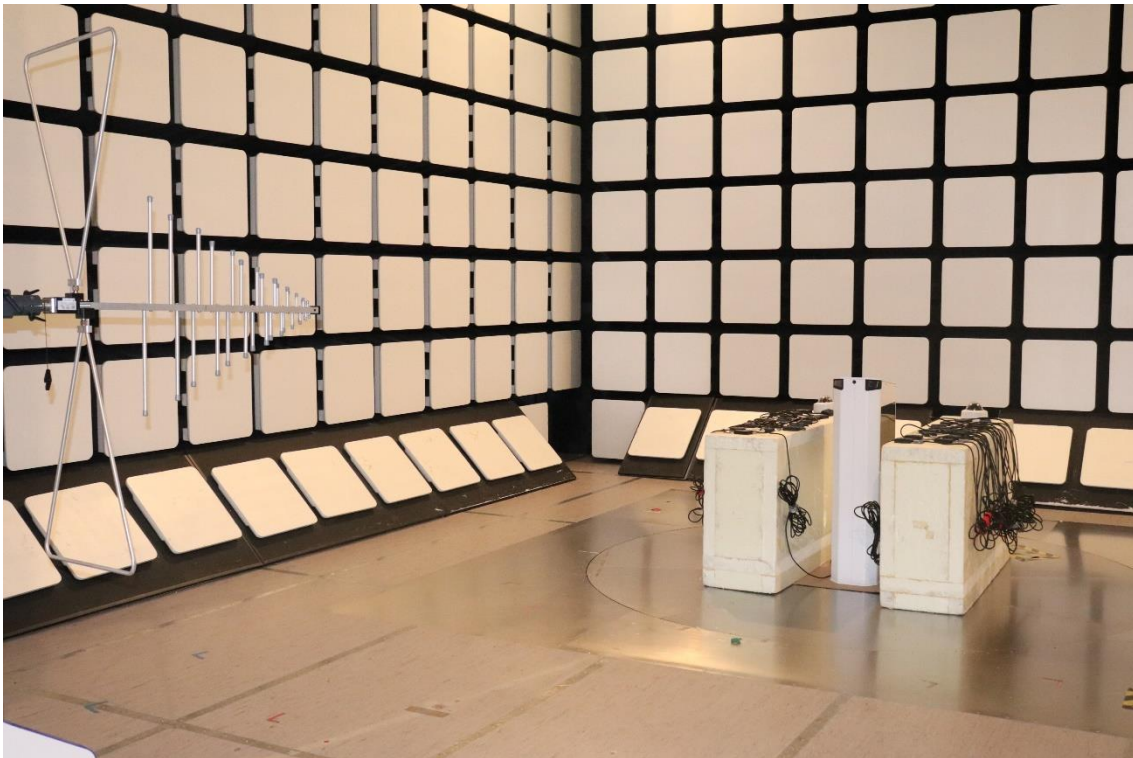
Photograph 2. Radiated emission test setup (30-1000 MHz)
