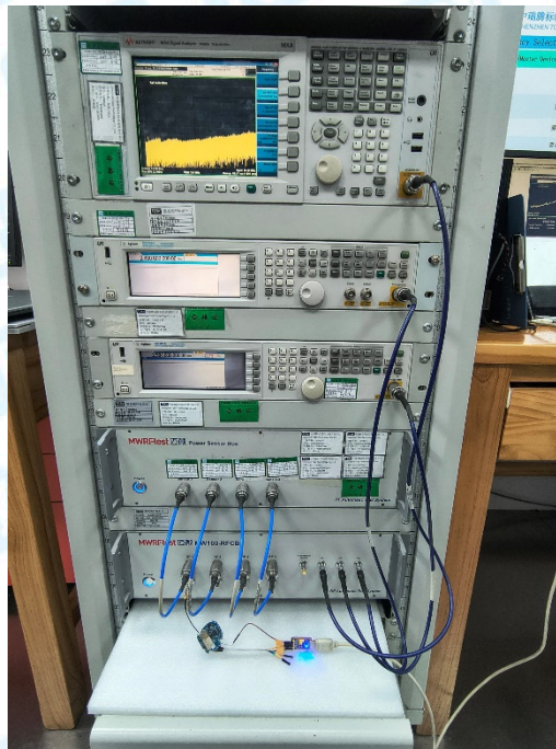
Photo of Setup for RF Conducted Emission
