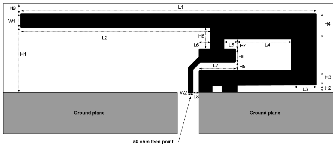
Figure 1. IFA Dimensions
