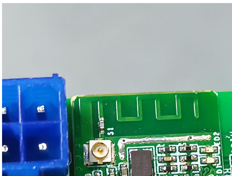
This Antenna was Not used
