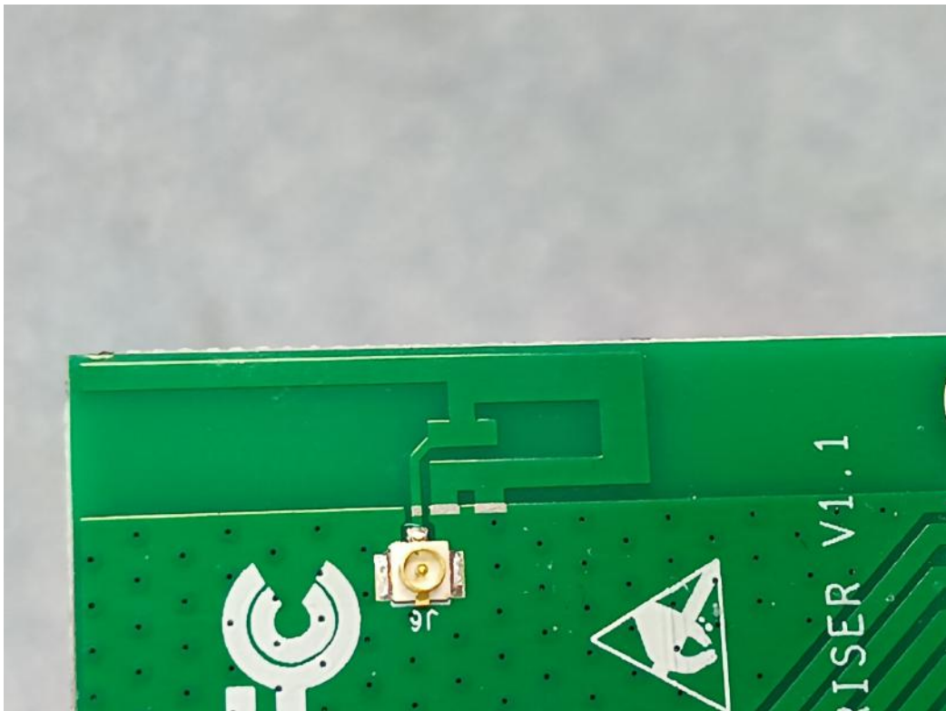
Wi-Fi Antenna
