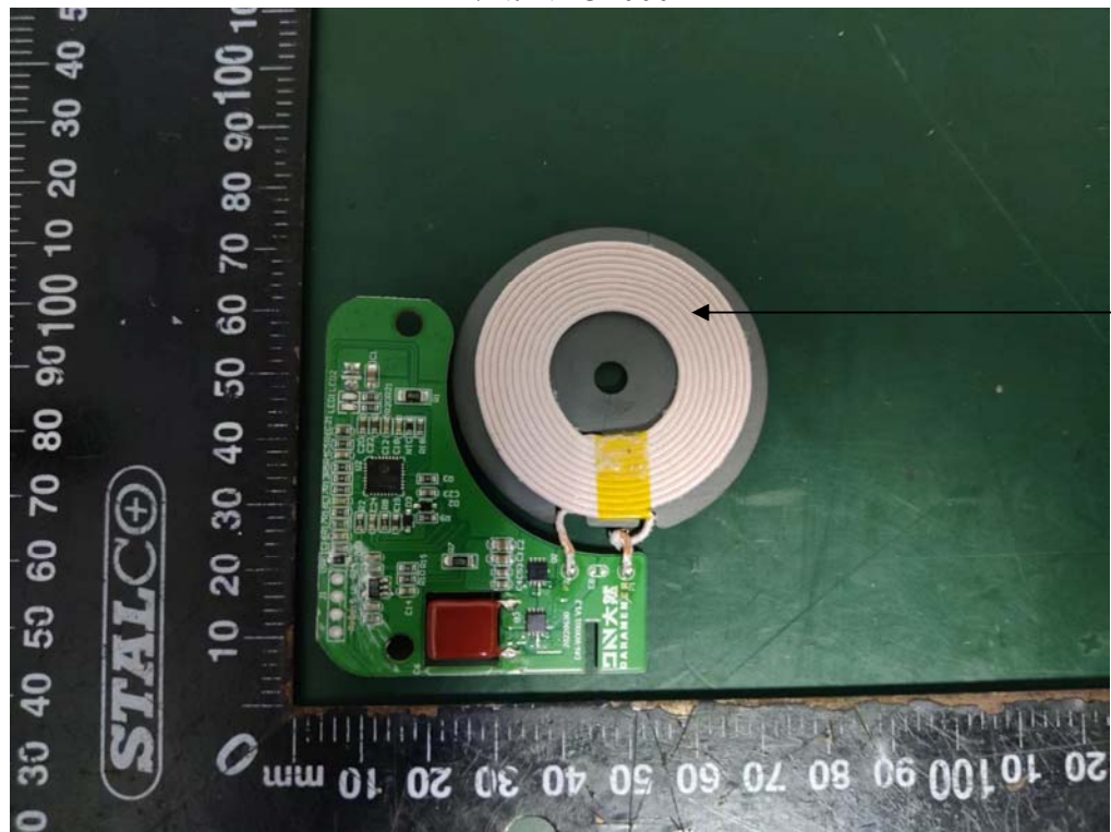
Coil Antenna
