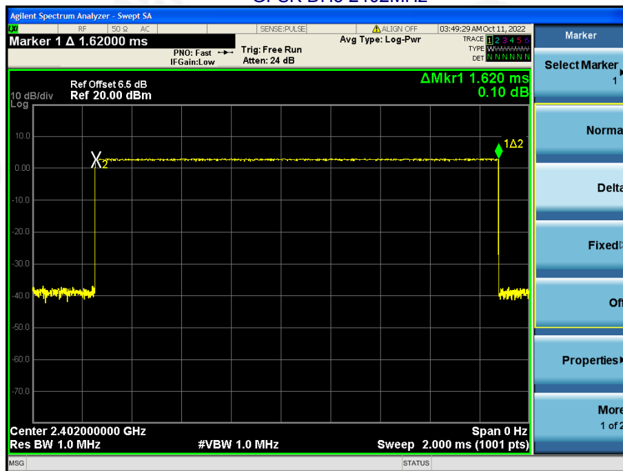
GFSK DH3 2402MHz
