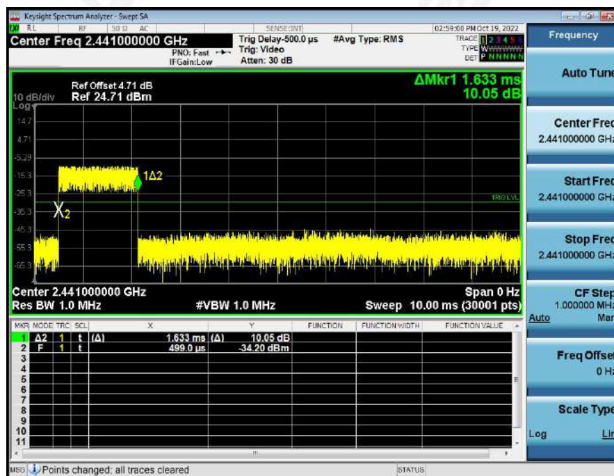
GFSK DH3 2441MHz
