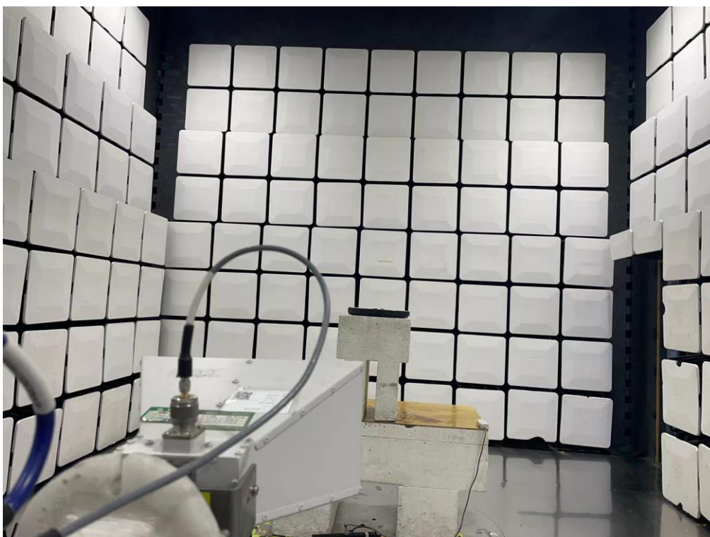
Above 1GHz Vertical
