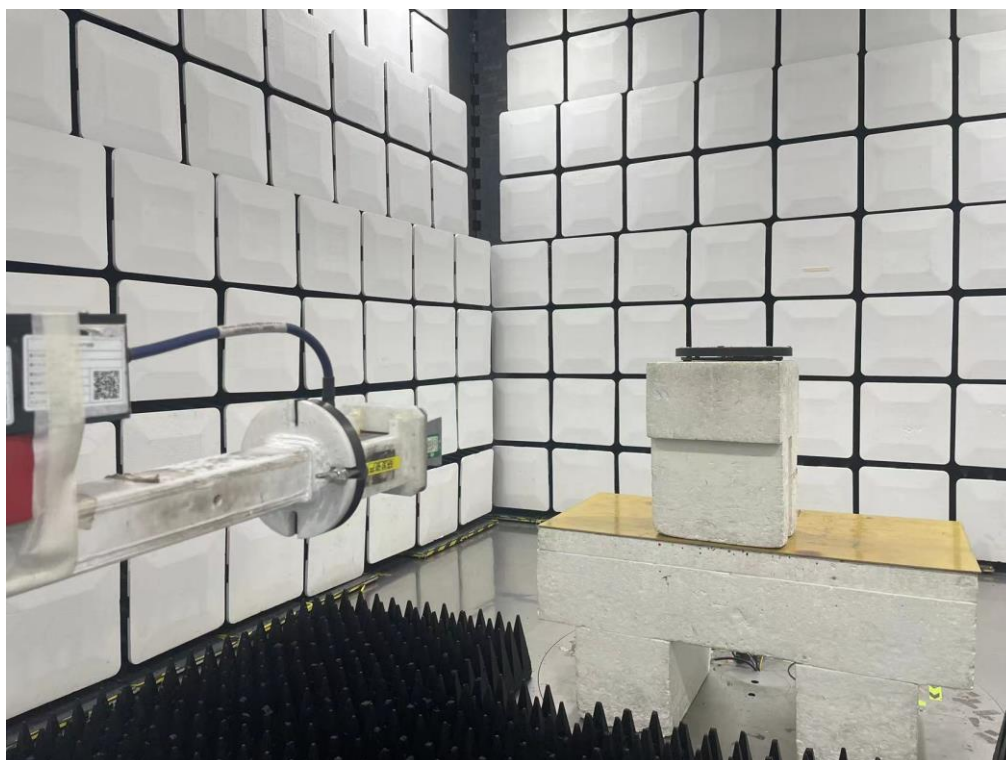
Above 18GHz Vertical
