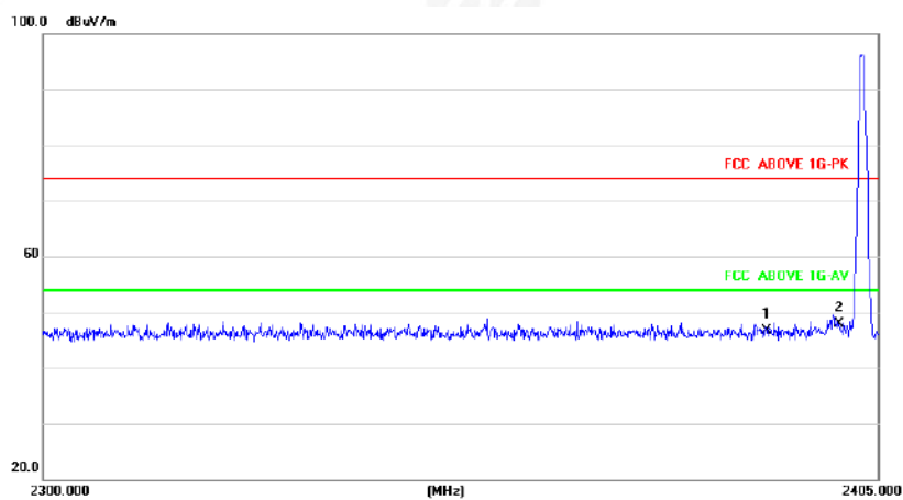
2402MHz Horizontal
