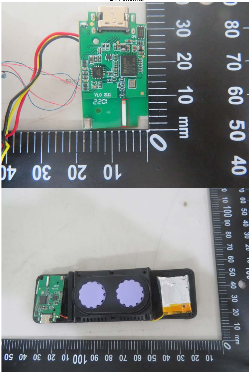
BT Antenna
