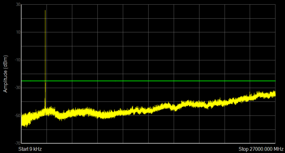
Band7 16QAM BW=15MHz Channel=21375 RB Size=1 Position=#0
