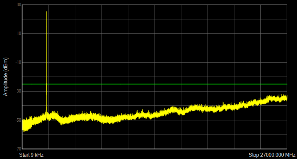
Band7 16QAM BW=20MHz Channel=20850 RB Size=1 Position=#0
