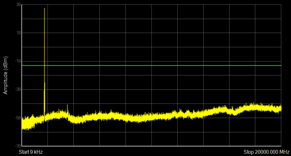
Band66 16QAM BW=15MHz Channel=132597 RB Size=1 Position=#0
