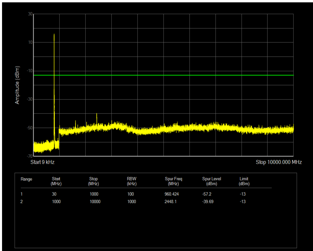
Band18 16QAM BW=5MHz Channel=23875 RB Size=1 Position=#0
