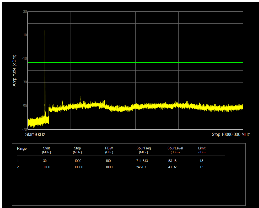
Band18 16QAM BW=5MHz Channel=23875 RB Size=25 Position=#0
