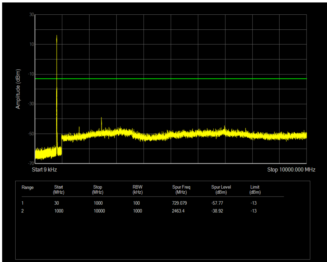
Band18 QPSK BW=5MHz Channel=23925 RB Size=25 Position=#0
