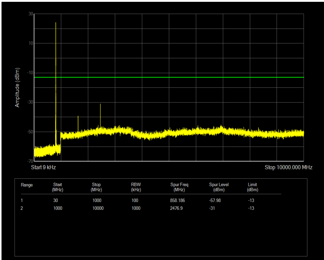
Band18 16QAM BW=5MHz Channel=23975 RB Size=25 Position=#0
