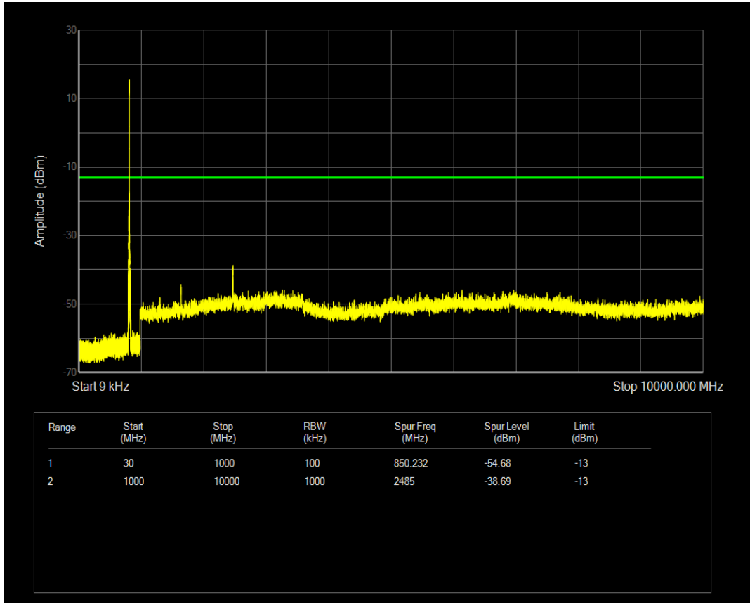
Band18 16QAM BW=5MHz Channel=23975 RB Size=1 Position=#0
