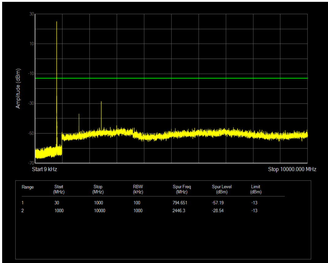
Band18 QPSK BW=5MHz Channel=23875 RB Size=25 Position=#0
