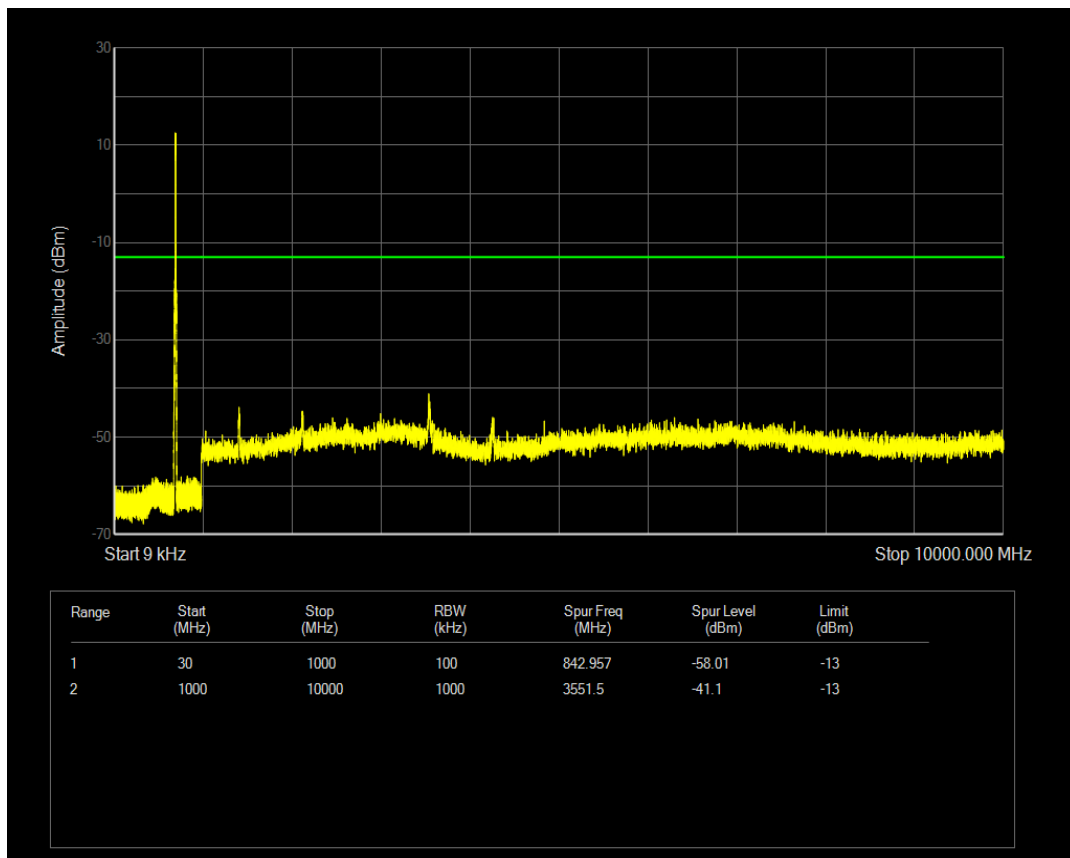
Band18 QPSK BW=5MHz Channel=23875 RB Size=1 Position=#0
