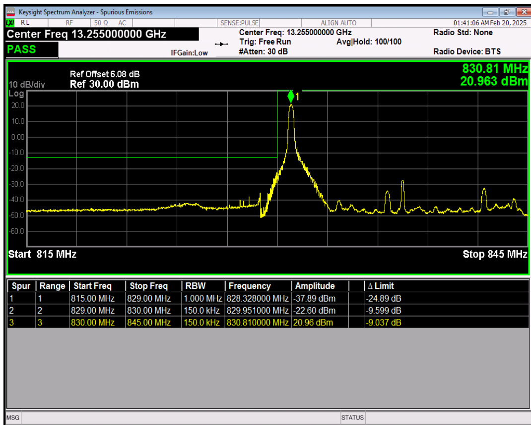
Band19 16QAM BW=15MHz Channel=24075 RB Size=1 Position=#Max
