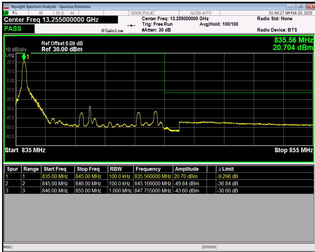
Band19 QPSK BW=10MHz Channel=24100 RB Size=1 Position=#Max
