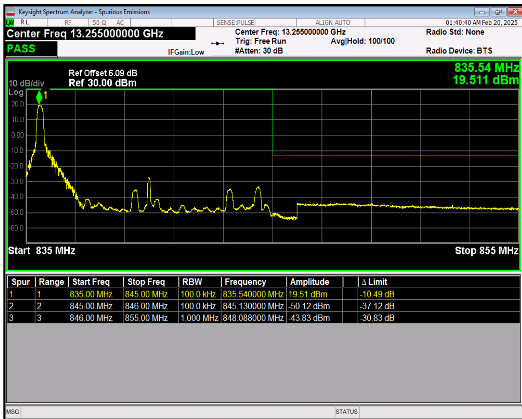
Band19 16QAM BW=10MHz Channel=24100 RB Size=1 Position=#Max
