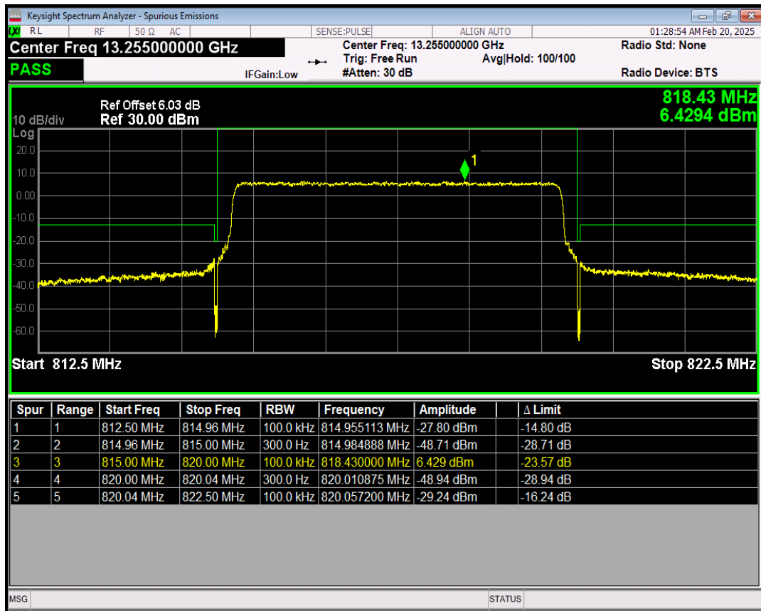
Band18 16QAM BW=5MHz Channel=23875 RB Size=1 Position=#0
