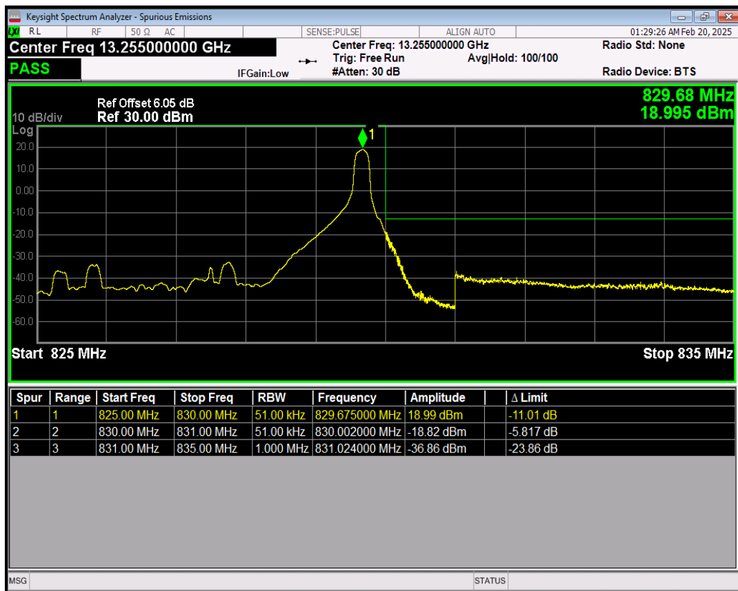
Band18 QPSK BW=5MHz Channel=23975 RB Size=25 Position=#0
