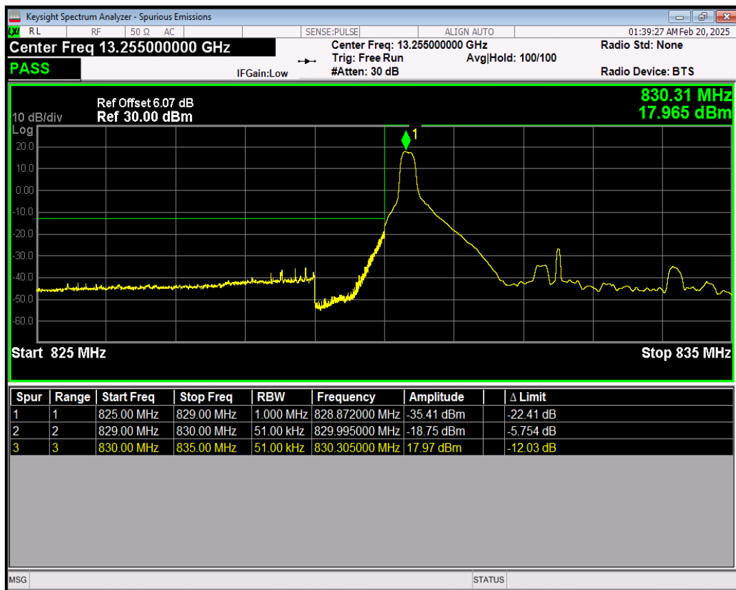
Band19 16QAM BW=5MHz Channel=24025 RB Size=1 Position=#Max
