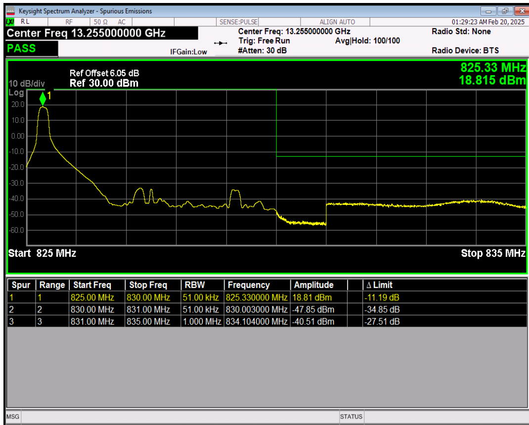
Band18 QPSK BW=5MHz Channel=23975 RB Size=1 Position=#Max
