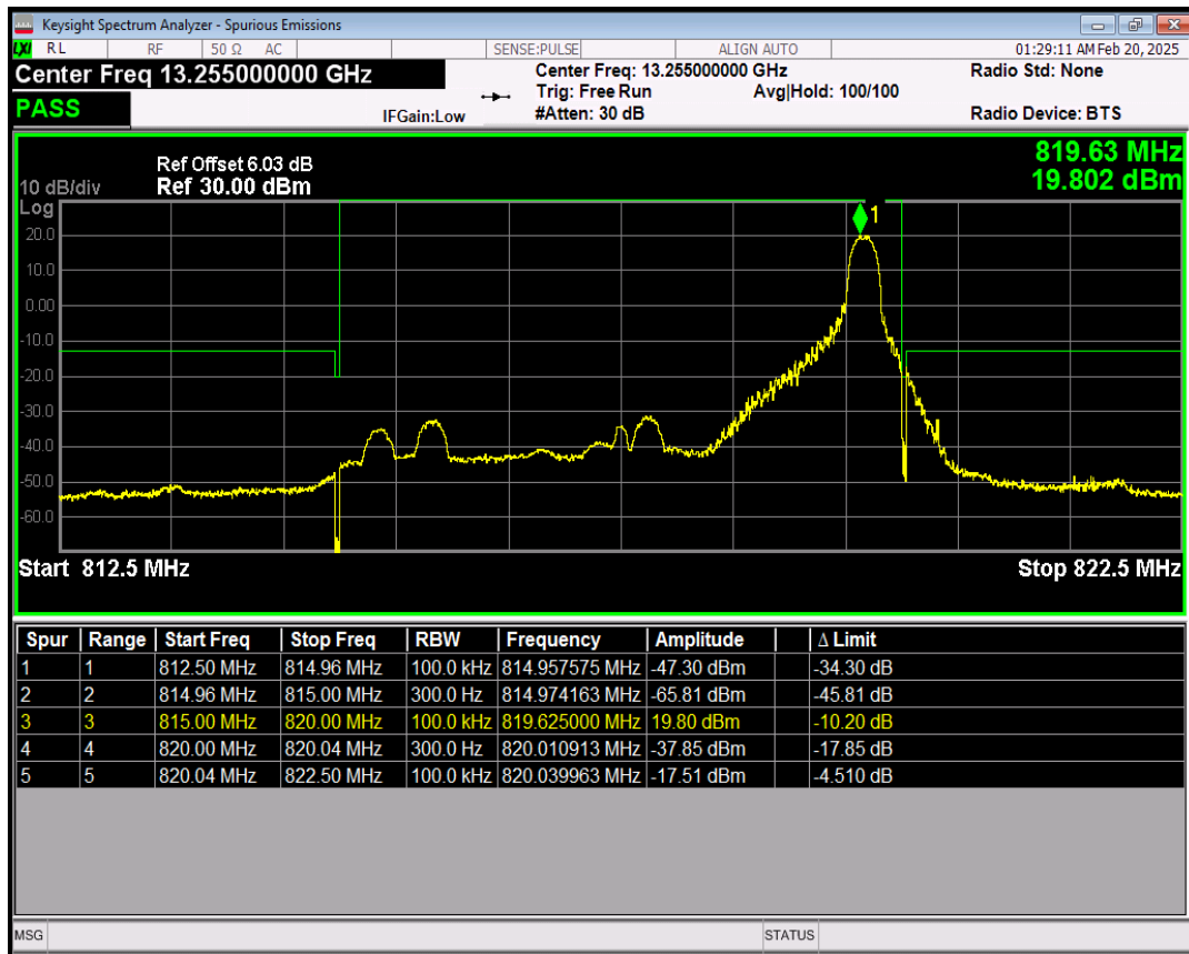
Band18 16QAM BW=5MHz Channel=23875 RB Size=25 Position=#0
