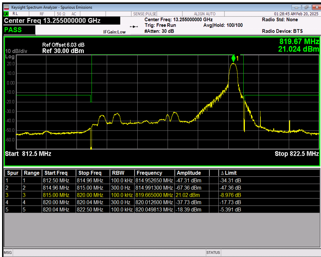
Band18 QPSK BW=5MHz Channel=23875 RB Size=25 Position=#0
