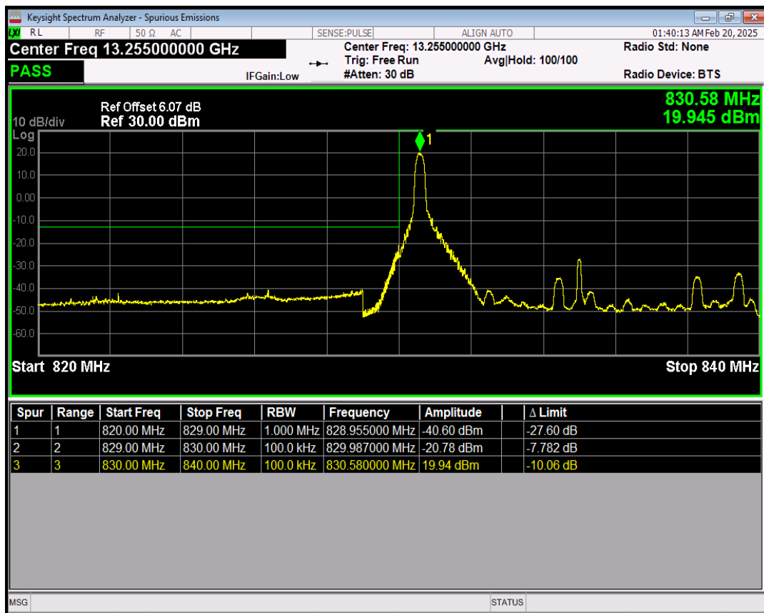
Band19 16QAM BW=10MHz Channel=24050 RB Size=1 Position=#Max
