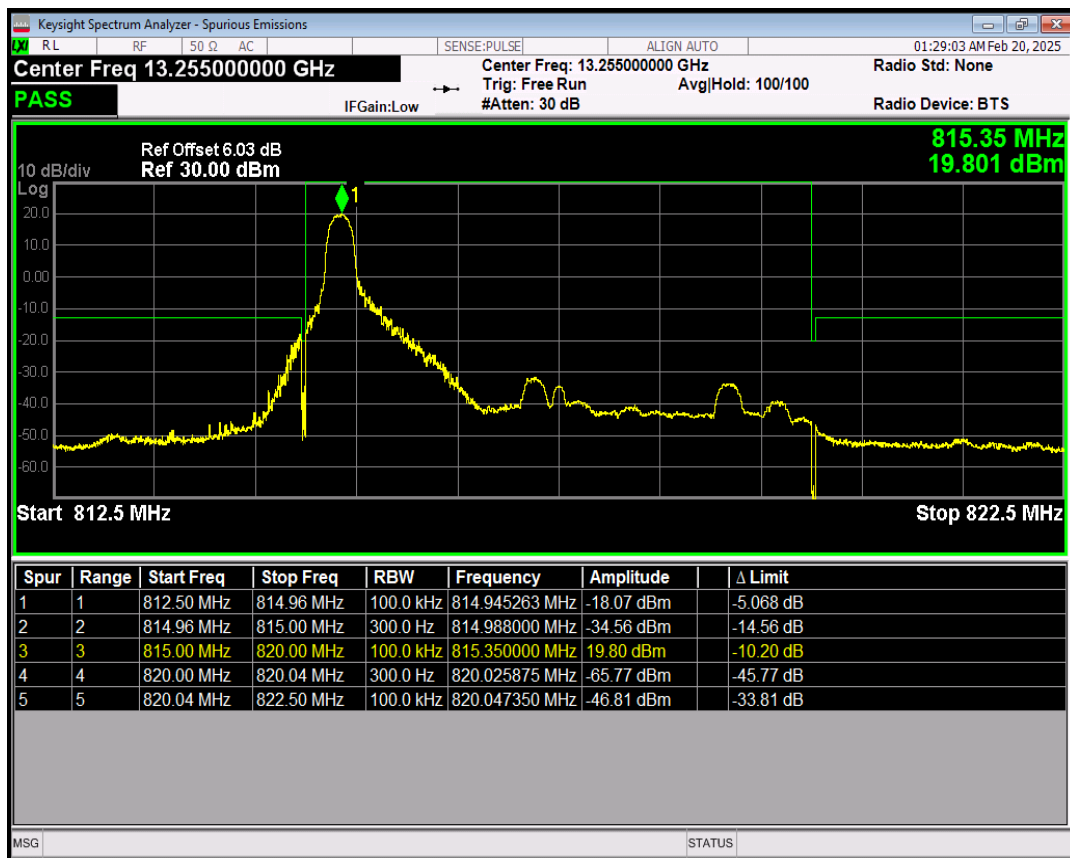
Band18 16QAM BW=5MHz Channel=23875 RB Size=1 Position=#Max
