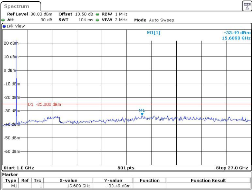
Band 41_5 MHz_Low_16QAM_RB1#0_2(1GHz-27GHz)
