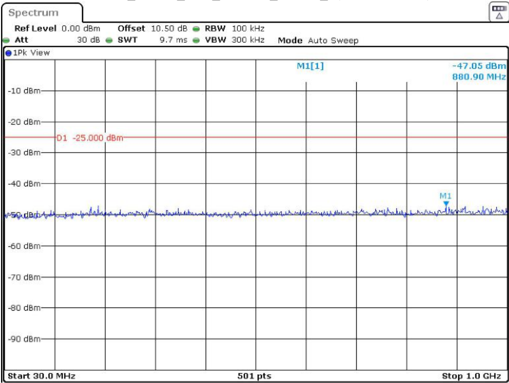
Band 41_5 MHz_Low_16QAM_RB1#0_1(30MHz-1GHz)
