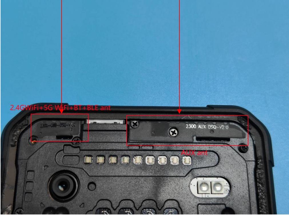
BT/Wi-Fi Ant
