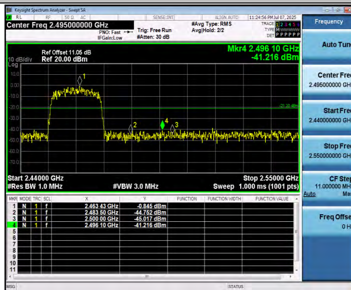
11AX20SISO_Ant2_High_2462_Peak
