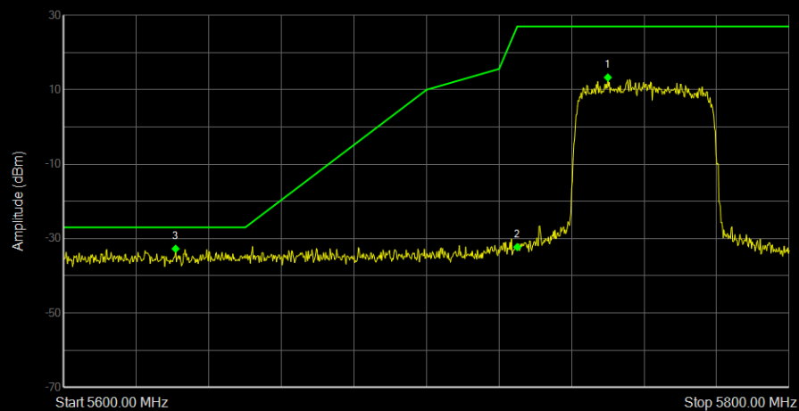
Band Edge NVNT 40M 5760MHz Low Ant 1
