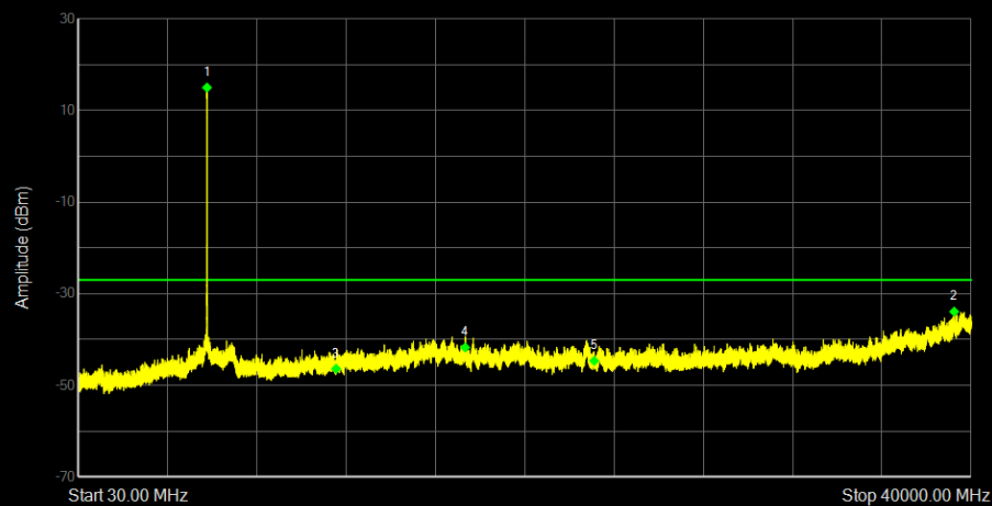
Tx. Spurious NVNT 20M 5780MHz Ant 2 Emission
