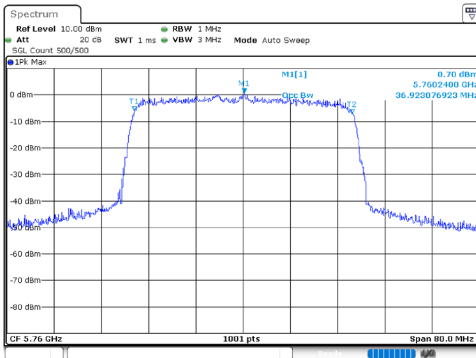
-26 dB BW NVNT 40M 5760MHz Ant 2
