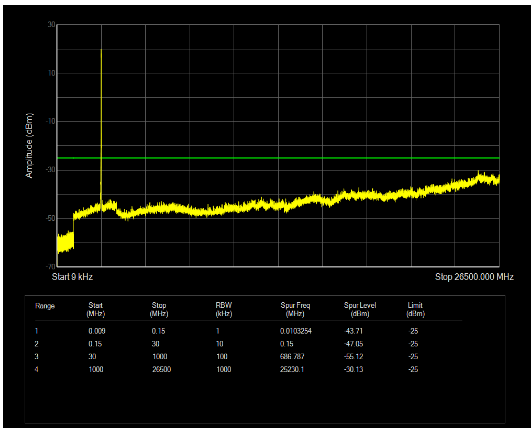
Band41(2555-2655) QAM16 BW=15MHz Channel=40315 RB Size=1 Position=#0
