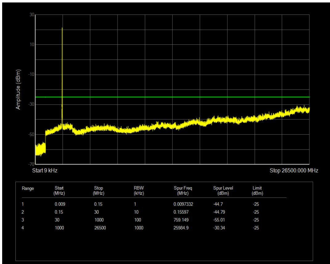
Band41(2555-2655) QAM16 BW=10MHz Channel=41190 RB Size=1 Position=#0
