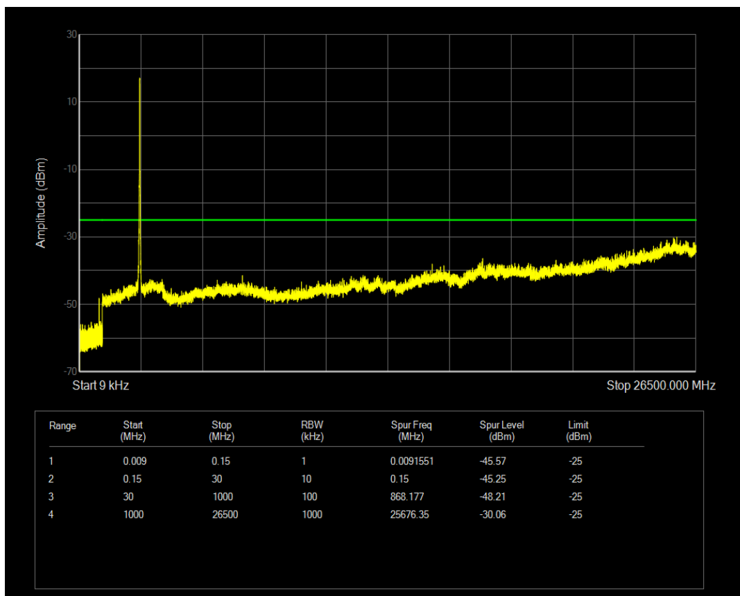
Band41(2555-2655) QAM16 BW=20MHz Channel=41140 RB Size=1 Position=#0
