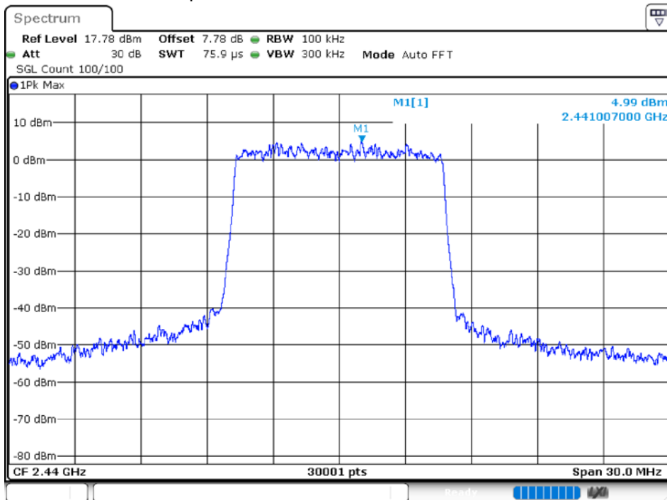
Tx. Spurious NVNT 10M 2440MHz Ant 1 Emission
