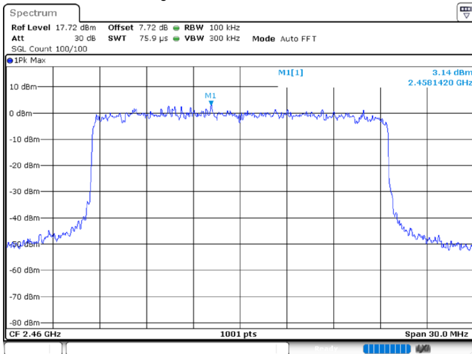
Band Edge NVNT 20M 2460MHz Ant 2 Emission
