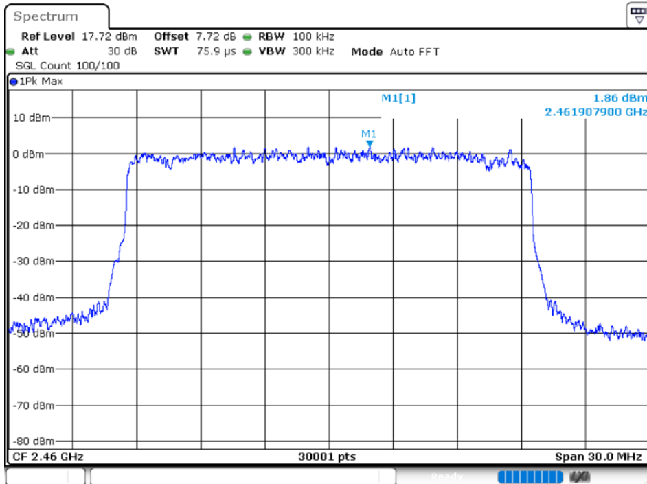
Tx. Spurious NVNT 20M 2460MHz Ant 1 Emission
