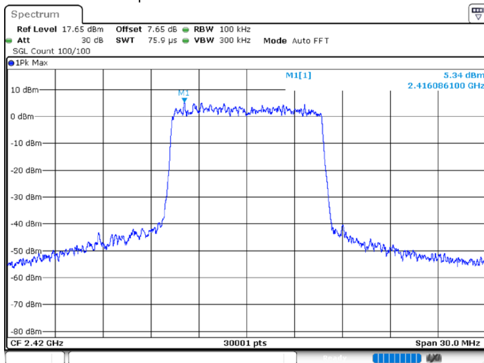
Tx. Spurious NVNT 10M 2420MHz Ant 1 Emission
