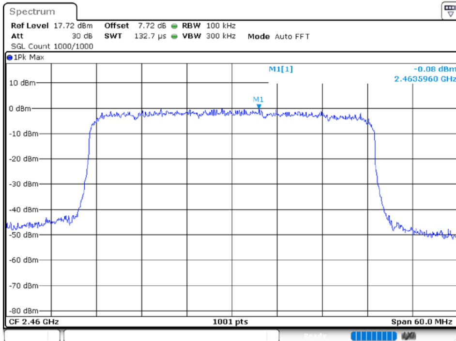
Band Edge NVNT 40M 2460MHz Ant 1 Emission
