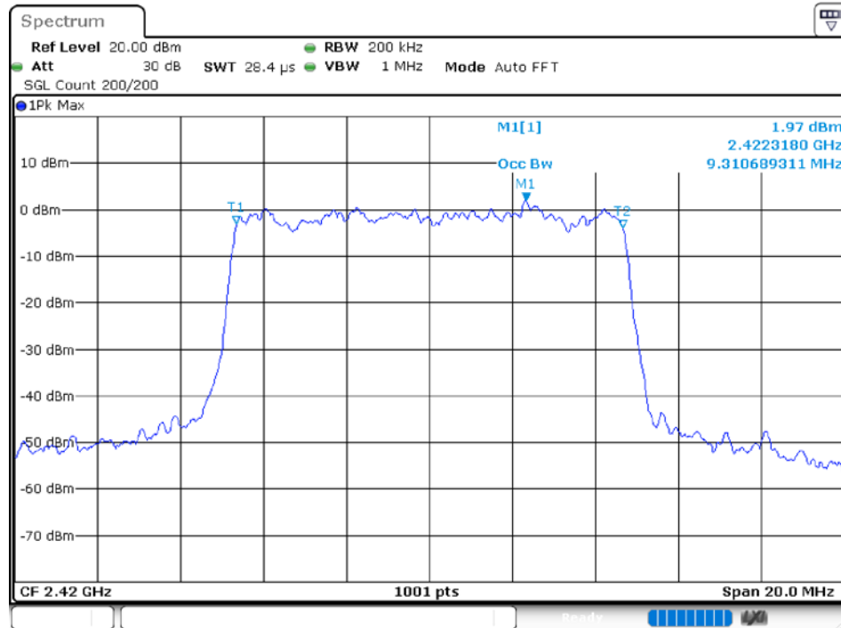
-6 dB BW NVNT 10M 2420MHz Ant 1
