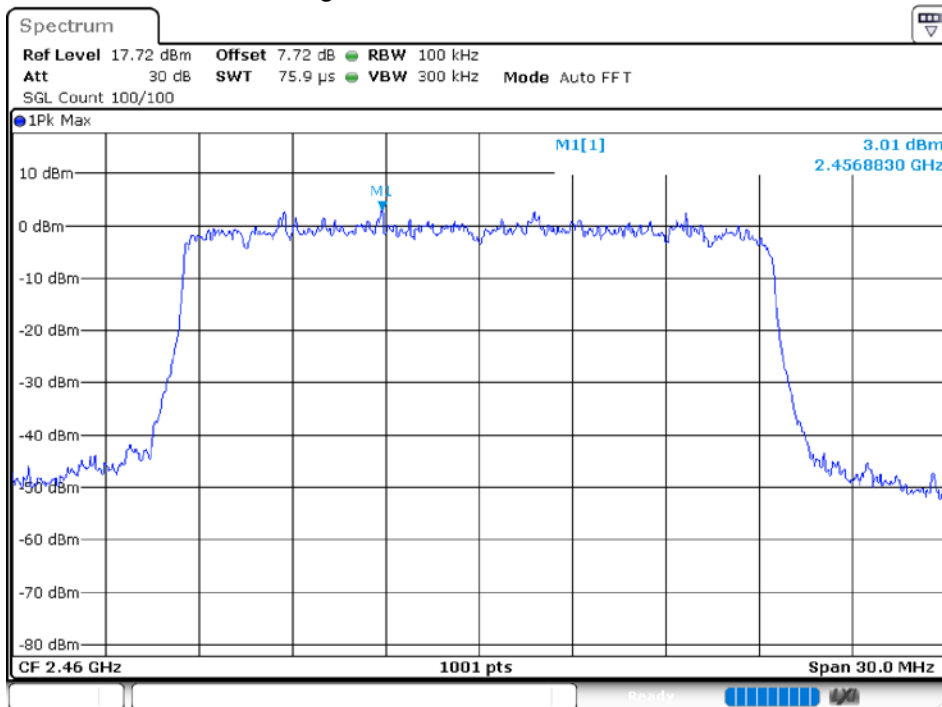
Band Edge NVNT 20M 2460MHz Ant 1 Emission
