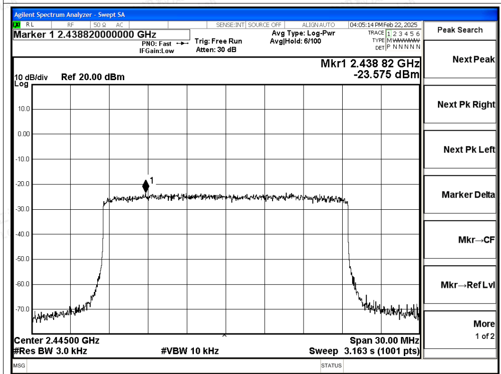
PSD NVNT 20MHz Bandwidth 2445MHz Ant1
