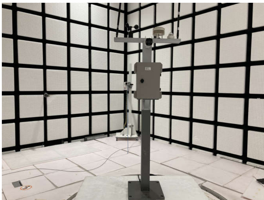
Radiated spurious emission Test Setup-2(Above 18GHz)
