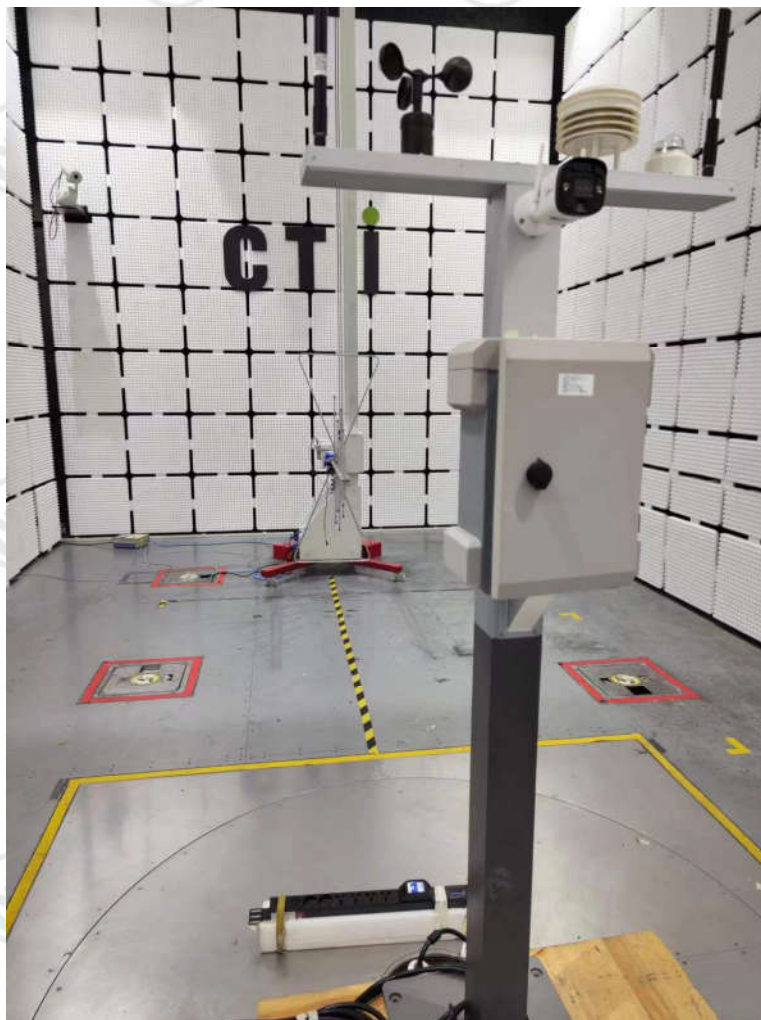
Radiated spurious emission Test Setup-1(Below 1GHz)
