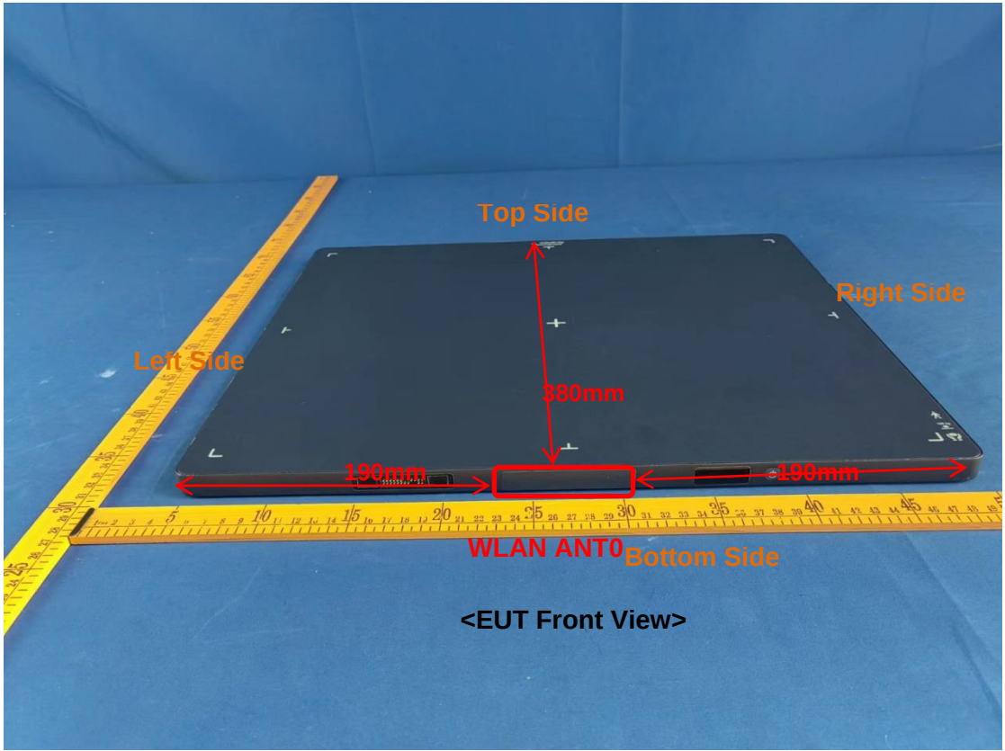
Fig 7.1 Block Diagram for EUT Antenna Position EUT Size: Long*Width =455mm*380mm
