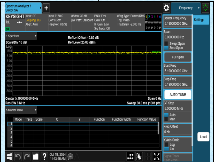
NTNV-11AC40MIMO-Ant4-5190
