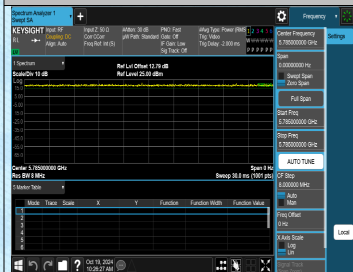
NTNV-11AC20SISO-Ant3-5785
