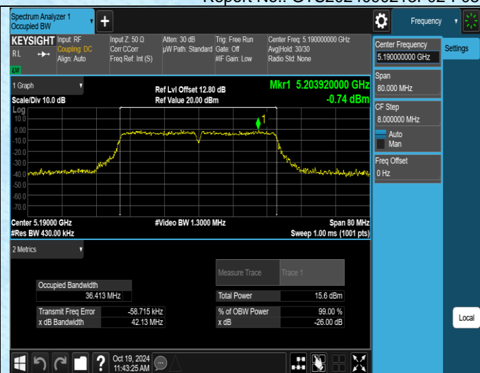
11AC40MIMO-Ant4-5190
