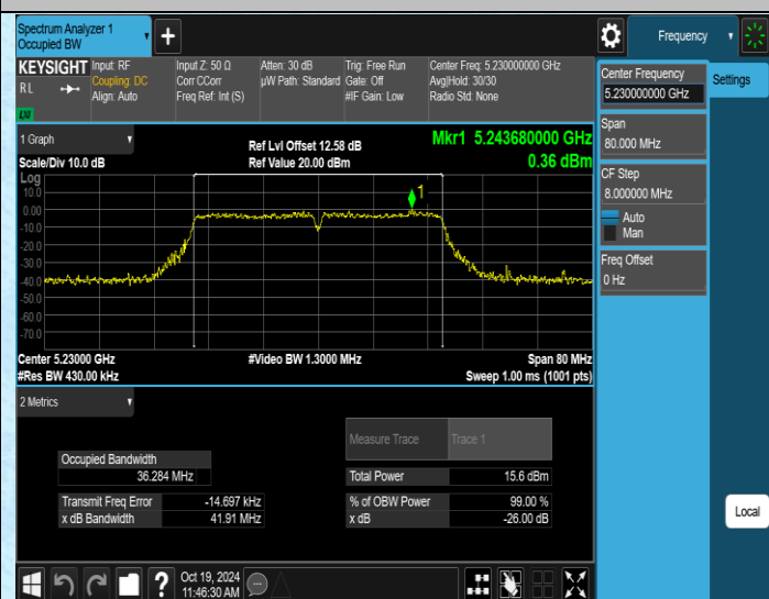
11AC40MIMO-Ant4-5230
