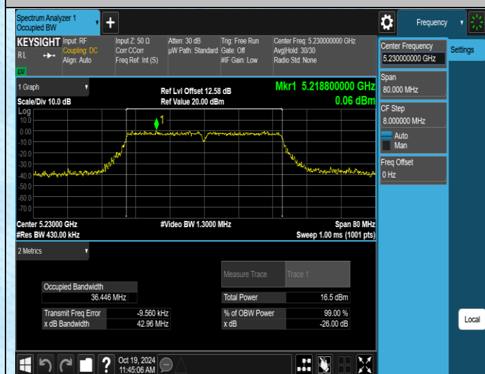
11AC40MIMO-Ant3-5230
