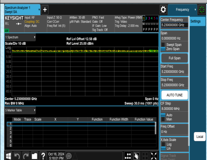
NTNV-11AC40SISO-Ant2-5230
