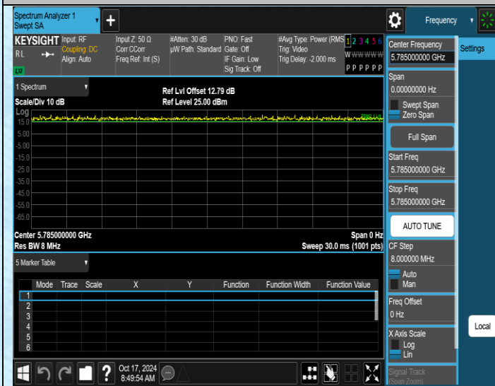
NTNV-11AC20MIMO-Ant1-5785
