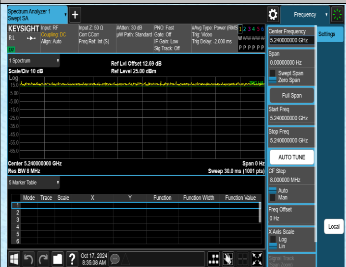
NTNV-11AC20MIMO-Ant2-5240
