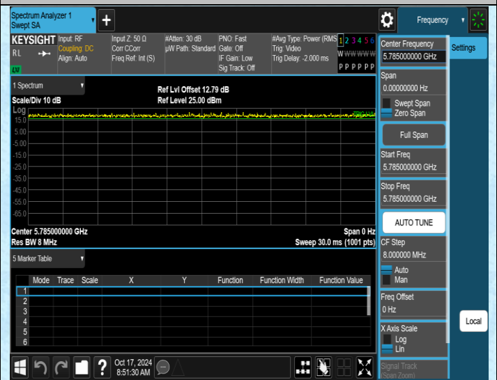
NTNV-11AC20MIMO-Ant2-5785
