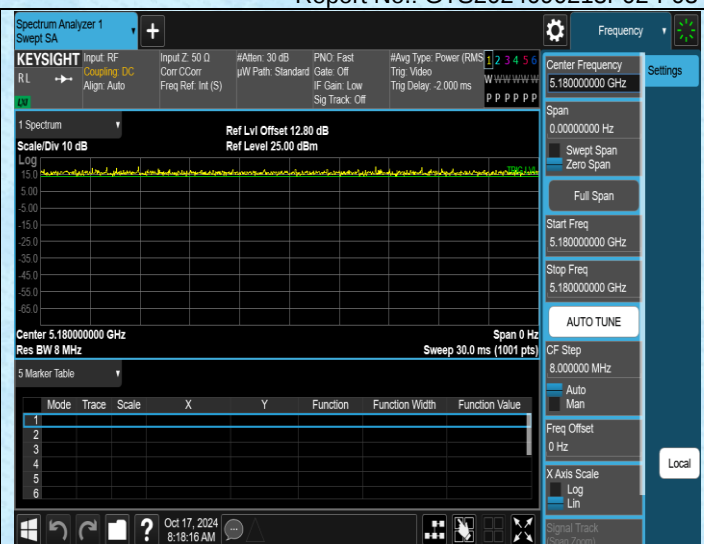
NTNV-11AC20MIMO-Ant2-5180
