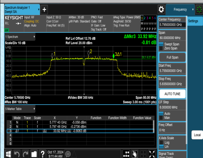
11AC40MIMO-Ant2-5795-PASS
