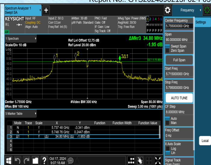
11AC40MIMO-Ant2-5755-PASS
