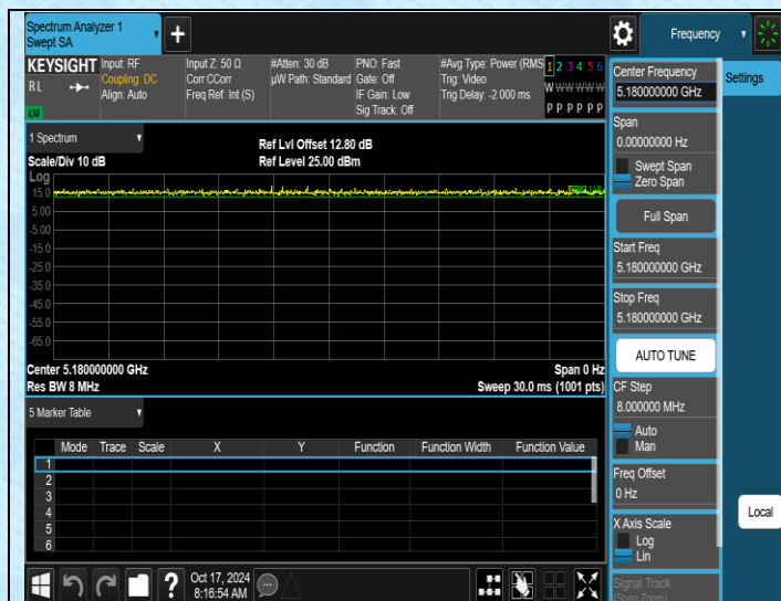
NTNV-11AC20MIMO-Ant1-5180
