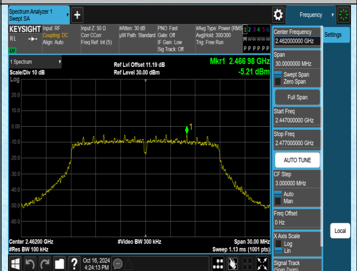
11N20MIMO-Ant2-2462-0~Reference-PASS
