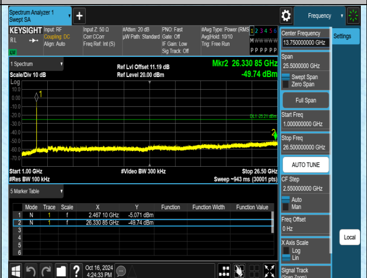
11N20MIMO-Ant2-2462-1000~26500-PASS
