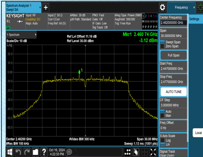
11N20MIMO-Ant1-2462-0~Reference-PASS
