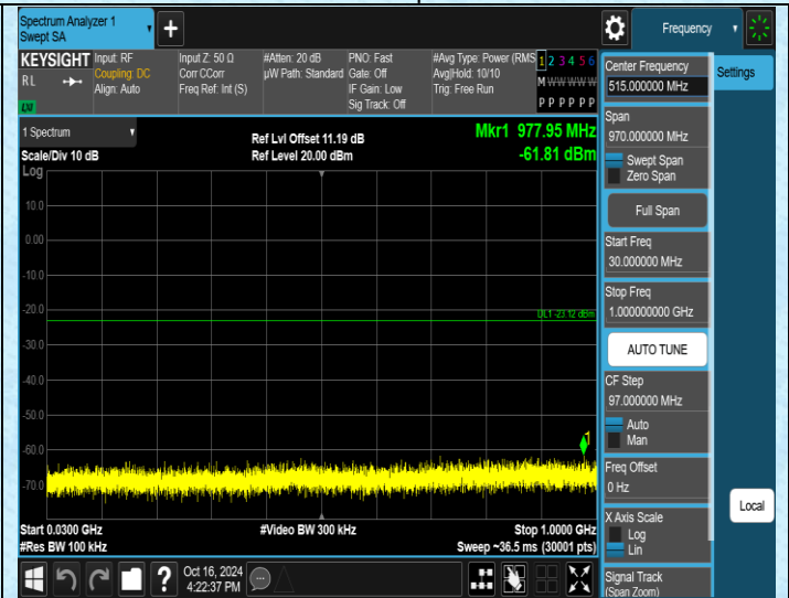
11N20MIMO-Ant1-2462-30~1000-PASS
