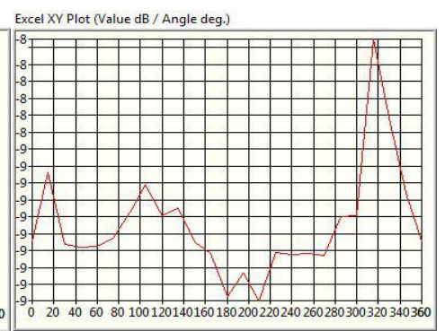
2.4GHz@Theta 0.0
