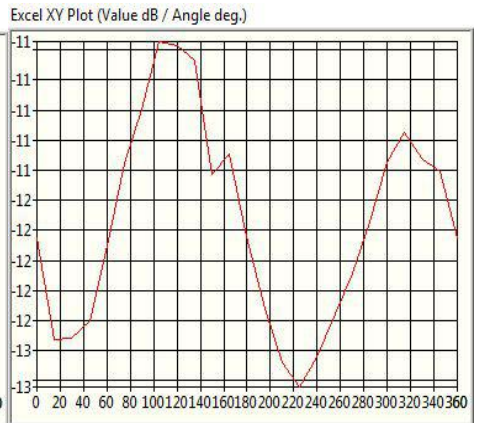
2.485GHz@Theta 0.0
