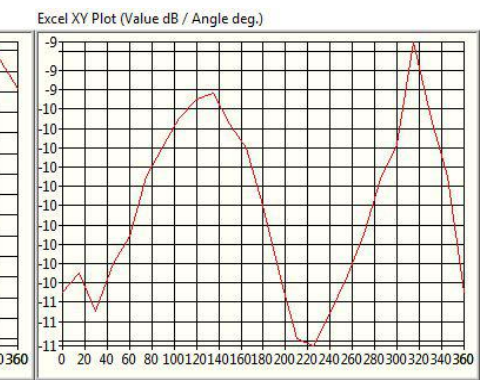
2.45GHz@Theta 0.0
