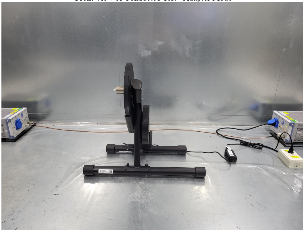
Front View of Conducted Test - Adapter Mode
