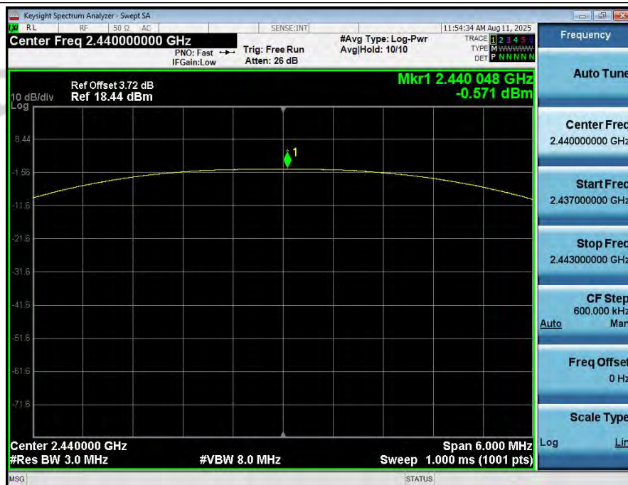
Peak_Output_Power_&_EIRP_NVNT_ANT1_1Mbps_2440
