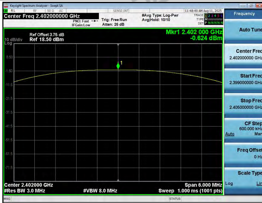
Peak_Output_Power_&_EIRP_NVNT_ANT1_1Mbps_2402
