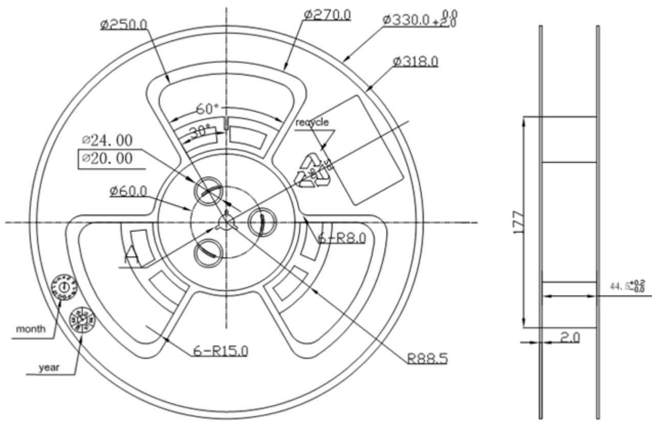
Figure 35: Reel detail
