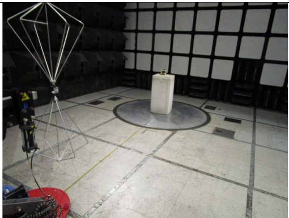
Below 1 GHz Radiated Emissions
