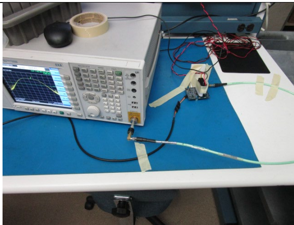
Conducted Setup
