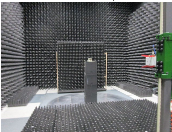
Above 1 GHz Radiated Emissions
